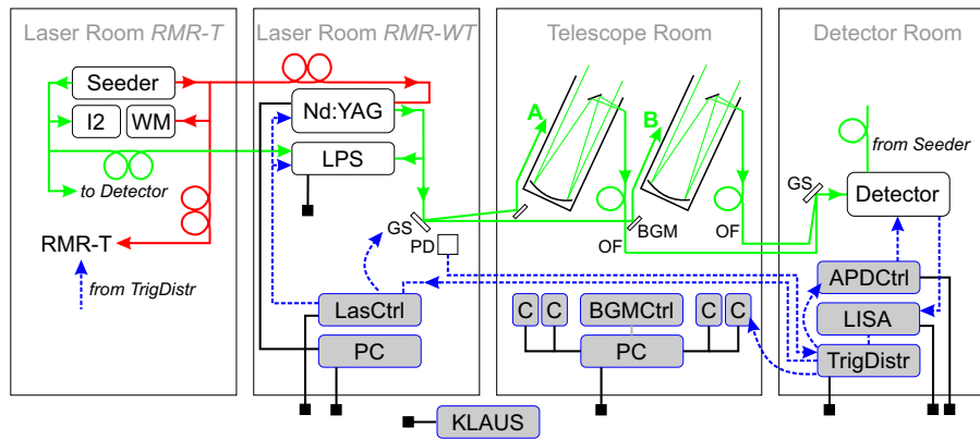
Figure 1. Schematic of the new wind lidar system 'RMR3RMR-WT' at K hlungsborn. I2: Iodine cell, WM: wavemeter, LPS Laser Pulse Spectrometer, GS: galvanometer scanner, PD: photodiode, LasCtrl-3LasCtrl: Laser Controller RMR3RMR-WT, BGM: Beam Guiding Mirror, OF: optical fibre, C: camera, BGMCtrl: BGM Controller, APDCtrl: Avalanche Photo Diode Controller, LISA: Lidar Singleshot Acquisition, TrigDistr: Trigger Distributor, KLAUS: K hlungsborn Lidar Automation System. A, B denote outgoing beams and telescopes. Green/red: light path of 532/1064 nm light; black: Ethernet/TCPIP connections, grey: USB connection; blue dashed: (coax) data cable. Only the most relevant parts and connections are displayed.
