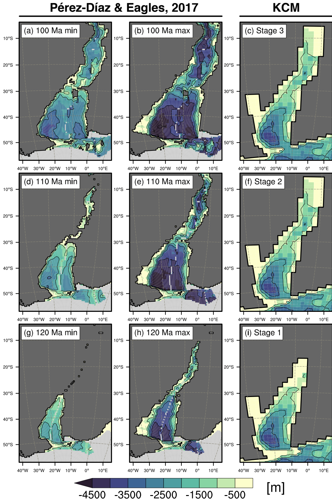
Figure S1. Comparison of available reconstructions for the Early Cretaceous South Atlantic 1 with the model bathymetries used in this study. Only the minimum and maximum reported water depth is shown for each stage, and the data have been re-gridded to a horizontal grid of 0.5^\circ \times 0.5^\circ horizontal grid. Contour line interval is 1000 m.
