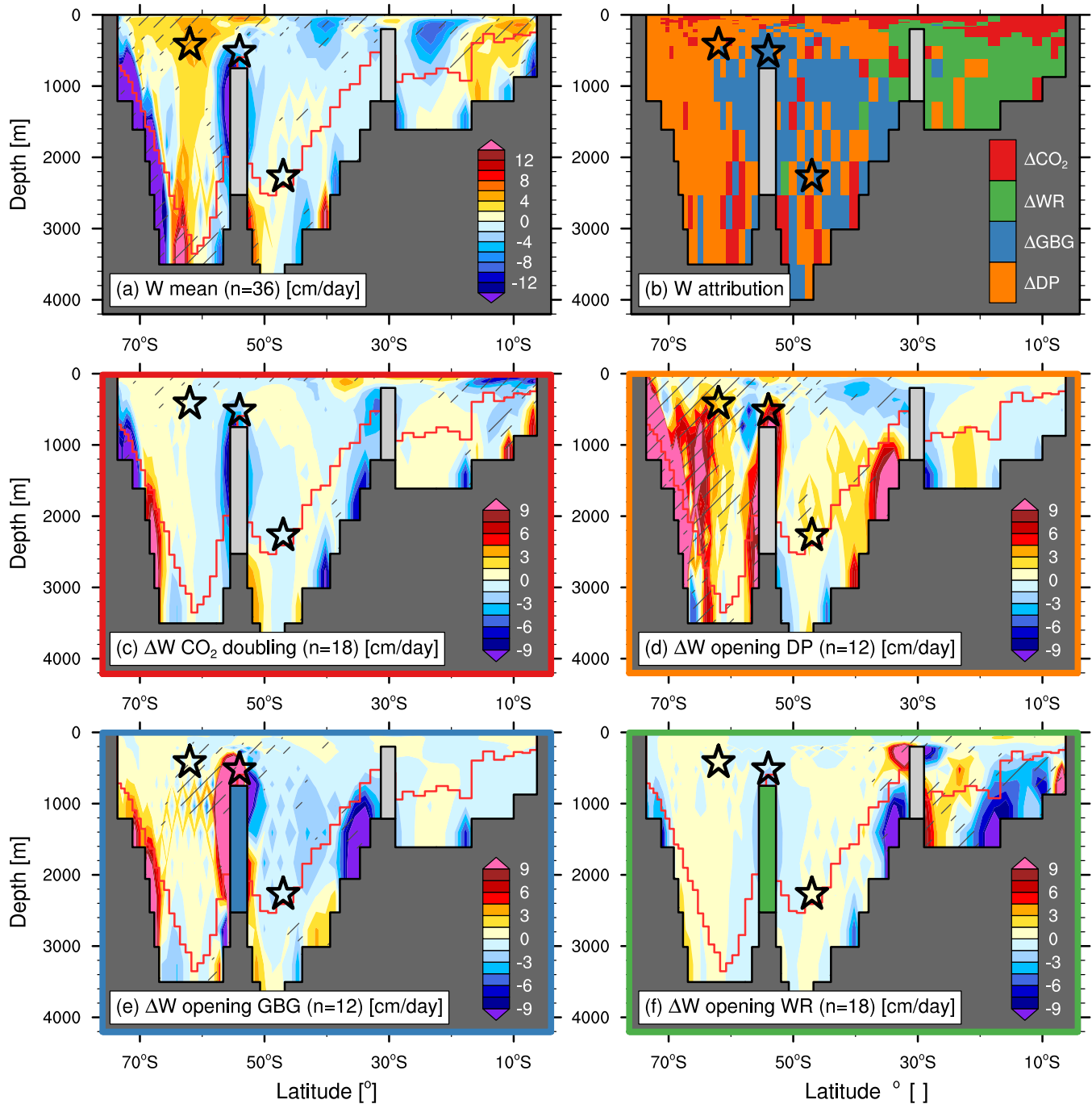
Figure S5. Vertical ocean circulation. Panels show the (a) ensemble mean, (b) the respective boundary condition resulting in the largest mean change, and (c-f) the mean change associated with the individual processes defined in Section 2.3 of the main text. Fields are smoothed with a nine-point average for figure clarity and are shown in cm/day. Positive (negative) values represent upward (downward) flow. Contour range only shows a subset of the data to focus on changes in the South Atlantic. Hatching indicates region where all ensemble members agree on the sign of the shown field. Black (red) lines indicate maximum (average) water depth at the respective latitude.
