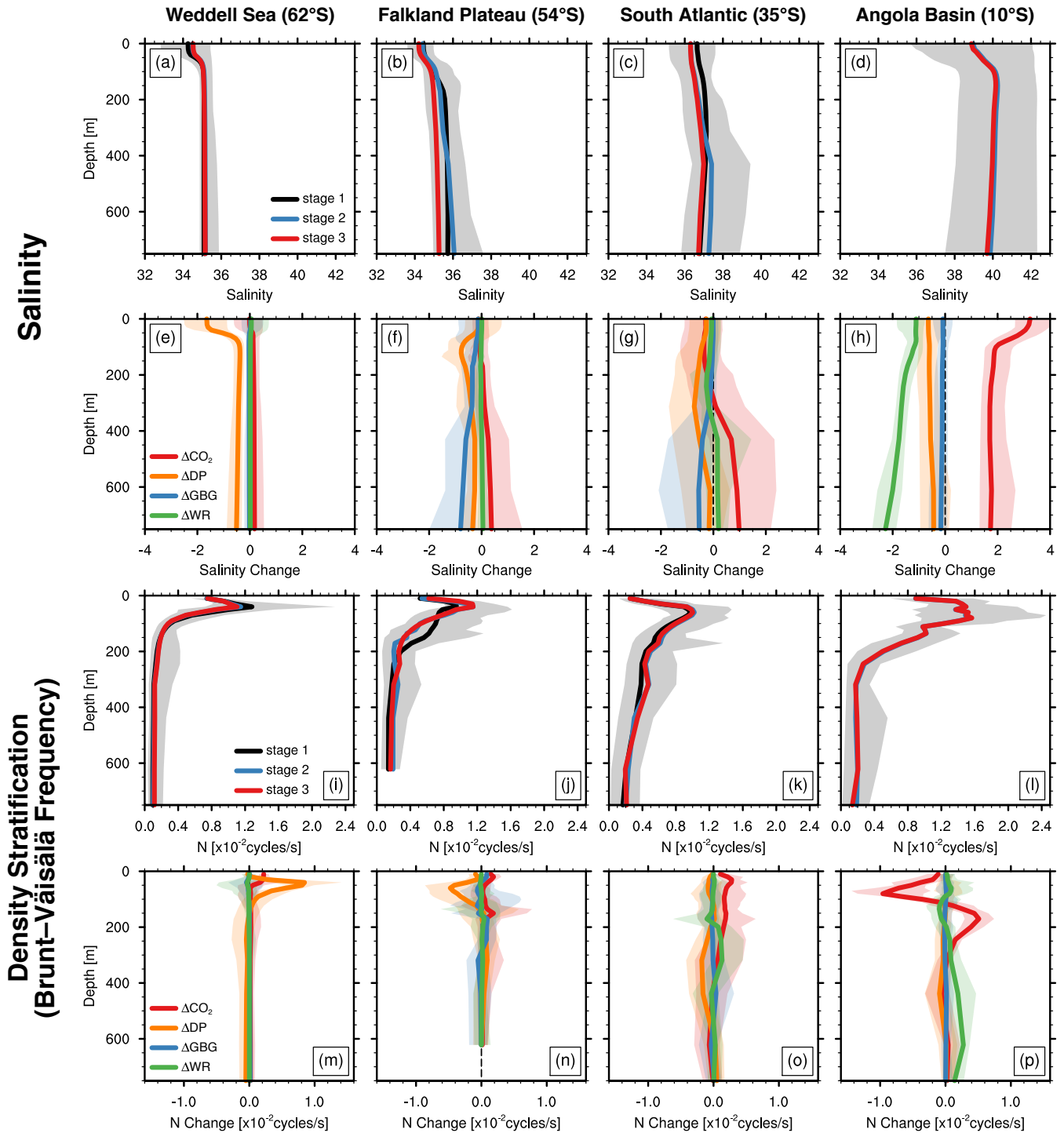
Figure S3. Simulated ocean salinity profiles and density stratification across the Southern Ocean and South Atlantic. Density stratification is expressed in terms of the Brunt–Väisälä frequency (buoyancy frequency) defined as: N = \sqrt{-\frac{g}{\rho_0} \frac{\delta \rho(z)}{\delta z}} , where \rho is the potential density. Solid lines represent regional averages (areas shown in Fig. 1g of the main text), while shading indicates the simulated maximum and minimum grid point values of the respective area across all simulations. The processes analysed are defined in Section 2.3 of the main text. The area used for averaging across the Falkland Plateau Basin in panels (b),(f),(j) and (n) moves westward for each consecutive model stage to allow comparison with the proxy record. N is calculated on the mid depths of the model and, therefore, only defined to 620 m on the Falkland Plateau. All simulations have a global mean salinity of 35.
