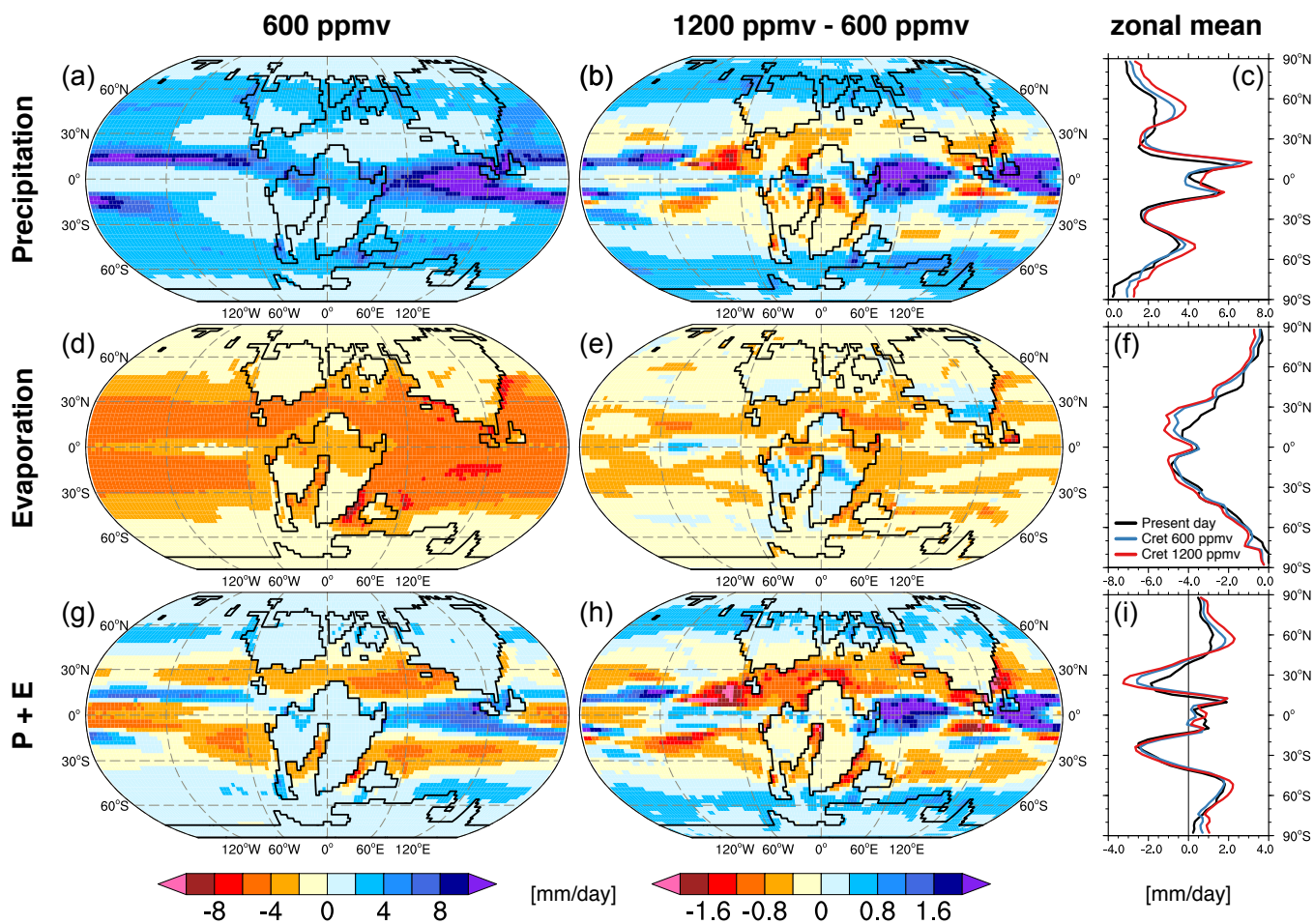
Figure S6. CO 2 sensitivity of the global hydrological cycle. Panels show ensemble mean (n=18) precipitation, evaporation and the sum of both for (left) 600 ppmv CO 2 , (middle) the respective change for doubling CO 2 and (right) the zonal mean values for the 600 and 1200 ppmv ensembles as well as for the same model configuration under present-day boundary conditions. All values are given in mm/day.
