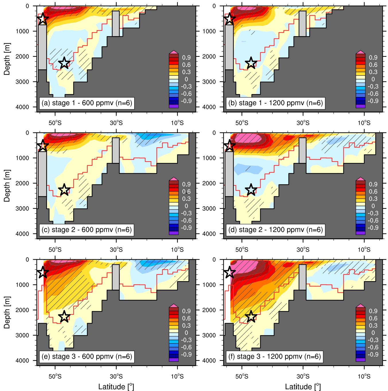
Figure S7. South Atlantic meridional overturning circulation (MOC). Panels show the respective ensemble means for stages 1 to 3 integrated at (left) 600 ppmv and (right) 1200 ppmv. Values are in Sv with 1 \text{ Sv} = 10^6 \text{ m}^3/\text{s} . Positive (negative) values represent clockwise (counterclockwise) circulation. Hatching indicates region where all 6 ensemble members agree on the sign of the MOC. Black (red) lines indicate maximum (average) water depth at the respective latitude.
