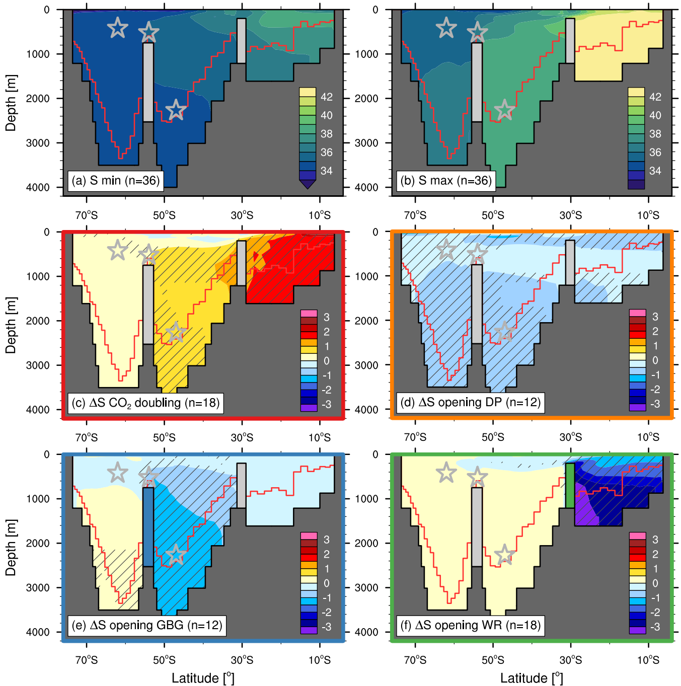
Figure S2. Zonal mean salinity sections for the South Atlantic and Southern Ocean. Values are averaged between 30°W and 10°W at the Falkland Plateau and between 30°W and 0° elsewhere. Black (red) lines indicate maximum (average) water depth at the respective latitude. Panels show the (a) minimum and (b) maximum simulated value across all 36 ensemble members and (c-e) the mean change associated with the individual processes defined in Section 2.3 of the main text. Hatching indicates areas where all the respective 12 or 18 model responses agree on the sign of the change.
