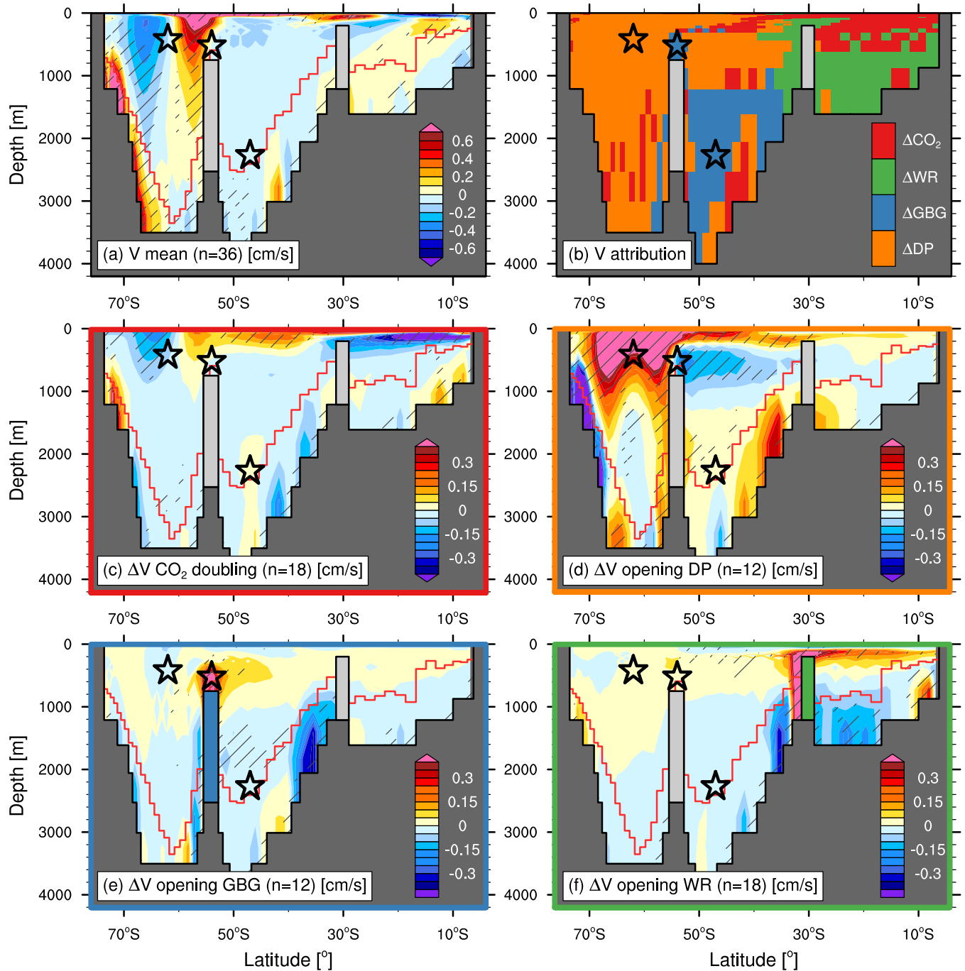
Figure S4. Meridional ocean circulation. Panels show the (a) ensemble mean, (b) the respective boundary condition resulting in the largest mean change, and (c-f) the mean change associated with the individual processes defined in Section 2.3 of the main text. Fields are smoothed with a nine-point average for figure clarity and are shown in cm/s. Positive (negative) values represent northward (southward) flow. Contour range only shows a subset of the data to focus on changes in the South Atlantic. Hatching indicates region where all ensemble members agree on the sign of the shown field. Black (red) lines indicate maximum (average) water depth at the respective latitude.
