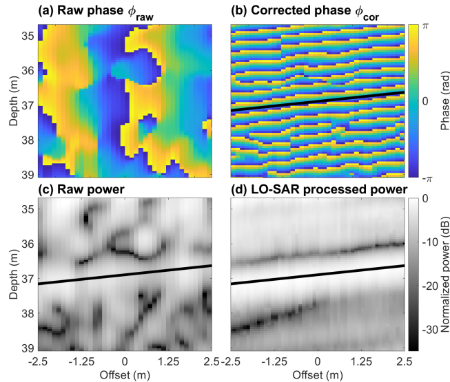
Figure 3. An exemplary segment of the pRES profile over one synthetic aperture length. Phase signal before (a) and after (b) correcting it with a reference signal. Power before (c) and after (d) LO-SAR processing. The slope of the central reflection is indicated by a black line and obtained in (b) by fitting to a coherent section of the reference corrected phase.
