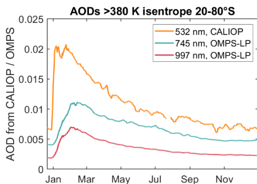
Figure 7 | Wildfire impact on stratospheric AODs at three wavelengths in the southern extratropics from CALIOP and OMPS-LP. The stratospheric column above the 380 K isentropes at 20-80°S.
