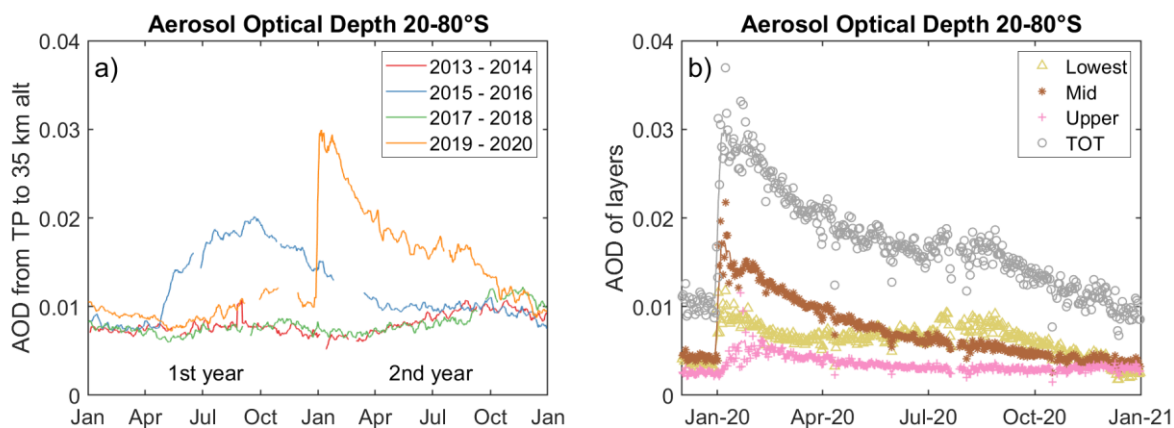
Figure 6 | Wildfire impact on the stratospheric aerosol load in the southern extratropics. a) The aerosol optical depth (AOD) from CALIOP in 2013-2020 divided into two-year-steps, illustrating the impact of the Australian wildfire in 2019-2020, together with that from the Calbuco eruption in 2015-2016, and background levels 2013-2014 and 2017-2018. b) the stratospheric AOD from CALIOP during Dec 2019 – Jul 2020 separated into the three layers used in Figure 2. Lines mark 8-day smoothed AOD data, and symbols are daily means of the LMS (yellow), shallow (brown) and upper (pink) BD-branches, and the total stratospheric AOD (grey).
