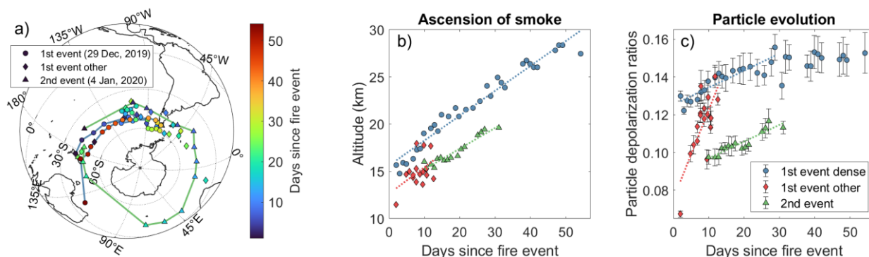
525 Figure 8 | The smoke transport and chemical evolution in the stratosphere. a) Geographical transport of the smoke from the two injection events. b) Ascension of the smoke clouds, and c) temporal evolution of the particle depolarization ratios for the two injection events. All data taken on individual smoke clouds in the stratosphere. Circles mark data taken in the dense isolated cloud from the 1 st event fires, diamonds are other data from the 1 st fire, and triangles mark smoke data from the 2 nd event fires.
