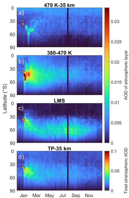
Figure 5 | Latitude and time distribution of the stratospheric aerosol load. Aerosol optical depth (AOD) in three stratospheric layers and in all layers combined. The upper (a) and mid (b) layers are the deep and shallow branches of Brewer-Dobson circulation, and the lowest layer (c) is the lowermost stratosphere.
