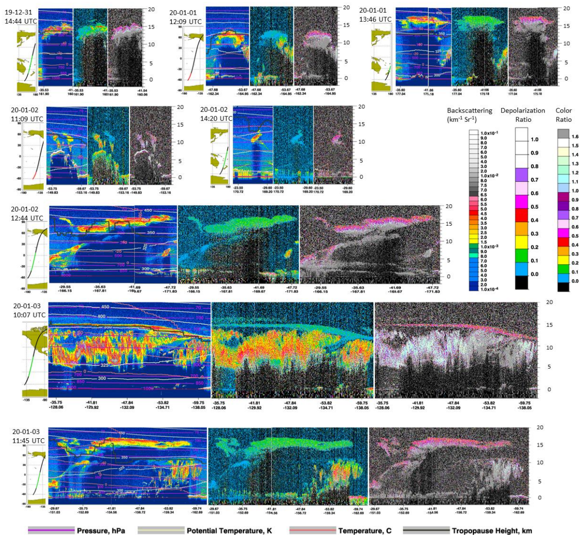
490 Figure 2. Four days CALIOP curtains from early overpasses of the region affected by the 1 st fire event on 2019-12-29. The day of the fire did not show elevated smoke levels from the single CALIOP overpass of the region, and the day after (2019-12-30) no measurements were taken in the fire region due to malfunction. Left panels show attenuated backscattering, mid panels, the volume depolarization ratios, and right panels the attenuated color ratios. Strong attenuation of the lidar beam is indicated by the dark blue colors below smoke layer, as well as through the higher color ratios at the bottom of the smoke layers.
