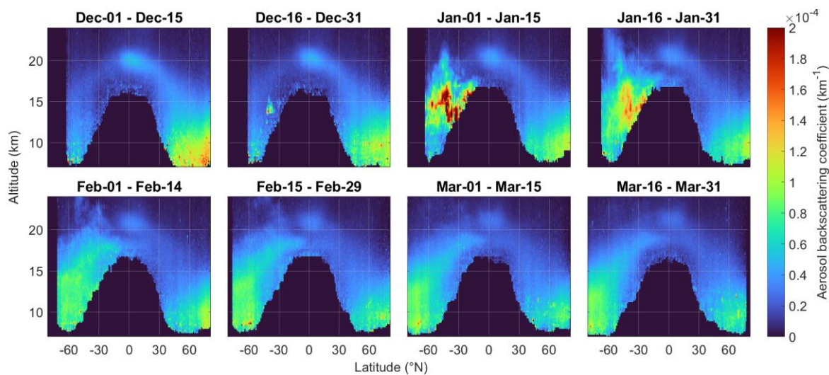
Figure 4 | Latitudinal and vertical distribution of smoke in Dec 2019 – Mar 2020. CALIOP zonal mean aerosol backscattering coefficients during the first three months after, and one month preceding, the first stratospheric injection. This parameter can be viewed as an optical version of aerosol concentration.
