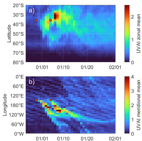
540 Figure 11. | Evolution of the UV aerosol index (UVAI) during the first weeks after the fire events for a) zonal means and b) meridional means. The locations and dates of the events are marked by orange dots. The lower UVAI range in a) stem from the method of area weighting data.
