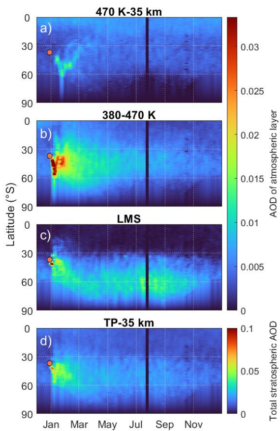
560 Figure 4 | Latitude and time distribution of the stratospheric aerosol load. Aerosol optical depth (AOD) in three stratospheric layers and in all layers combined. The upper (a) and mid (b) layers are the deep and shallow branches of Brewer-Dobson circulation, and the lowest layer (c) is the lowermost stratosphere. The orange dot shows the approximate latitude and the time of the 1 st fire.
