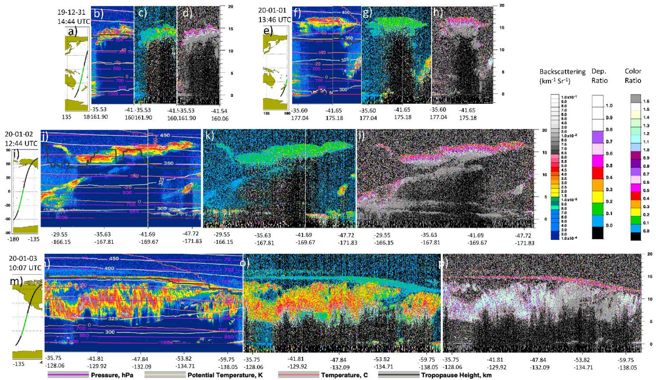
Figure 1. CALIOP curtains from early overpasses of the region affected by the 1 st fire event that started on 2019-12-29. Left panels show attenuated backscattering, mid panels, the volume depolarization ratios, and right panels the attenuated color ratios. Strong attenuation of the lidar beam is indicated by the dark blue colors below smoke layer, as well as through the higher color ratios at the bottom of the smoke layers. Meteorological parameters are marked with lines; pressure levels (purple), potential temperatures (white), temperatures (orange), and tropopause heights (grey). See the supplementary for further curtain plots.
