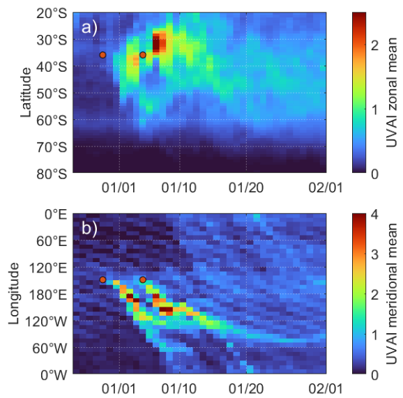
595 Figure 10. | Evolution of the UV aerosol index (UVAI) during the first weeks after the fire events for a) zonal means and b) meridional means. The locations and dates of the events are marked by orange dots. The lower UVAI range in a) stem from the method of area weighting data.
