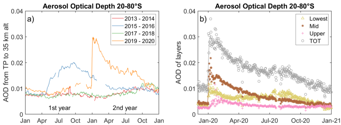
565 Figure 5 | Wildfire impact on the stratospheric aerosol load in the southern extratropics. a) The aerosol optical depth (AOD) from CALIOP in 2013-2020 divided into two-year-steps, illustrating the impact of the Australian wildfire in 2019-2020, together with that from the Calbuco eruption in 2015-2016, and background levels 2013-2014 and 2017-2018. b) the stratospheric AOD from CALIOP during Dec 2019 – Jul 2020 separated into the three layers used in Figure 4. Lines mark 8-day smoothed AOD data, and symbols are daily means of the LMS (yellow), shallow (brown) and upper (pink) BD-branches, and the total stratospheric AOD (grey).
