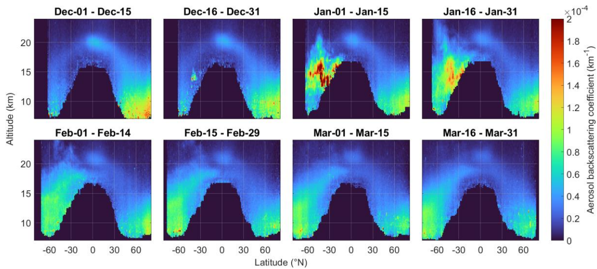
555 Figure 3 | Latitudinal and vertical distribution of smoke in Dec 2019 – Mar 2020. CALIOP zonal mean aerosol backscattering coefficients during the first three months after, and one month preceding, the first stratospheric injection. This parameter can be viewed as an optical version of aerosol concentration.
