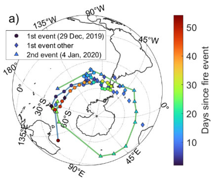
Figure 7 | The smoke transport and chemical-smoke particle evolution in the stratosphere. a) Geographical transport of the smoke from the two injection events. b) Ascension of the smoke clouds, and c) temporal evolution of the particle depolarization ratios for the two injection events. All data taken on individual smoke clouds in the stratosphere. Circles mark data taken in the dense isolated cloud from the 1 st event fires, diamonds are other data from the 1 st fire, and triangles mark smoke data from the 2 nd event fires.
