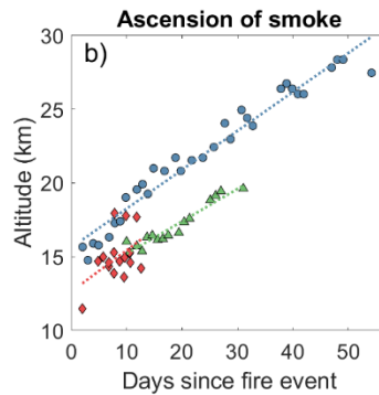
Figure 7 | The smoke transport and chemical-smoke particle evolution in the stratosphere. a) Geographical transport of the smoke from the two injection events. b) Ascension of the smoke clouds, and c) temporal evolution of the particle depolarization ratios for the two injection events. All data taken on individual smoke clouds in the stratosphere. Circles mark data taken in the dense isolated cloud from the 1 st event fires, diamonds are other data from the 1 st fire, and triangles mark smoke data from the 2 nd event fires.
