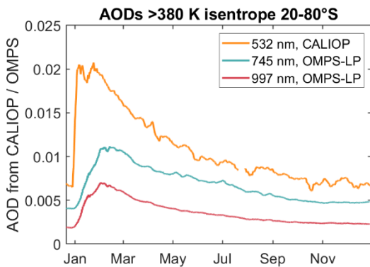
570 Figure 6 | Wildfire impact on stratospheric AODs at three wavelengths in the southern extratropics from CALIOP and OMPS-LP. The stratospheric column above the 380 K isentropes at 20-80°S.
