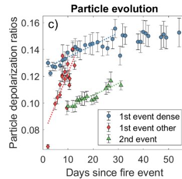
Figure 7 | The smoke transport and chemical-smoke particle evolution in the stratosphere. a) Geographical transport of the smoke from the two injection events. b) Ascension of the smoke clouds, and c) temporal evolution of the particle depolarization ratios for the two injection events. All data taken on individual smoke clouds in the stratosphere. Circles mark data taken in the dense isolated cloud from the 1 st event fires, diamonds are other data from the 1 st fire, and triangles mark smoke data from the 2 nd event fires.
