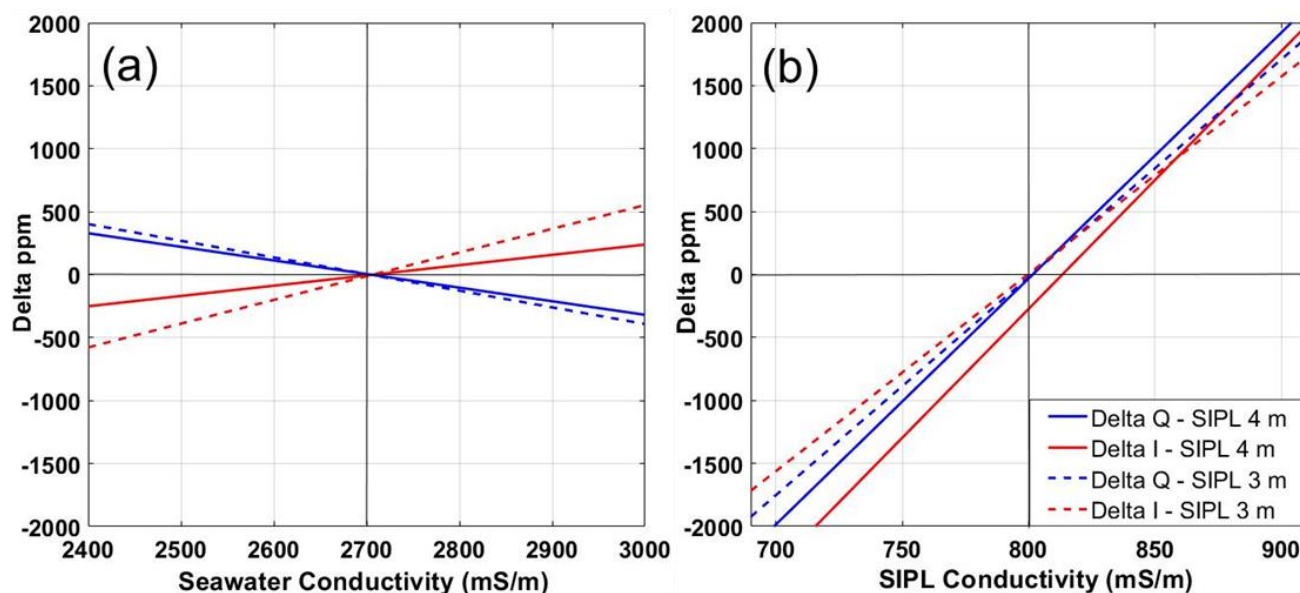
Figure 3. Forward modelled I and Q for a 3-layer case consisting of constant consolidated ice thickness of 2.7 m and SIPL thicknesses of 3 m or 4 m, for (a) a range of seawater conductivities from 2400 to 3000 \text{ mS m}^{-1} and a fixed bulk SIPL conductivity of 800 \text{ mS m}^{-1} , and (b) a range of SIPL bulk conductivity values from 700 to 900 \text{ mS m}^{-1} and a fixed bulk seawater conductivity of 2700 \text{ mS m}^{-1} . Y-axes show the magnitude of change in delta ppm with respect to the (a) seawater ( 2700 \text{ mS m}^{-1} ) and (b) SIPL ( 800 \text{ mS m}^{-1} ) conductivities used in the base forward model for the Spring EM time-series.
