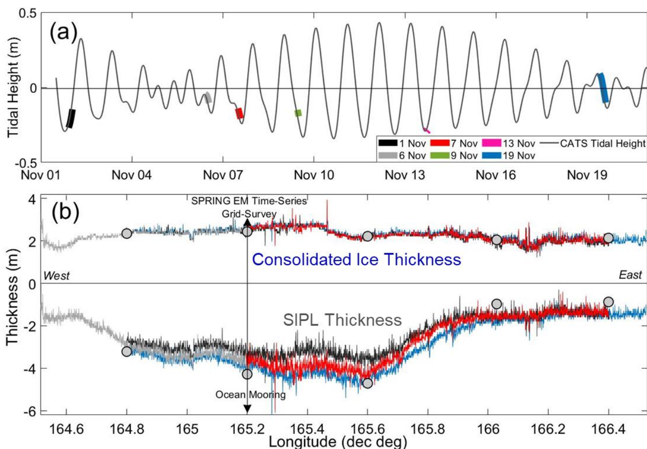
Figure 7. Temporal variability in SIPL thickness on the repeated west-east transect (refer to Fig. 1 for location) of EM consolidated ice and SIPL across McMurdo Sound with full surveys carried out on the 1 and 19, and partial surveys on the 6, 7, 9, and 13 November (EM surveys on the 9 and 13 are not shown in (b) for clarity). The times of the repeated transects are colour-coded and displayed on the tidal height curve in (a). Drill hole measurements (circles) carried out along the transect between 3-19 November 2018 are also shown. The Spring EM time-series site, and grid-survey were located at a drill site on the transect at 165.2° E and the oceanographic mooring was deployed 500 m to the north.
