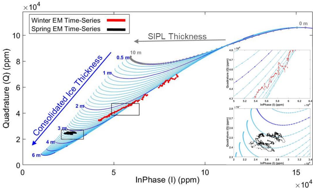
210 Figure 2. Forward model curves of quadrature ( Q ) versus in-phase ( I ) for consolidated ice, bulk SIPL, and seawater conductivities of 0, 900, and 2700 \text{mS m}^{-1} , respectively. Field measured Q and I (calibrated) data from the Winter (red) and Spring (black) EM time-series are overlaid to illustrate their location in the ( Q -vs- I ) domain. Note that the Spring EM time-series data plotted in a similar region of the 800 \text{mS m}^{-1} SIPL bulk conductivity model. The curves illustrate thicknesses of consolidated ice increasing from 0.5-6 m (from top to bottom) and SIPL increasing from 0-10 m along each individual curve (from right to left) shown as grey circles on the 0.5 m consolidated ice thickness curve, and in the insets 215 as dots on curves. Insets show magnifications of the Winter and Spring EM time-series measurements as discussed in sect. 3.1. The model is shown here at 0.10 m resolution for both consolidated ice and SIPL thickness.
