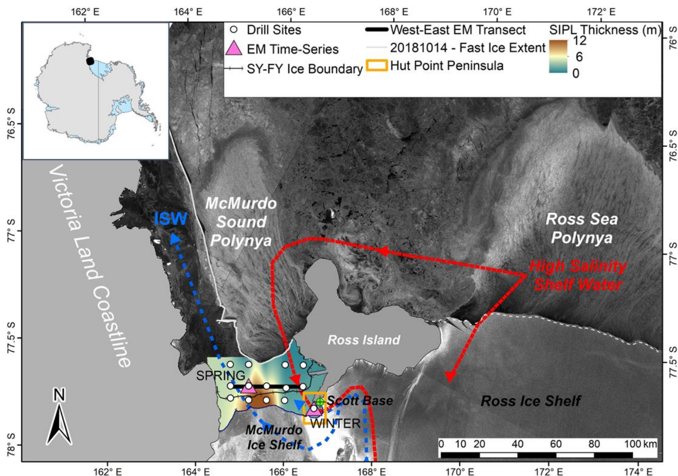
Figure 1. McMurdo Sound, western Ross Sea, Antarctica (inset map) with dashed lines illustrating the circulation of HSSW (red) and ISW (blue). The boundary between second year (SY) and first year (FY) fast ice present in the study region in 2018 is shown with the locations of the Winter and Spring EM time-series sites (pink triangles) and the Electronic Weather Station (EWS) at Scott Base. SIPL thickness distribution was spline interpolated from drill hole measurements made at 14 drill sites (circles) in November 2018, along with repeated west-east EM transects (black line) across McMurdo Sound. At the Spring site, we additionally carried out repeated 200 m x 200 m grid-surveys and collected oceanographic data at a mooring deployed (500 m to the north) in November 2018 (satellite image: Sentinel-1 SAR - 2 October 2018).
