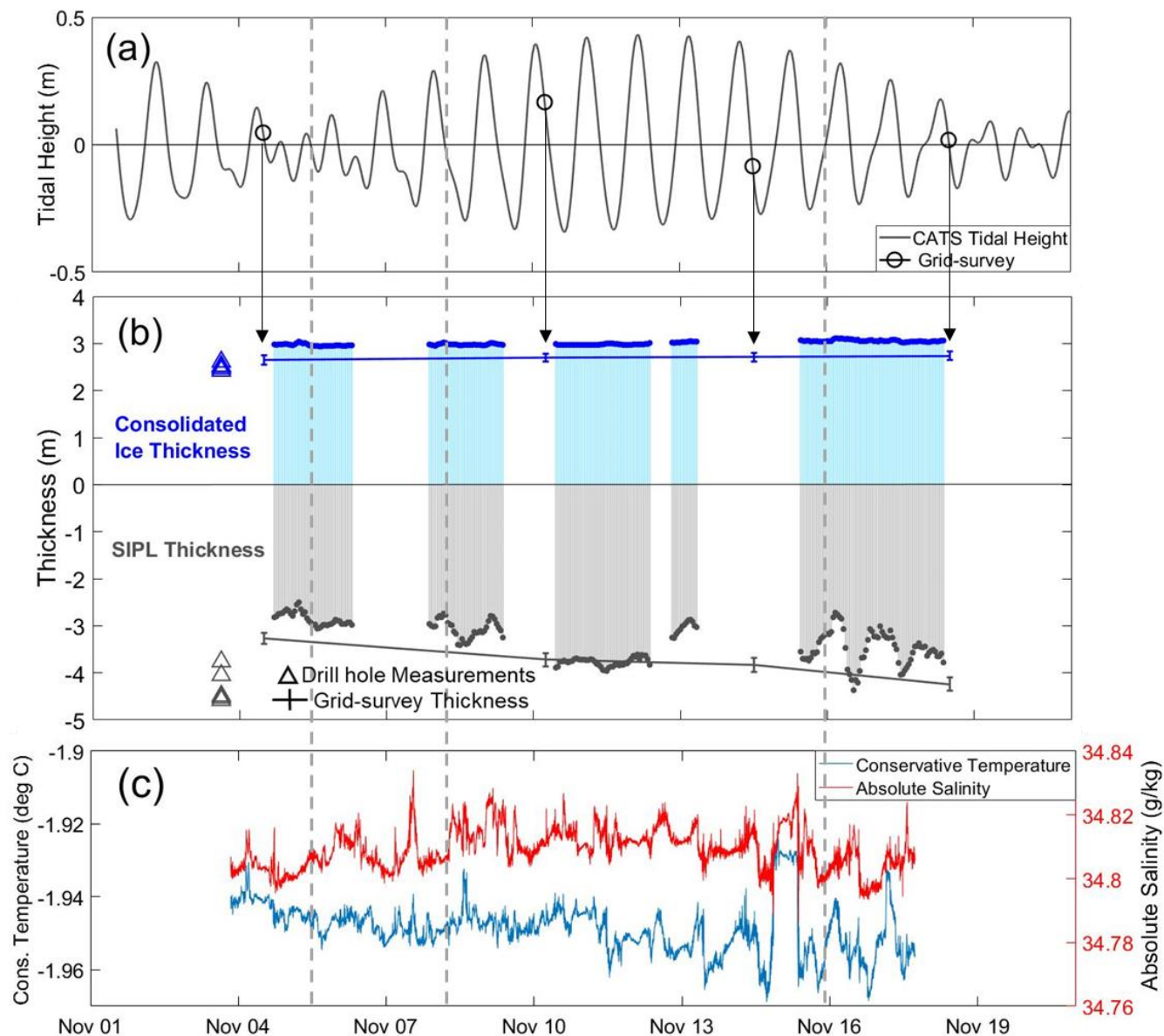
345 Figure 5. (a) CATS tidal height with the times of the repeat grid-surveys (circles) shown in (b) as lines of mean EM sea ice and SIPL thickness with standard deviations (vertical bars) plotted with the Spring EM time-series measurements of consolidated ice and SIPL thicknesses and the five drill hole measurements (triangles) of consolidated ice and SIPL thickness made on 3 November 2018. (c) The 101-m depth MicroCAT time-series of absolute salinity and conservative 350 temperature from the oceanographic mooring deployed 500 m due north of the Spring site. Stippled vertical lines show the changes in SIPL thickness with the tides on 5, 8, and 16 which are discussed in sect. 3.1.
