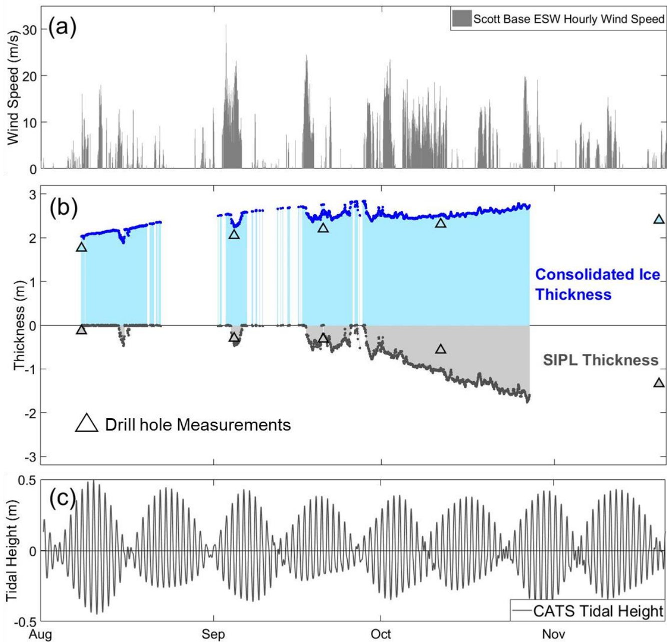
310 Figure 4. Times-series of (a) southwesterly to easterly ( 45\text{-}270^\circ ) hourly wind speeds recorded at the Scott Base EWS (retrieved on the 26 August 2019: http://cliflo.niwa.co.nz ), (b) EM consolidated ice (positive values) and SIPL thickness (negative values) recorded at the Winter EM time-series site near Hut Point Peninsula (Fig. 1) from 8 August to 27 October 2018 with drill hole measurements of consolidated ice and SIPL thickness (triangles), and (c) CATs tidal height.
