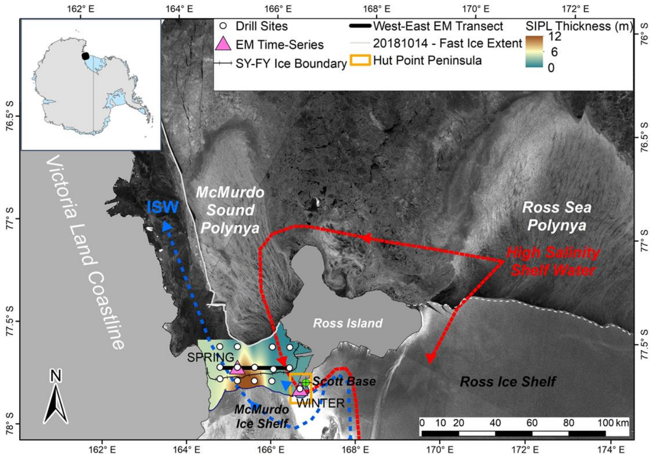
75 80 Figure 1. McMurdo Sound, western Ross Sea, Antarctica (inset map) with dashed lines illustrating HSSW (red), formed within the Ross Sea and McMurdo Sound polynyas, circulating into the conjoined McMurdo-Ross Ice Shelf cavity and ISW (blue) outflow into McMurdo Sound. The late spring fast ice edge (grey line) and boundary between second year (SY) and first year (FY) fast ice present in the study region in 2018 are shown with the locations of the Winter and Spring EM time-series sites (pink triangles) and the Electronic Weather Station (EWS) at Scott Base (green crossed circle). SIPL thickness distribution was spline interpolated from drill hole measurements made at 14 drill sites (white circles) in November 2018, along with repeated west-east EM transects (black line) across McMurdo Sound. At the Spring site, we additionally carried out repeated 200 m x 200 m grid-surveys and collected oceanographic data at a mooring deployed (500 m to the north) in November 2018 (satellite image: Sentinel-1 SAR - 2 October 2018).
