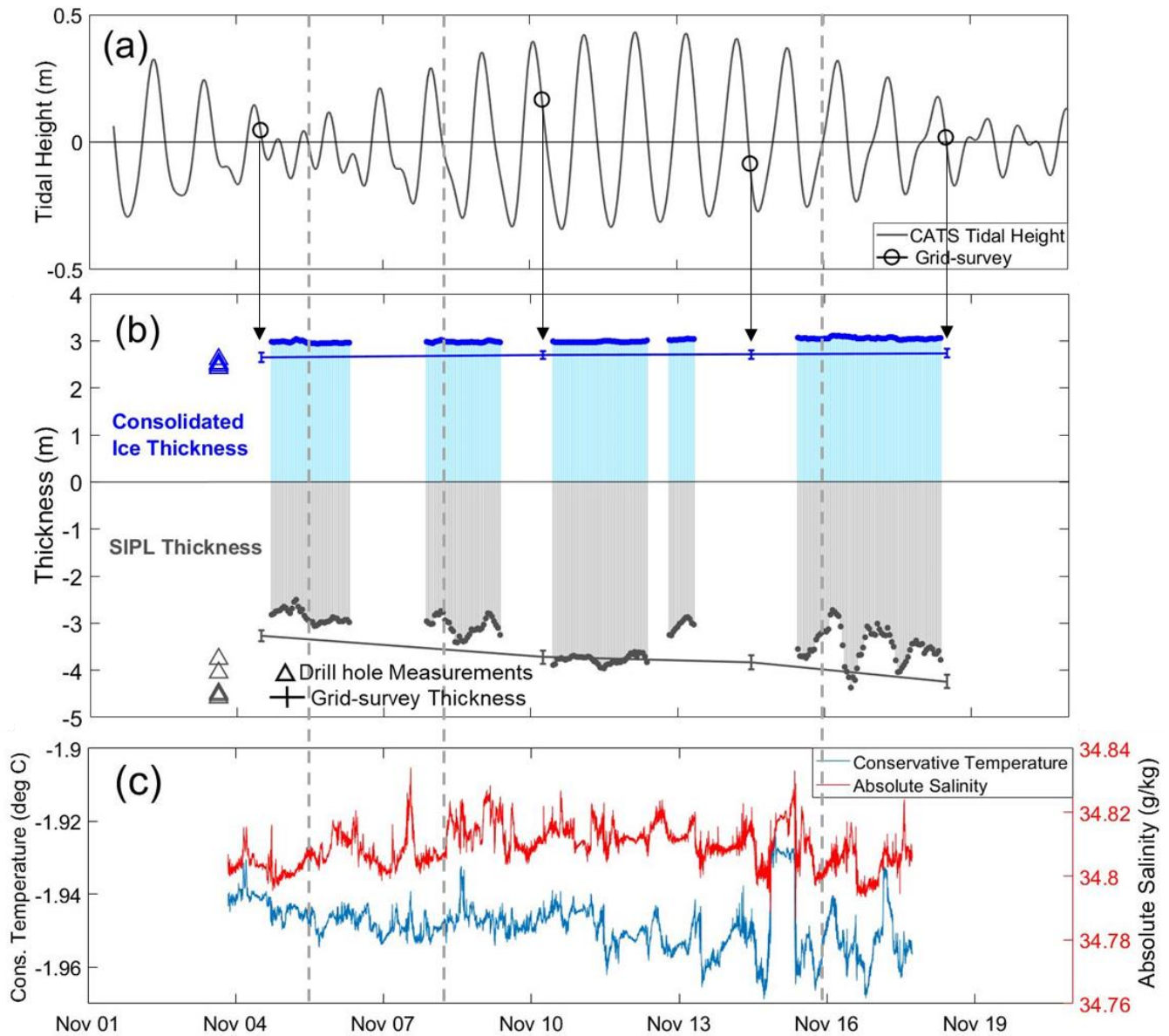
350 355 Figure 5. (a) CATS tidal height with the times of the repeat grid-surveys (circles) shown in (b) as lines of mean EM sea ice and SIPL thickness with standard deviations (vertical bars) plotted with the Spring EM time-series measurements of consolidated ice and SIPL thicknesses and the five drill hole measurements (triangles) of consolidated ice and SIPL thickness made on 3 November 2018. (c) The 101-m depth MicroCAT time-series of absolute salinity and conservative temperature from the oceanographic mooring deployed 500 m due north of the Spring site. Stippled vertical lines show the changes in SIPL thickness with the tides on 5, 8, and 16 which are discussed in sect. 3.1.
