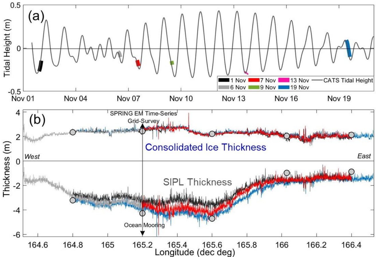
Figure 7. Temporal variability in SIPL thickness on the repeated west-east transect ( latitude 77.767° S ) (refer to Fig. 1 for location) of EM consolidated ice and SIPL across McMurdo Sound with full surveys carried out on the 1 and 19, and partial surveys on the 6, 7, 9, and 13 November (EM surveys on the 9 and 13 are not shown in (b) for clarity). The times of the repeated transects are colour-coded and displayed on the tidal height curve in (a). Drill hole measurements (circles) carried out along the transect between 3-19 November 2018 are also shown. The Spring EM time-series site, and grid-
