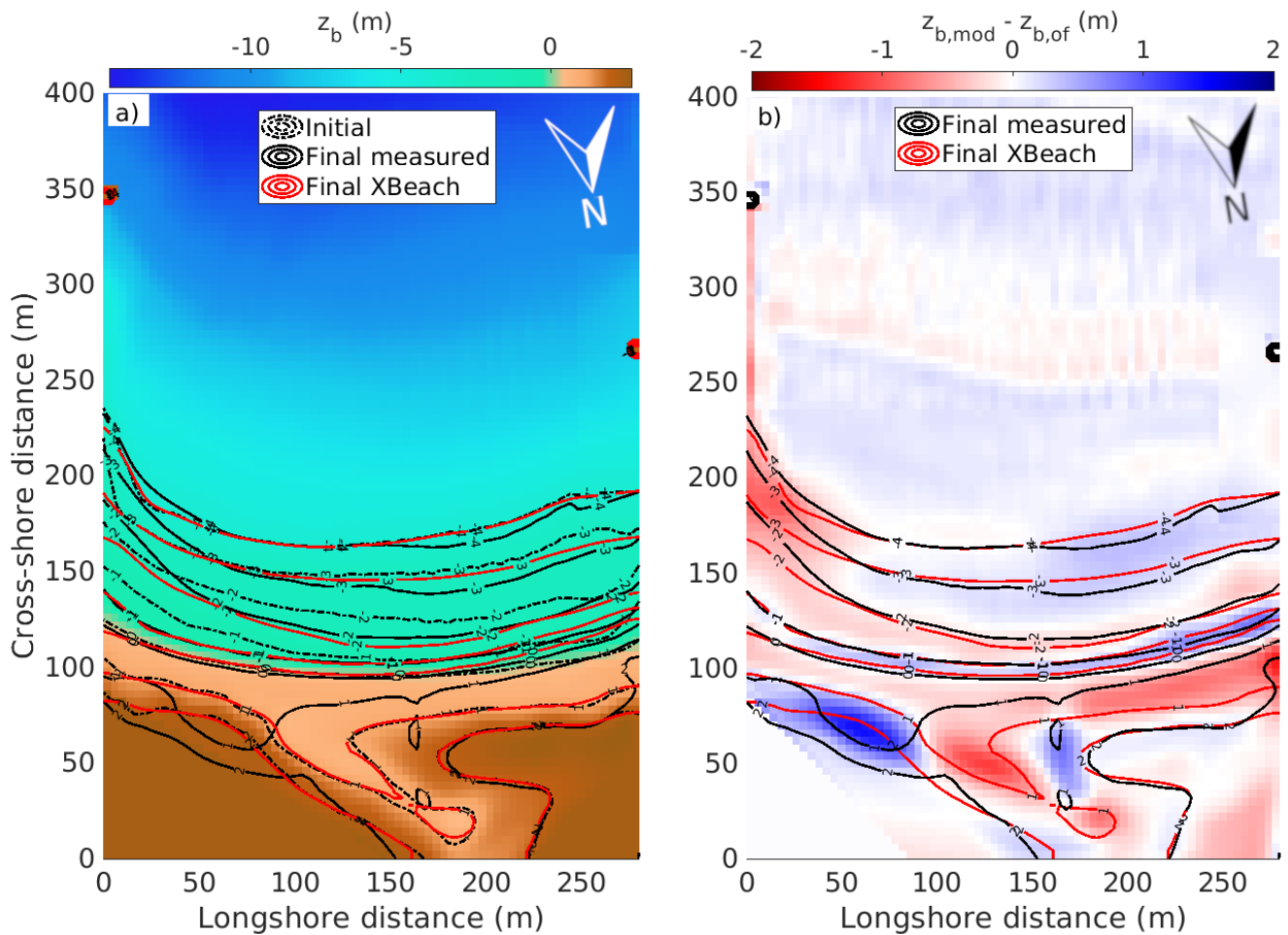
Figure 6. Panel a: Comparison between the final topobathymetry modelled by XBeach (red solid contours), the final observed one in July 2020 (black solid contours) and the initial one of January 2020 (black dashed contours and background colours). Panel b: Difference between the final modelled and observed topobathymetries (background colours), with the modelled and observed topobathymetric contours in red and black, respectively. The calibrated parameter values were used (Table 2), with the wave and sea level measured by the AWAC.
