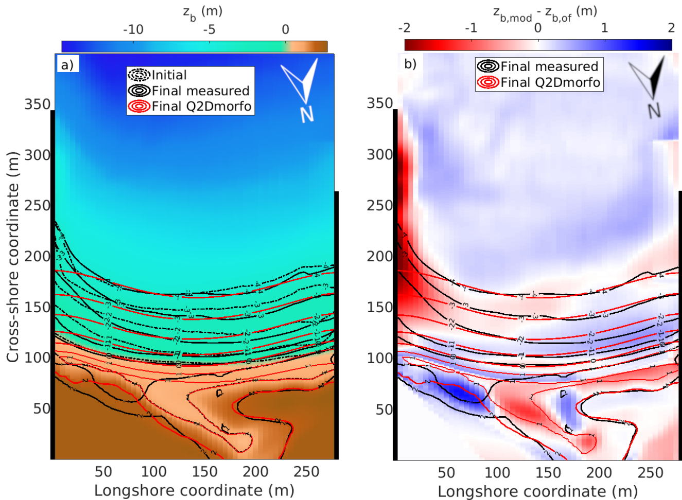
Figure 7. Panel a: Comparison between the final topobathymetry modelled by Q2Dmorfo (red solid contours), the final observed one in July 2020 (black solid contours) and the initial one of January 2020 (black dashed contours and background colours). Panel b: Difference between the final modelled and observed topobathymetries (background colours), with the modelled and observed topobathymetric contours in red and black, respectively. The calibrated parameter values were used (Table 3), with the wave and sea level measured by the AWAC.
