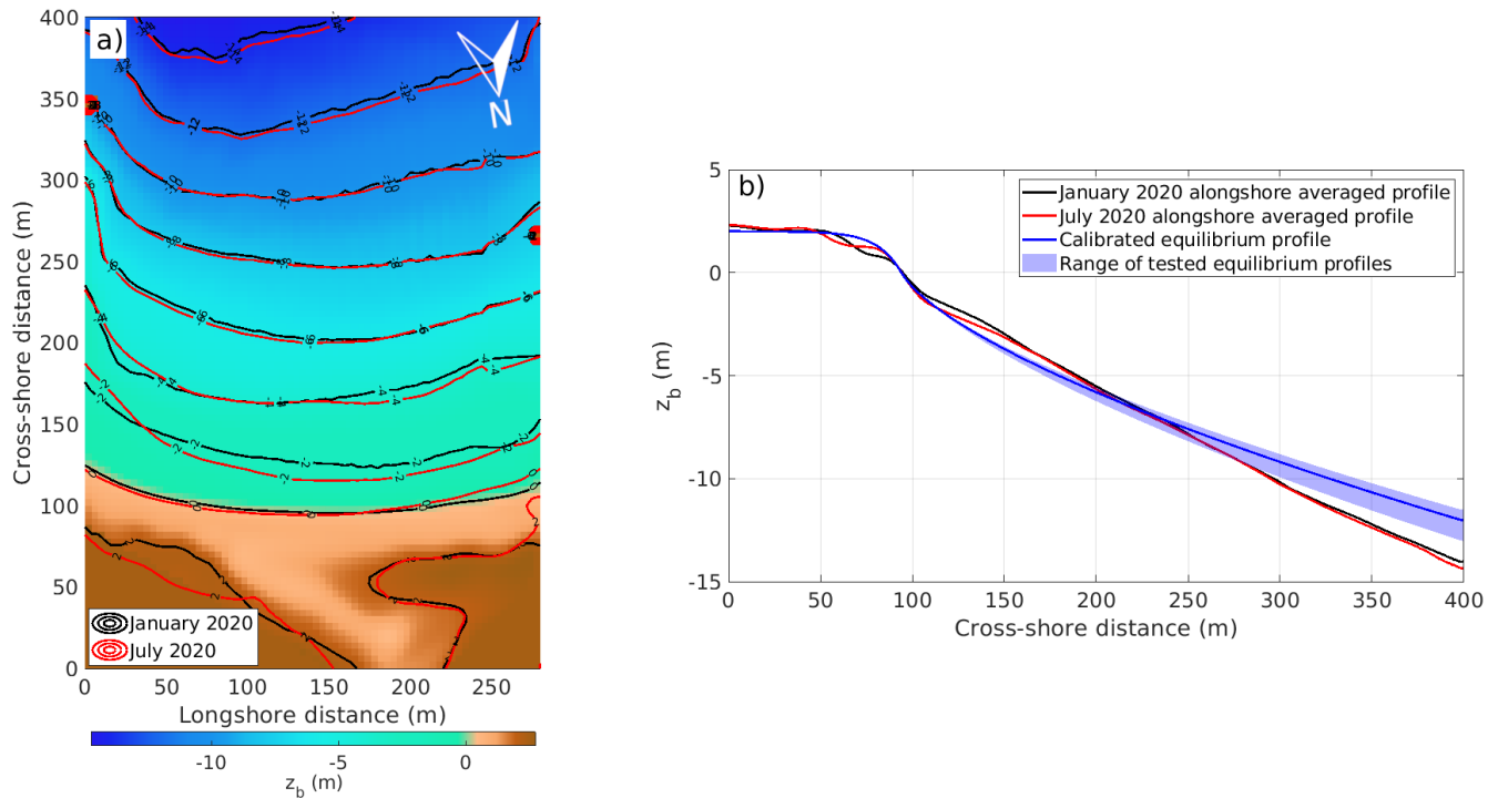
Figure 2. Topobathymetric surveys in January and July 2020 within the model domain oriented using the local coordinate system (x, y) shown in Fig. 1 (panel a), and their alongshore averaged cross-shore profiles (panel b). Panel b) also shows the range of tested equilibrium profiles in light blue and the calibrated equilibrium profile in dark blue used in the Q2Dmorfo model. In both panels January is represented in black lines and July in red lines. The background colours in the left panel correspond to January 2020.
