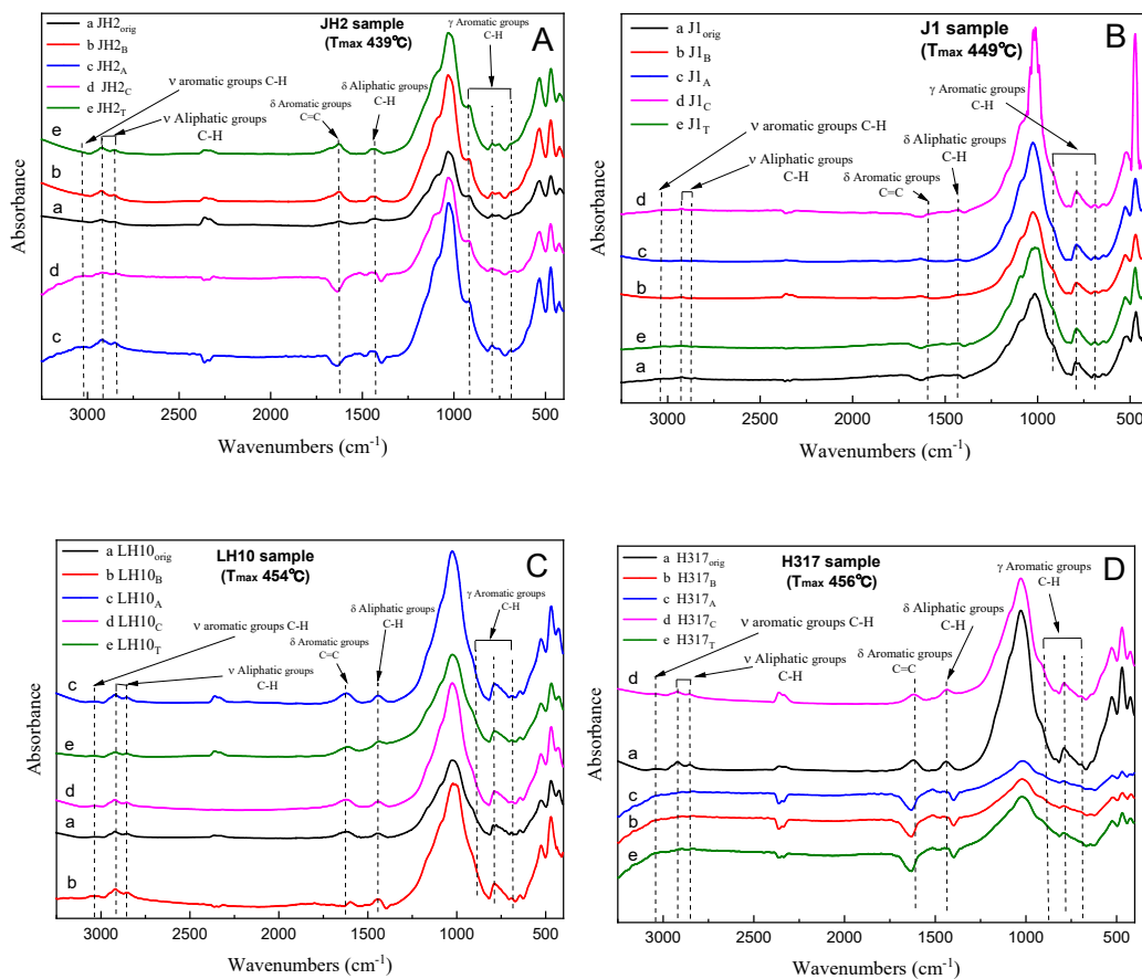
150 Fig. 5. FTIR spectra of original (a) marginally mature sample JH2 orig ( T_{max}=439^{\circ}\text{C} ) (b) the mature sample J1 orig ( T_{max}=449^{\circ}\text{C} ) (c) late mature sample LH10 orig ( T_{max}=454^{\circ}\text{C} ) and (d) late mature sample H317 orig ( T_{max}=456^{\circ}\text{C} ).
