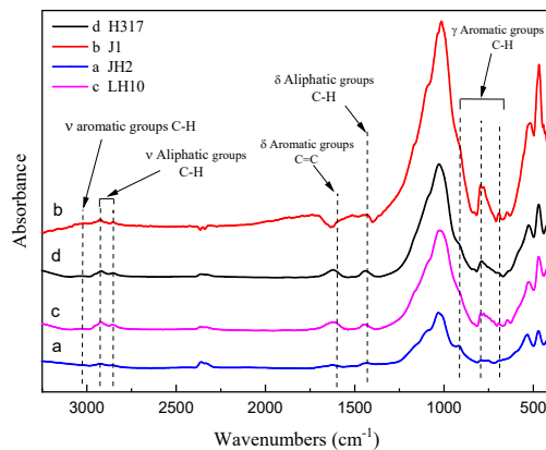
150 Fig. 5. FTIR spectra of original (a) marginally mature sample JH2 orig ( T_{max}=439^{\circ}\text{C} ) (b) the mature sample J1 orig ( T_{max}=449^{\circ}\text{C} ) (c) late mature sample LH10 orig ( T_{max}=454^{\circ}\text{C} ) and (d) late mature sample H317 orig ( T_{max}=456^{\circ}\text{C} ).
