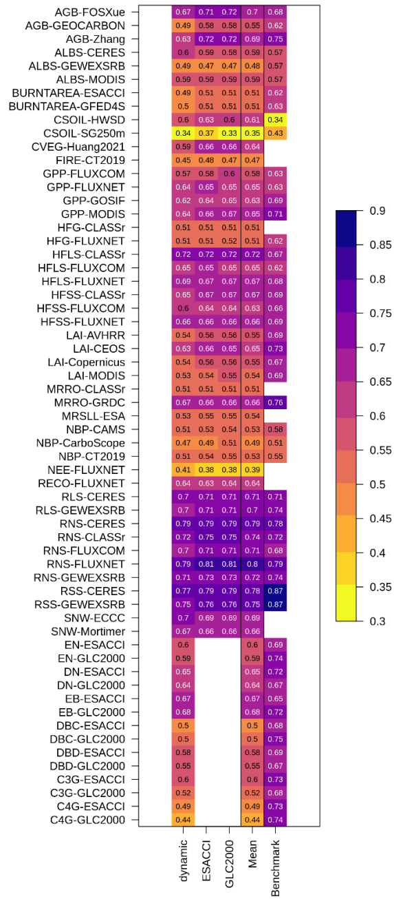
Figure B3: Scores of model performance in reproducing observation-based datasets of principal C, water, and energy variables as well as land cover fractions of each natural plant functional type (PFT) for simulations of CLASSIC with prescribed land cover (with an ESACCI-derived land cover forcing and a GLC2000-derived land cover forcing) and dynamic land cover. Abbreviations for C, water, and energy variables and observation-based datasets are described in the Methods. Abbreviations for PFTs are evergreen needleleaf (EN), deciduous needleleaf (DN), evergreen broadleaf (EB), deciduous broadleaf cold (DBC), deciduous broadleaf dry (DBD), C 3 grass (C3G), and C 4 grass (C4G).
