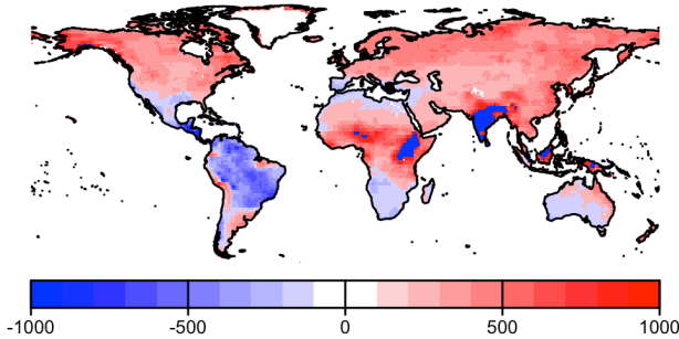
Figure B6: Temperature and precipitation in ab. the historical period (averaged over 1995-2015), cd. SSP5-8.5 (averaged over 2080-2100), and ef. change between the historical period and SSP5-8.5.
