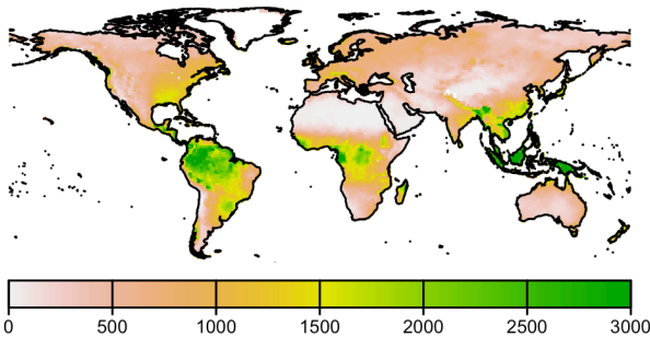
c Historical precipitation
