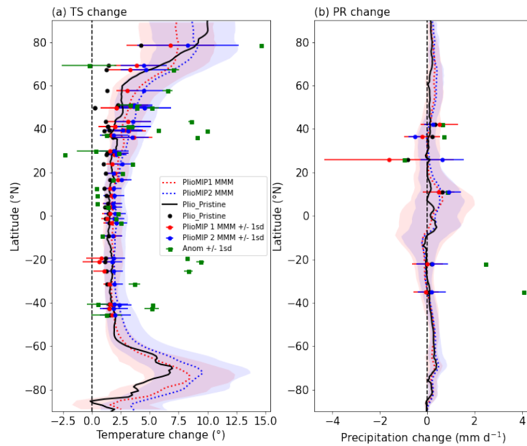
Figure 2. Zonal averaged changes in mean annual (a) surface temperature in ^{\circ}\text{C} and (b) precipitation in \text{mm d}^{-1} . In all panels, black solid lines show the simulated anomalies (Plio_Pristine - PI). Dotted lines represent the multi-model means of the PlioMIP1 (red, Haywood et al., 2013) and PlioMIP2 (blue, Haywood et al., 2020) respectively, with shaded areas showing the model spread, i.e. the standard deviation of the ensemble. Green squares show the site-level reconstructions in Fig. 1, and dots show the corresponding grid-level anomalies with error bars showing the range of the PlioMIPs.
