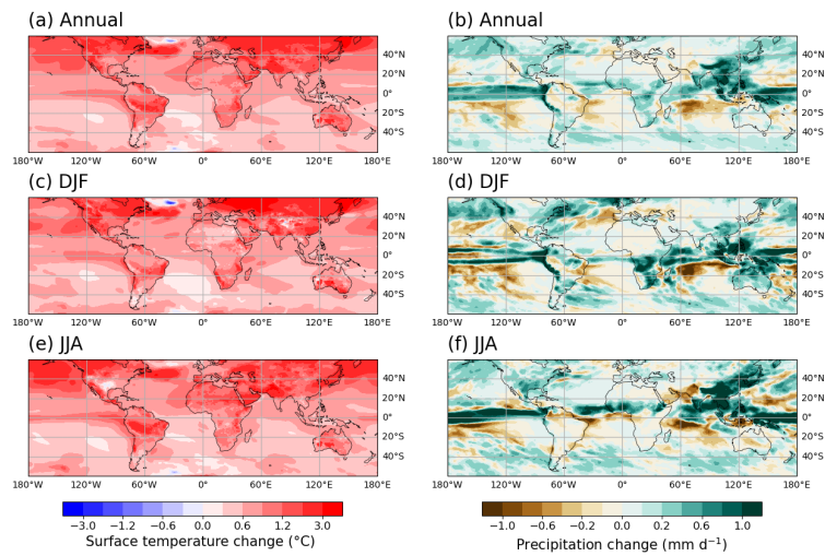
Figure 5. Annual, DJF and JJA mean surface temperature change in °C (a, c, e) and precipitation change in mm d -1 (b,d,f) after removal of anthropogenic emissions (Plio_Pristine - Plio_Polluted) Annual, DJF and JJA mean surface temperature change in °C (a, c, e) and precipitation change in mm d -1 (b,d,f) after removal of anthropogenic emissions (Plio_Pristine - Plio_Polluted).
