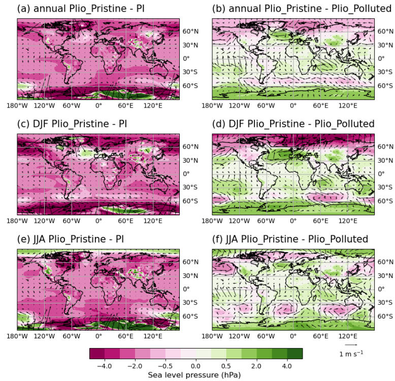
Figure 10. Changes in annual and seasonal sea level pressure (hPa) and surface wind ( \text{m s}^{-1} ) during the mPWP (Plio_Pristine - PI, left column) and after removal removal of anthropogenic aerosols (Plio_Pristine - Plio_Polluted, right column).
