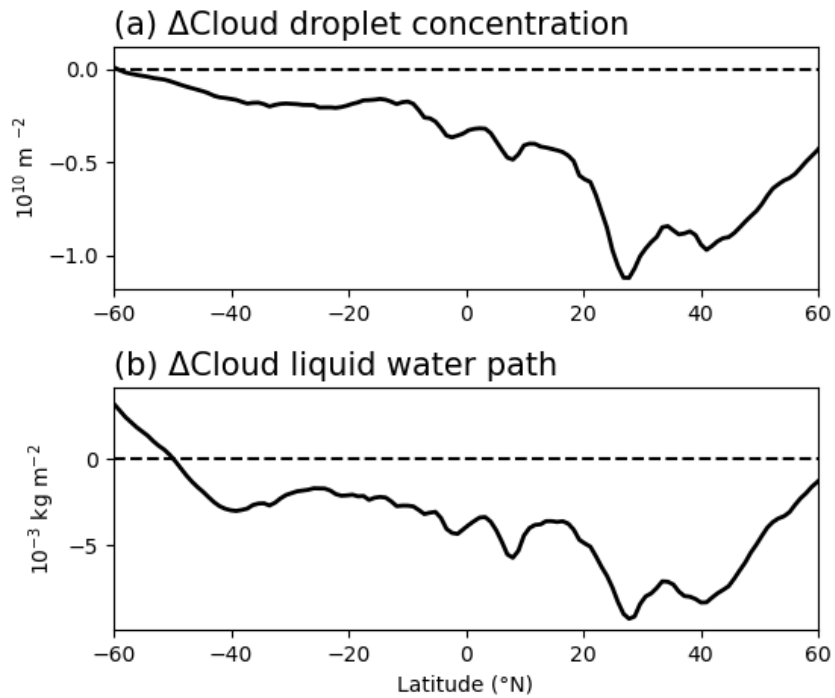
Figure 9. Zonal-averaged change in (a) cloud droplet concentration in \text{m}^{-2} and (b) cloud liquid water path in \text{kg m}^{-2} . Zonal averaged change (Plio_Pristine - Plio_Polluted) in (a) cloud droplet concentration in \text{m}^{-2} and (b) cloud liquid water path in \text{kg m}^{-2} . The corresponding spatial relative change are given in Fig. A3.
