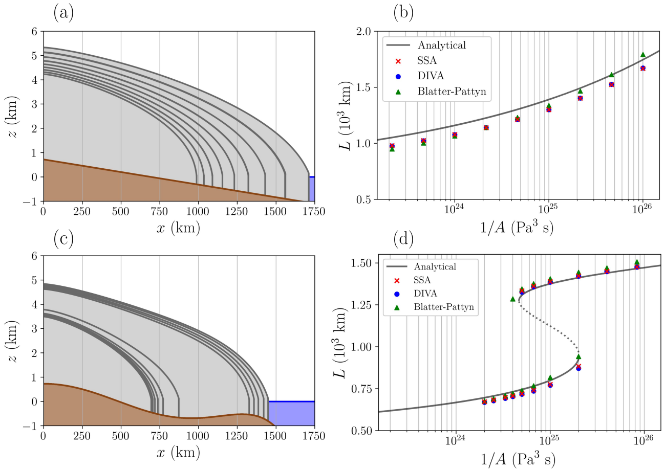
Figure 3. Left column: ice-sheet extent. Right column: grounding-line position as a function of the MISIP forcing A for three independent Stokes approximations: SSA, DIVA and Blatter-Pattyn. Grey line represents the analytical solution at equilibrium from Schoof (2007b): solid line, stable branch; dashed line, unstable branch. Markers represent Nix’s results after the equilibration time given in Pattyn et al. (2012). Bed geometries correspond to: first row, Experiments 1 and 2 (both advance and retreat); second row, Experiment 3.
