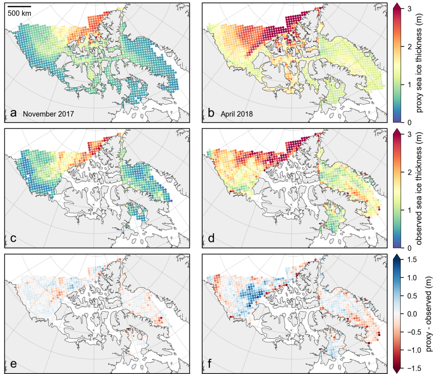
Figure 7. (a,b) proxy Proxy sea ice thickness (without correction) , (c,d) CryoSat-2 observed sea ice thickness, (e,f) proxy SIT-observed SIT, for (a,c,e) November 2017 and (b,d,f) April 2018, when leaving the winter 2017-2018 season of CryoSat-2 ice thickness data out of the model training dataset.
