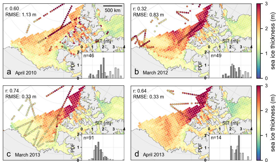
Figure 9. Operation IceBridge sea ice thickness measurements compare to the proxy corr sea ice thickness ( without correction ) product for (a) April 2010, (b) March 2012, (c) March 2013, (d) April 2013. Subfigure shows the PDF probability density function for OIB (lightgrey) and the proxy SIT product (darkgrey) on the OIB tracks.
