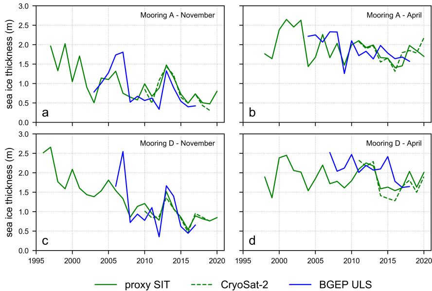
Figure 8. BGEP ULS moorings sea ice thickness compared to the proxy _corr sea ice thickness product ( without correction ) and CryoSat-2 observed sea ice thickness at the same location, (a) November mooring A, (b) April mooring A, (c) November mooring D, (d) April mooring D. Locations of ULS moorings are shown in Figure 1.
