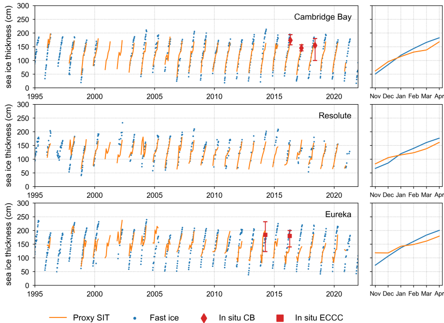
Figure 10. Fast ice thickness measurements (for locations see Fig 1), proxy_corr sea ice thickness product (without correction), and field campaign in-situ observations from ECCC in Eureka (King et al., 2015, 2020) and Cambridge Bay. Graphs on right-hand side show mean seasonal cycle for each location.
