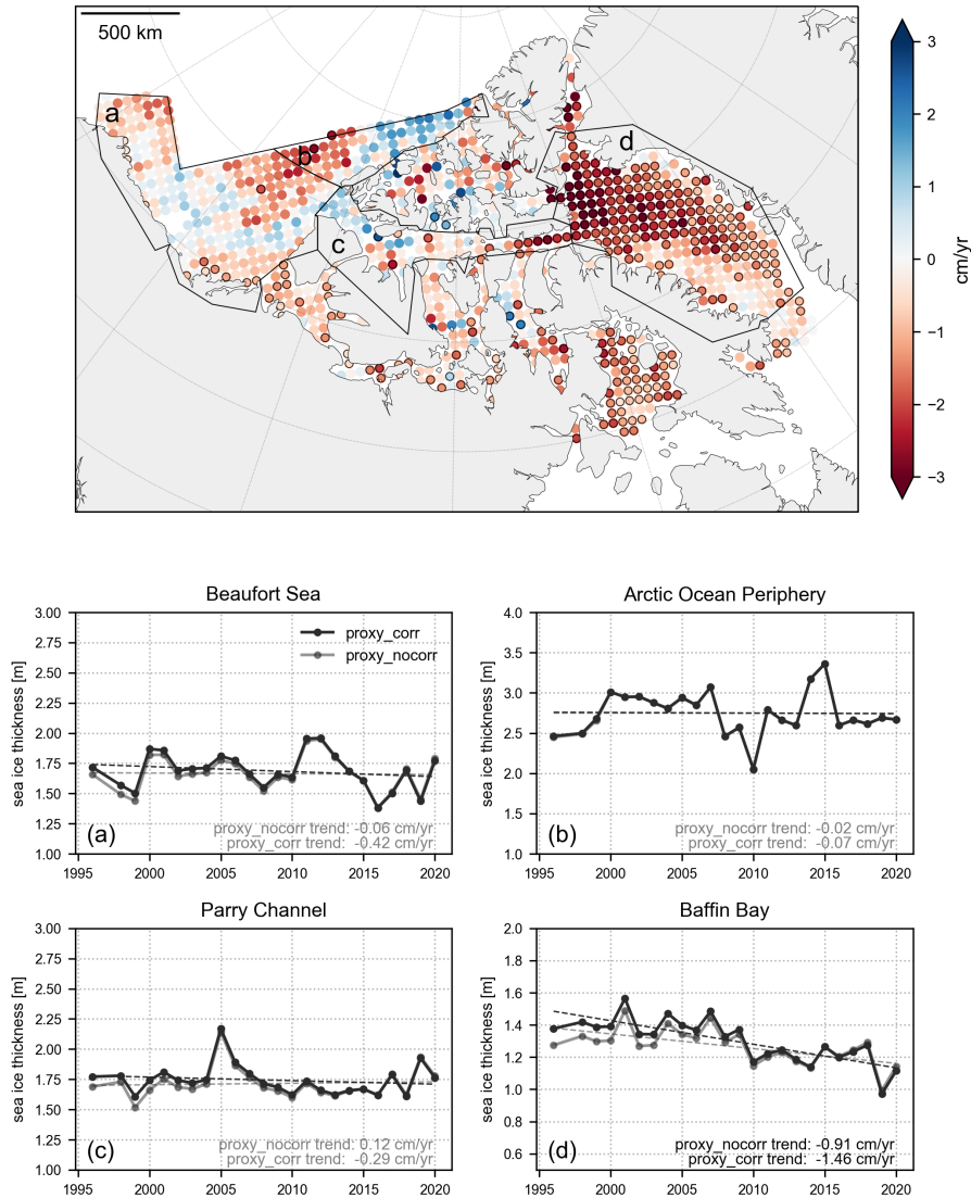
Figure 12. Sea ice thickness trends from the proxy product for April 1996-2020. Solid —The map shows trends from the proxy_corr SIT product, solid outline circles where statistically significant ( p < 0.05 ), weaker circle where the corrected version is statistically significant ( p < 0.05 ), but the original version is not. Colours show the trend for the not-corrected version. Timelines given for the mean of subregions of the Canadian Arctic (a,b,c,d). Trends shown for the original proxy-product proxy_nocorr SIT product (light) and the corrected-proxy_corr SIT product (dark). Trends shaded when not Trend numbers are bold where significant ( p > 0.05 ).
