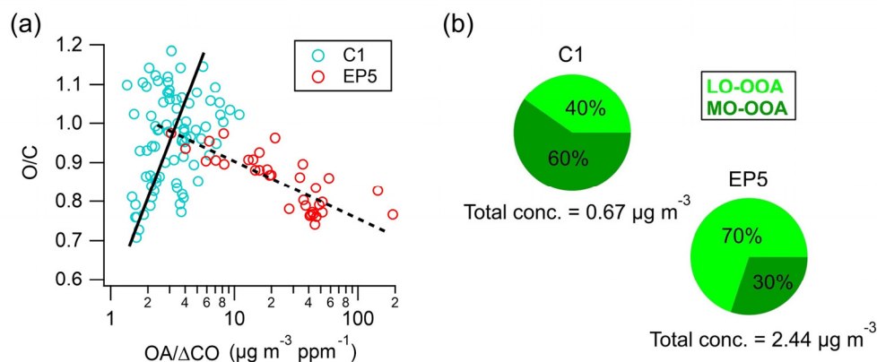
395 Figure 9. (a) Scatter plot of O/C as a function of OA/ΔCO values and (b) mass concentrations and proportions of MO-OOA and LO-OOA during C1 and EP5.
