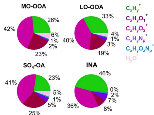
350 Figure 7. Mass fractional composition of OA ion families for the resolved four PMF factors.
