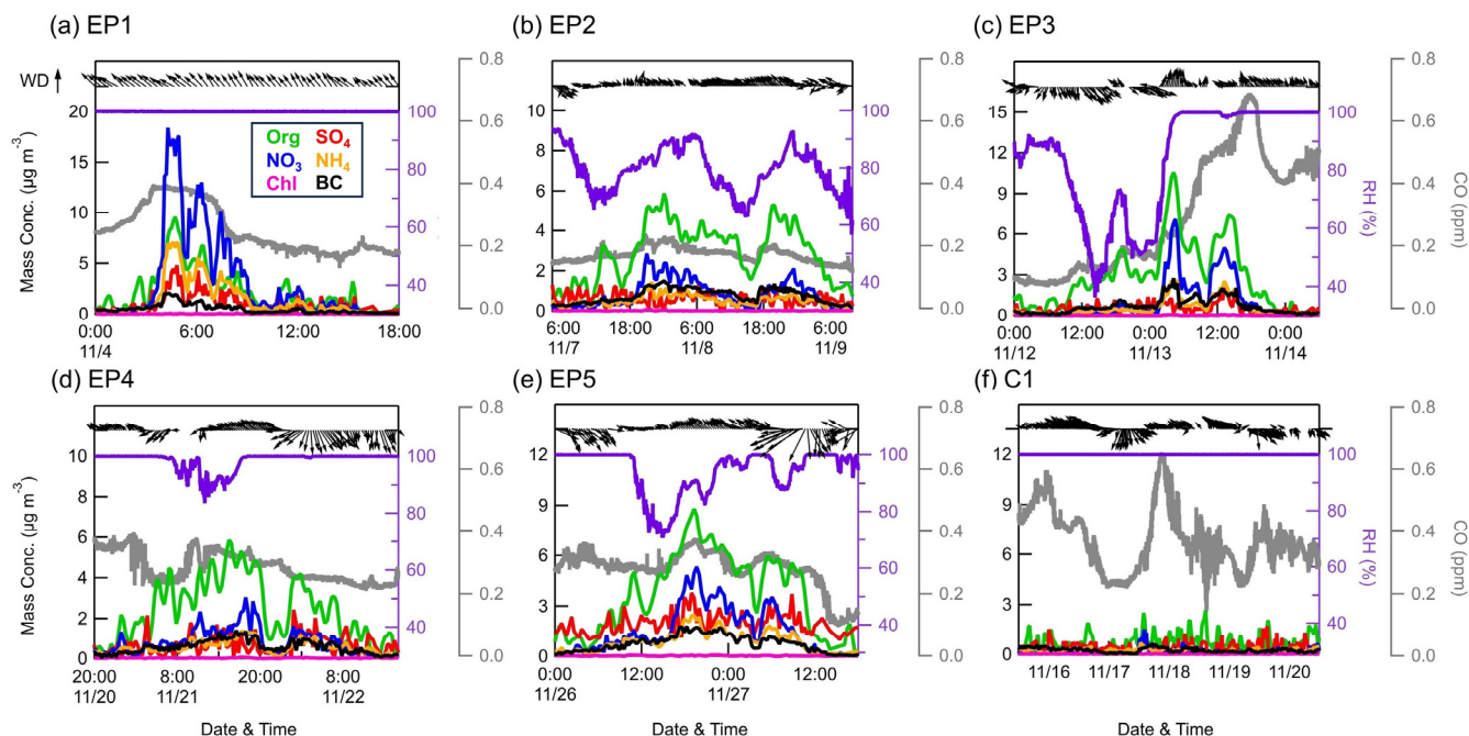
Figure 3. Temporal variations of the concentrations of PM 1 species measured by ACSM, as well as CO (grey lines), RH (purple lines), and WD/WS (black arrows) during six events.
