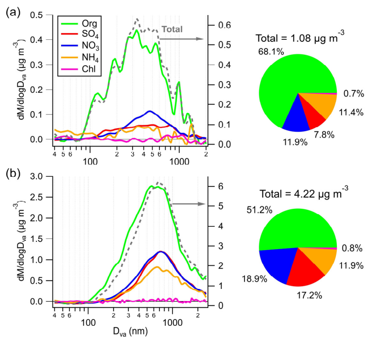
315 Figure 4. Averaged size distributions and chemical composition of NR-PM 1 during (a) C1 and (b) EP5.
