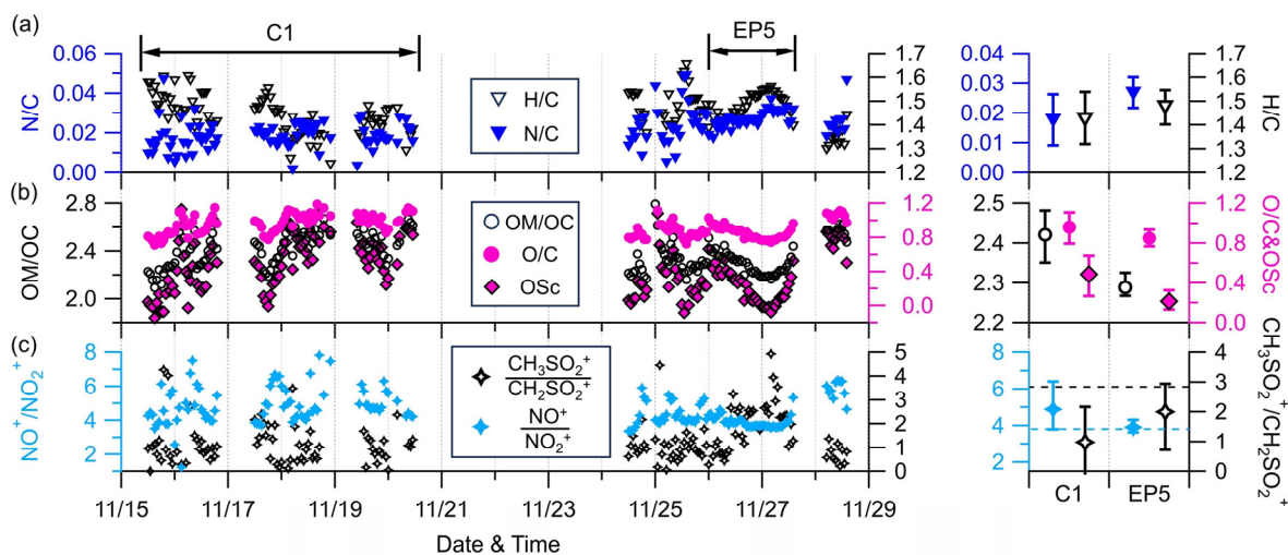
Figure 5. Time series of 1-hour averaged (a) N/C and H/C, (b) OM/OC, OSc, and O/C, and (c) \text{NO}^+/\text{NO}_2^+ and \text{CH}_3\text{SO}_2^+/\text{CH}_2\text{SO}_2^+ during the AMS sampling site (left) and their mean values in C1 and EP5 (right). Only ratios determined with good S/N (i.e., organics > 0.7 \mu\text{g m}^{-3} ) are shown. The horizontal black and blue dash line in the
