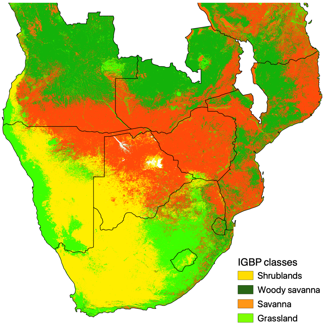
Figure 2. Distribution of the IGBP landcover classes used in figure 7 of the main text.
