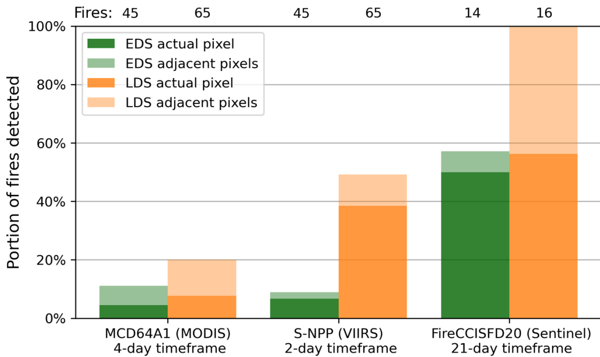
Figure 10. Detection of the fires measured using the UAS-methodology by different satellite algorithms in the EDS (green) and LDS (orange). The darker area represents the cases where a fire was observed in the actual pixel within the listed timeframe. The lighter areas represent fires that were not detected in the same pixel as the samples but were detected in adjacent pixels. Timeframes are listed below the product labels. For the VIIRS detections the distance limits between the detection point and closest sample of the fire were 1km for the darker shaded area and 3.5 km for the lighter shaded area.
