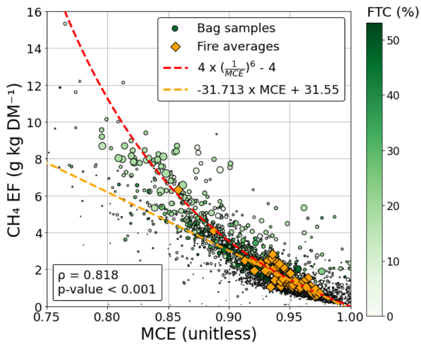
Figure 1. The non-linear regression between the CH 4 EF and the MCE for the individual bag samples. In the box on the bottom left, \rho refers to Spearman's rank correlation coefficient measured in the bag samples. The orange linear regression line is the linear regression of fire-averages.
