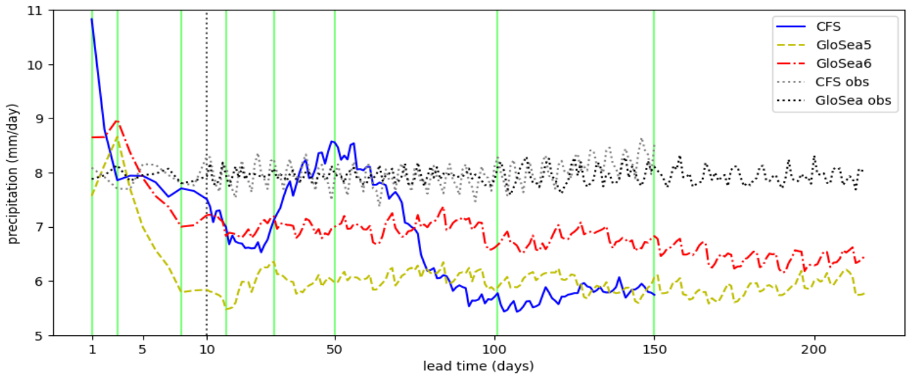
Figure A4. As Fig. 2 but with only 3 of the 7 ensemble members in GloSea.
