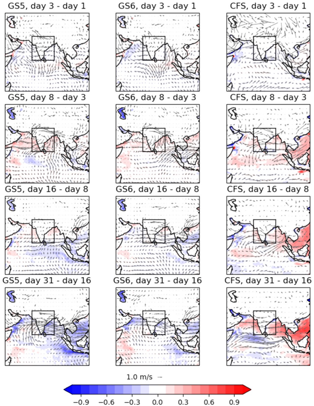
Figure 4. SST differences (colours, in K) and 850-hPa wind differences (vectors; note that this field is identical to that in Fig. 3) in GloSea5 (left column), GloSea6 (centre column) and CFSv2 (right column), between the hindcast lead times shown, averaged over June–August 2002–2015. The black boxes show the evaluation region (8N–29N, 69E–89E) used throughout this study.
