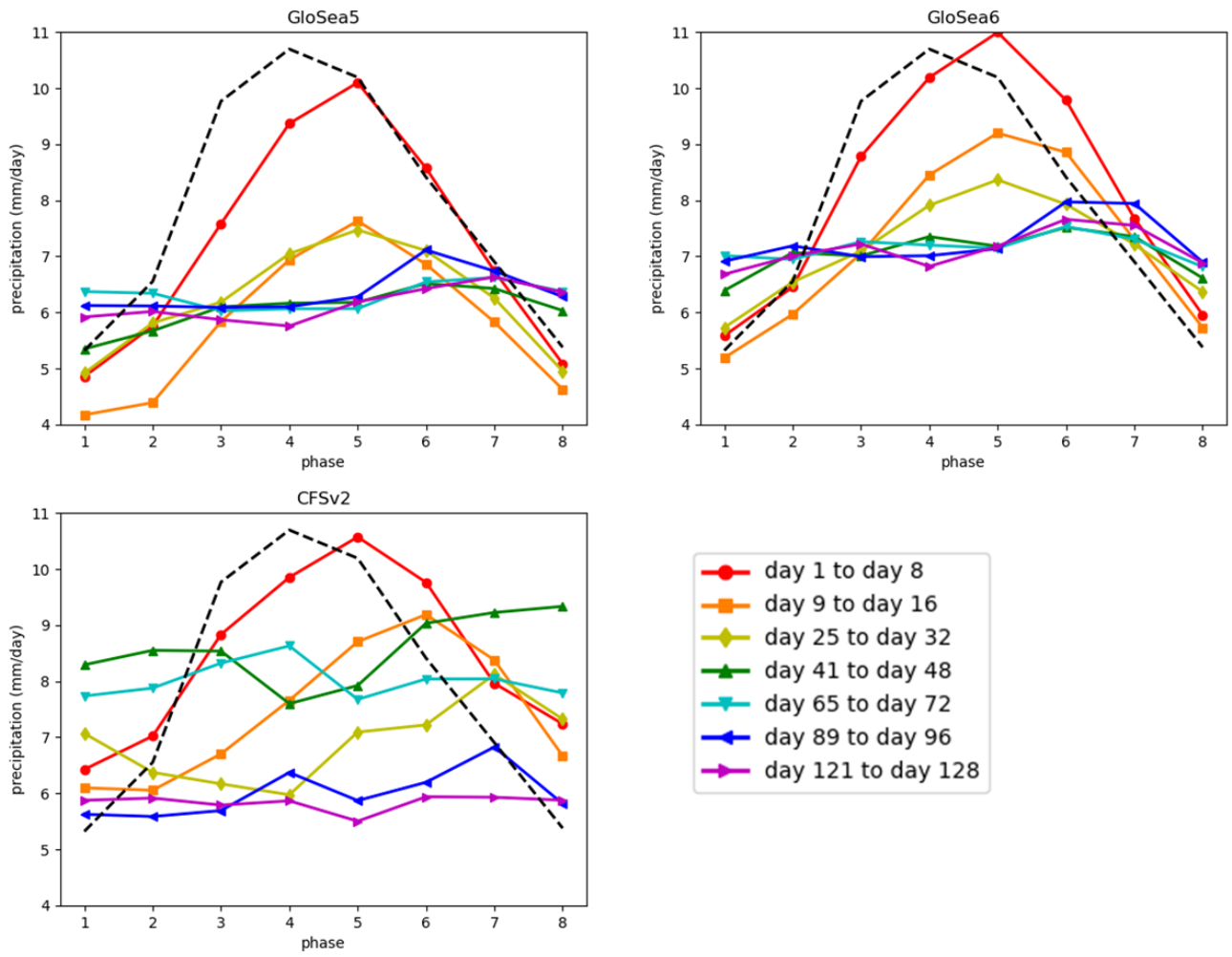
Figure A13. As Fig. 13 but with GloSea5 hindcasts valid during 1994–2015 and GloSea6 hindcasts valid during 1994–2016 (all other data unchanged, i.e., the black dashed lines refer to observations during 2002–2015 in all three panels).
