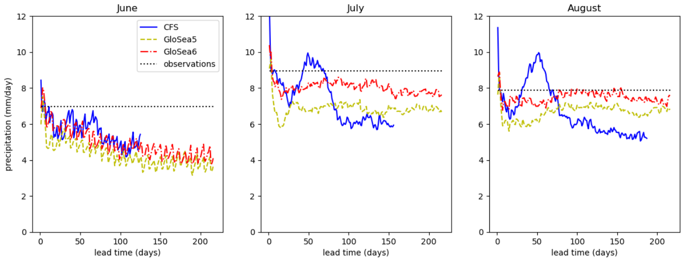
Figure 9. Variation of precipitation with hindcast lead time (averaged over 8N–29N, 69E–89E and 2002–2015) for hindcasts valid in each of June, July and August. The dotted lines show observed values averaged over all dates in the month (i.e., not just dates on which hindcasts are available).
