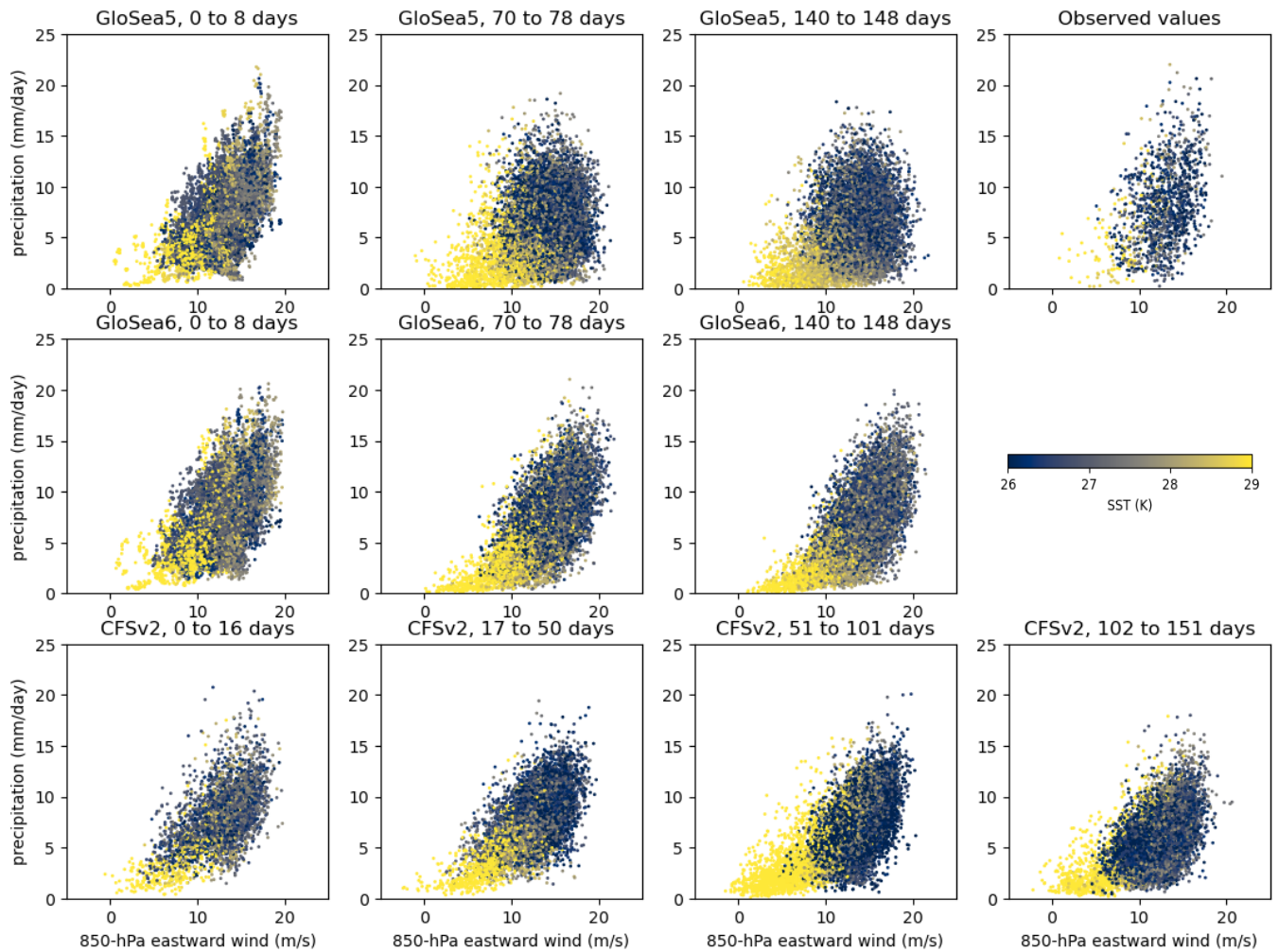
305 Figure 8. Scatter plots of precipitation over India (8–29N, 69–89E) against 850-hPa eastward wind over the Arabian Sea (0–21N, 49–69E), coloured by SST over the Arabian Sea. Each dot represents a single hindcast for one year during 2002–2015, one day in June, July or August and one lead time within the range shown.
