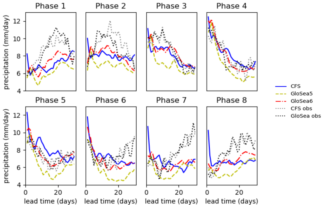
Figure A14. As Fig. 14 but including start dates up to 31st August and only to 30 days' hindcast time.
