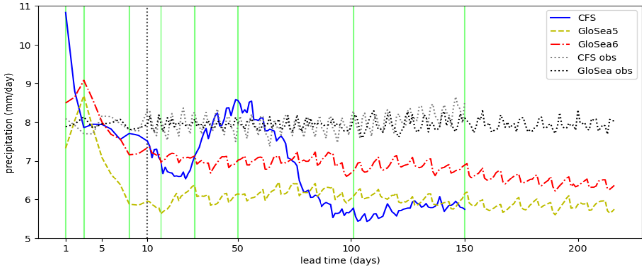
530 Figure A5. As Fig. 2 but with GloSea5 hindcasts valid during 1994–2015 and GloSea6 hindcasts valid during 1994–2016 (all other data unchanged, i.e., “GloSea obs” still refers to the period 2002–2015).
