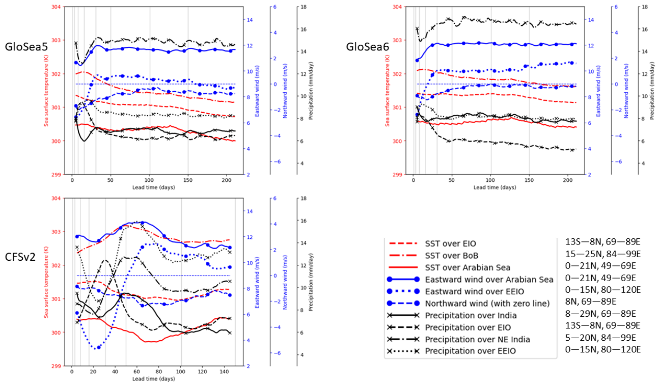
355 Figure 11. SST, 850-hPa wind and precipitation averaged over different regions (shown in Fig. 5), averaged over July 2002–2015, as a function of lead time. A smoothing is applied by taking a 9-day running average in the lead-time direction.
