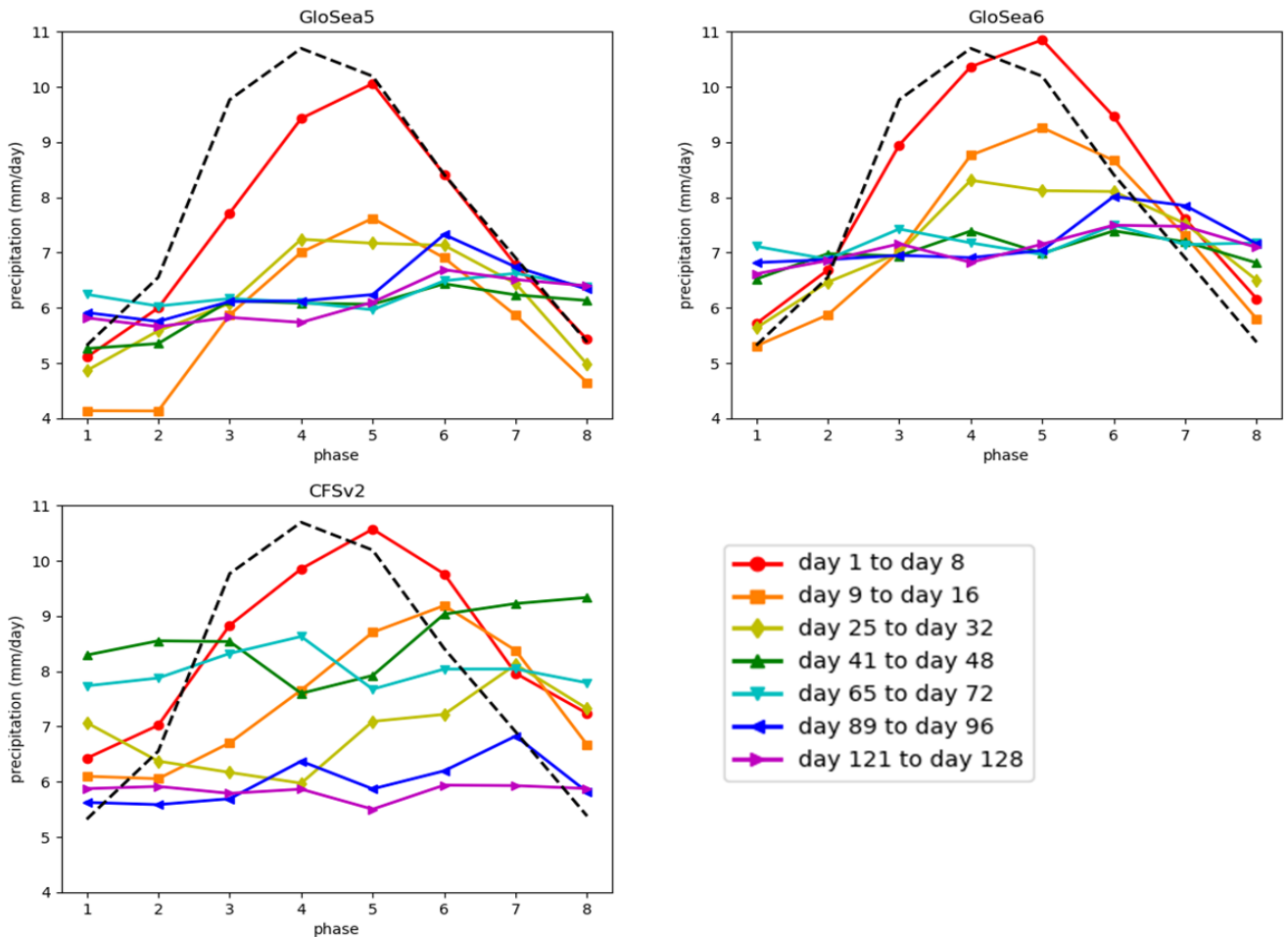
Figure 13: Variation in precipitation (averaged over 8N–29N, 69E–89E and June–August 2002–2015) with lead time as a function of observed BSISO phase at valid time, averaged over 8-day lead time blocks (coloured lines). Each panel corresponds to a model denoted by its title. Observed precipitation corresponding to each BSISO phase is denoted by the black dashed line in all three panels.
