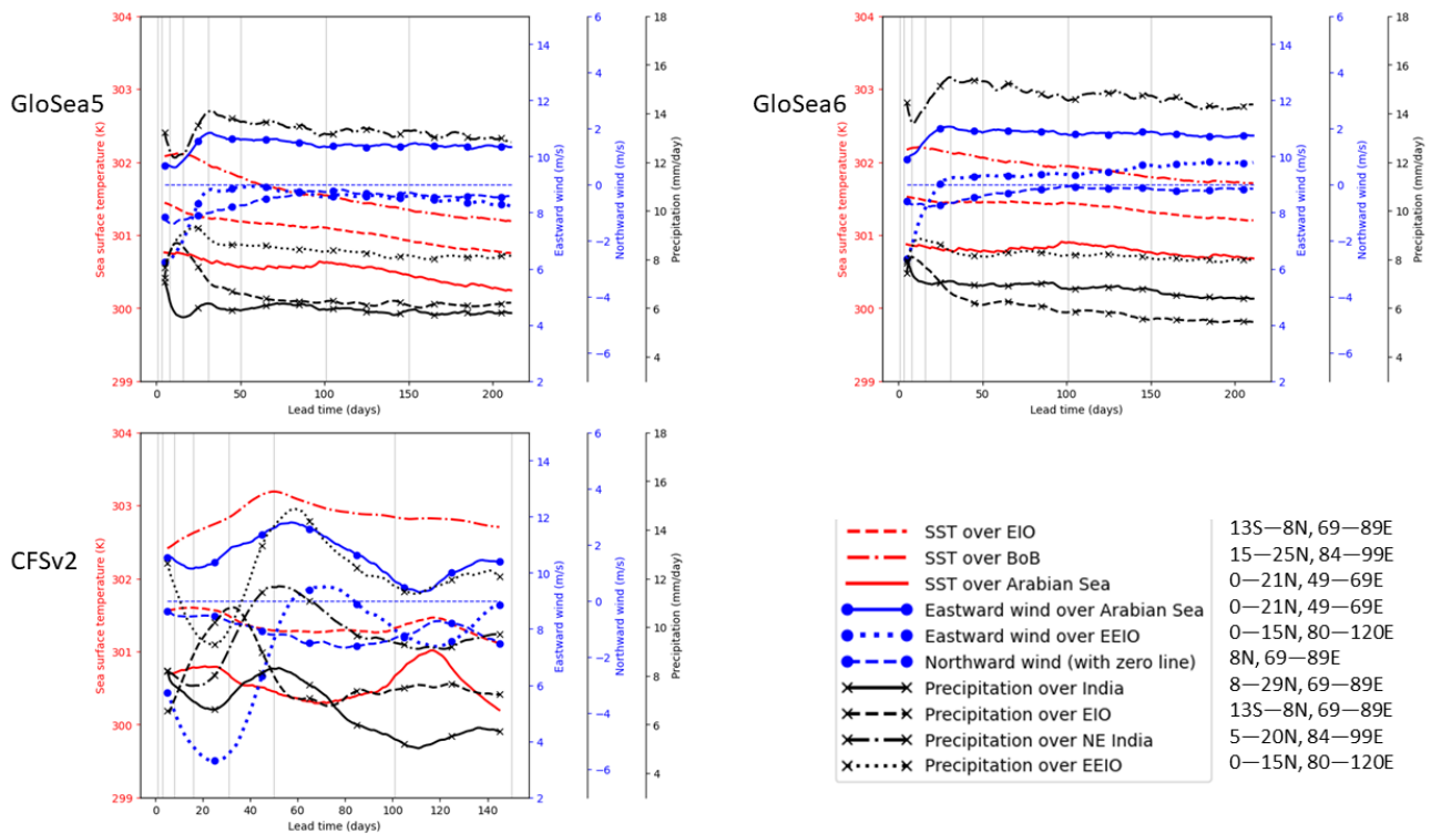
260 Figure 7. SST, 850-hPa wind and precipitation averaged over different regions (shown in Fig. 5), averaged over June–August 2002–2015, as a function of lead time. A smoothing is applied by taking a 9-day running average in the lead-time direction.
