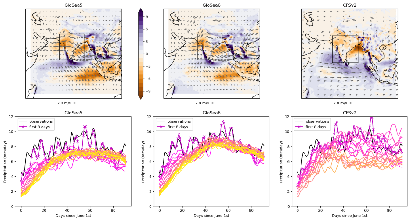
135 Figure 1. Top row: Overall biases averaged over valid times in June–August 2002–2015 and initial times during May. Variables are precipitation in mm/day (bias against IMERG observations) and 850-hPa horizontal wind (bias against ERA5 reanalysis). Bottom row: Seasonal cycle of precipitation in hindcasts and IMERG observations, averaged over June–August 2002–2015, 8N–29N, 69E–89E (region denoted by the black boxes in the panels in the top row). Hindcasts are grouped into 8-day lead time sections and depicted in colours ranging with increasing lead time from magenta (darker, for lead times of 1–8 days) to yellow (lighter, for lead times of 199–216 days). Quantities are smoothed in the time-of-year direction with a 1-2-1 filter. 140
