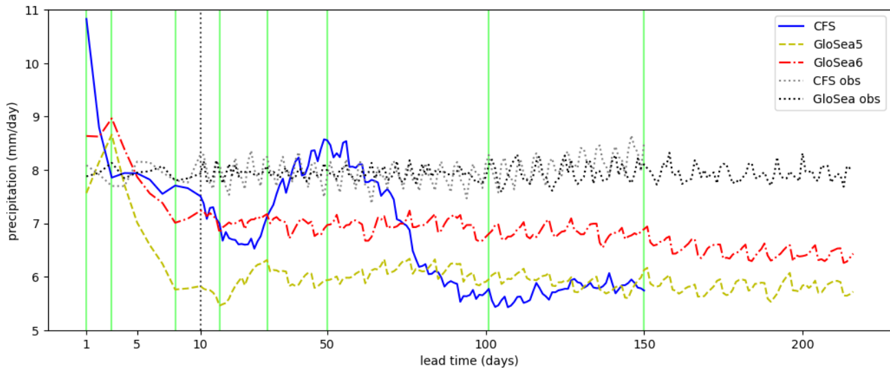
160 Figure 2. Variation of precipitation (averaged over 8N–29N and 69E–89E and June–August 2012–2015) with hindcast lead time in different seasonal forecasting systems. The dotted lines show observed (IMERG) values averaged over the dates on which hindcasts were available in the specified system at that lead time. The green vertical lines show the lead times used in Figs. 3–6 (1, 3, 8, 16, 31, 50, 101 and 150 days). Note that the horizontal scale is larger for lead times less than 10 days than for lead times greater than 10 days (so that it is different either side of the vertical dotted grey line).
