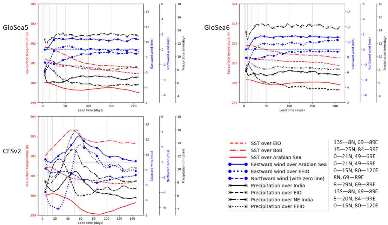
Figure 12. SST, 850-hPa wind and precipitation averaged over different regions (shown in Fig. 5), averaged over August 2002–2015, as a function of lead time. A smoothing is applied by taking a 9-day running average in the lead-time direction.
