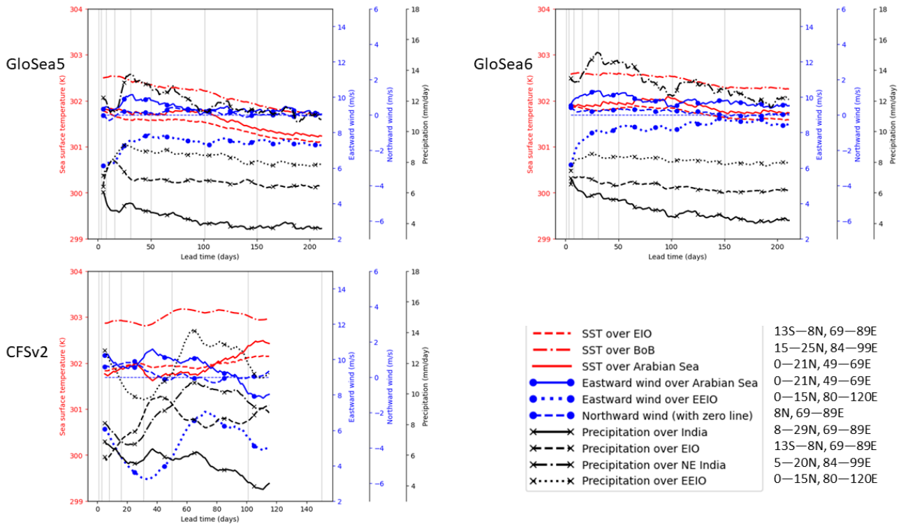
Figure 10: SST, 850-hPa wind and precipitation averaged over different regions (shown in Fig. 5), averaged over June 2002–2015, as a function of lead time. A smoothing is applied by taking a 9-day running average in the lead-time direction.
