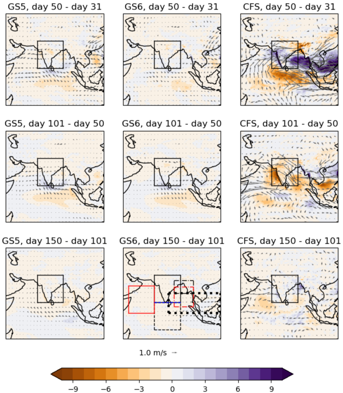
195 Figure 5. Precipitation differences (colours, in mm/day) and 850-hPa wind differences (vectors) in GloSea5 (left column), GloSea6 (centre column) and CFSv2 (right column), between two fields at (top row) and averaged over 30 days centred on (centre and bottom rows) the two hindcast lead times shown above the panel. The black boxes show the evaluation region (8N–29N, 69E–89E) used throughout this study and the boxes in the bottom centre panel show the regions used in Figs. 7, 8, 10, 11 & 12.
