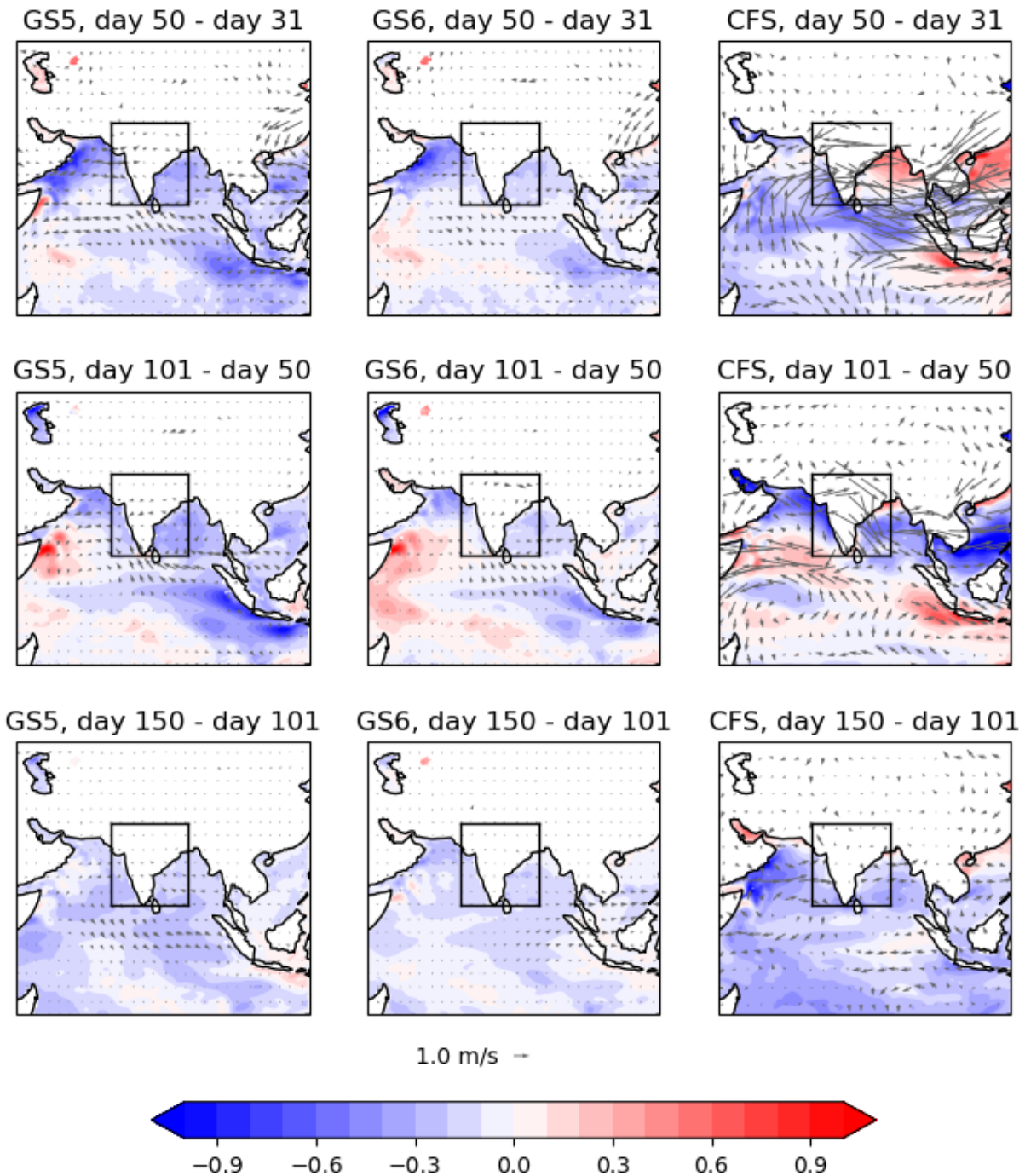
200 Figure 6. SST differences (colours, in K) and 850-hPa wind differences (vectors; note that this field is identical to that in Fig. 5) in GloSea5 (left column), GloSea6 (centre column) and CFSv2 (right column), between two fields at (top row) and averaged over 30 days centred on (centre and bottom rows) the two hindcast lead times shown above the panel. The black boxes show the evaluation region (8N–29N, 69E–89E) used throughout this study.
