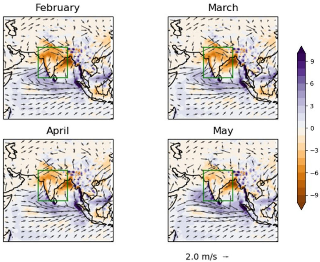
Figure A15. Overall CFSv2 biases averaged over valid times in June–August 2002–2015 and initial times in the month shown. Variables are precipitation in mm/day (bias against IMERG observations) and 850-hPa horizontal wind (bias against ERA5 reanalysis).
