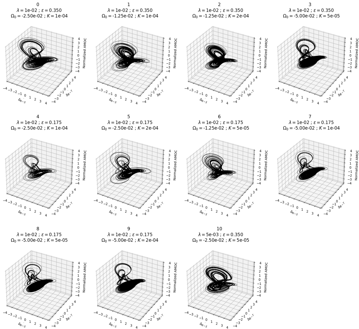
Figure 2. Chaotic trajectories in the phase space of the eleven perturbed versions of the 3-variable (normalized here) AMOC model (Sévelle and Fedorov 2014). The values of the perturbed parameters \lambda , \epsilon , \Omega_0 and K used to generate the eleven model versions are indicated in the title. The attractor labelled 0 (top left) corresponds to the model with the reference set of parameters.
