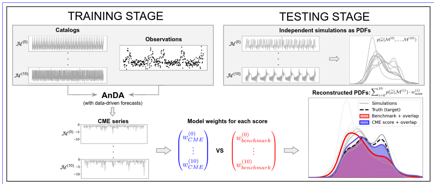
Figure 1. Schematic of the two-stages methodology for one experiment using 11 -models. Left panel: training stage performing AnDA with the 11 catalogs and a single set of observations leading to CME computation. Bottom center: from the CME-based score and benchmark score-model weights are obtained-calculated for two illustrative scores, one based on CME and another based on a benchmark method (blue and red, respectively). Right panel: by applying the weights to individual PDF of new model distributions-simulations (grey) -,are weighted following (8) to obtain a single-reconstructed distribution-PDF associated with each-score-is-obtained-both-competing-scores (blue and red)which-is-compared-to-the-truth-(dashed-black). The quality of the reconstruction-both-reconstructions is assessed using-a-distribution-by-measuring-the overlap (blue and red shadings) with the true PDF (dashed black line) which allows comparison of the performance of the two scores. Here, the CME score shows a higher overlap with the true distribution, highlighting a better reconstruction compared to the benchmark score.
