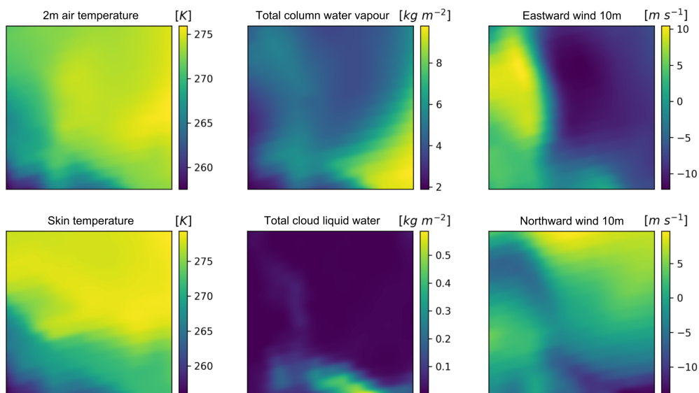
Figure 6. An example of the numerical weather prediction parameters including 2m air and skin temperature, total column water vapour and cloud liquid water, and East- and Northward wind 10m components for the scene depicted in Fig. 2 and in the same perspective as Fig. 3-5.
