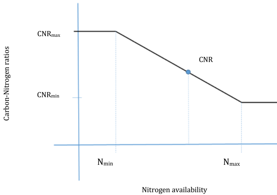
210 Figure 2. The relationship between soil nitrogen availability and plant carbon-nitrogen ratios.
