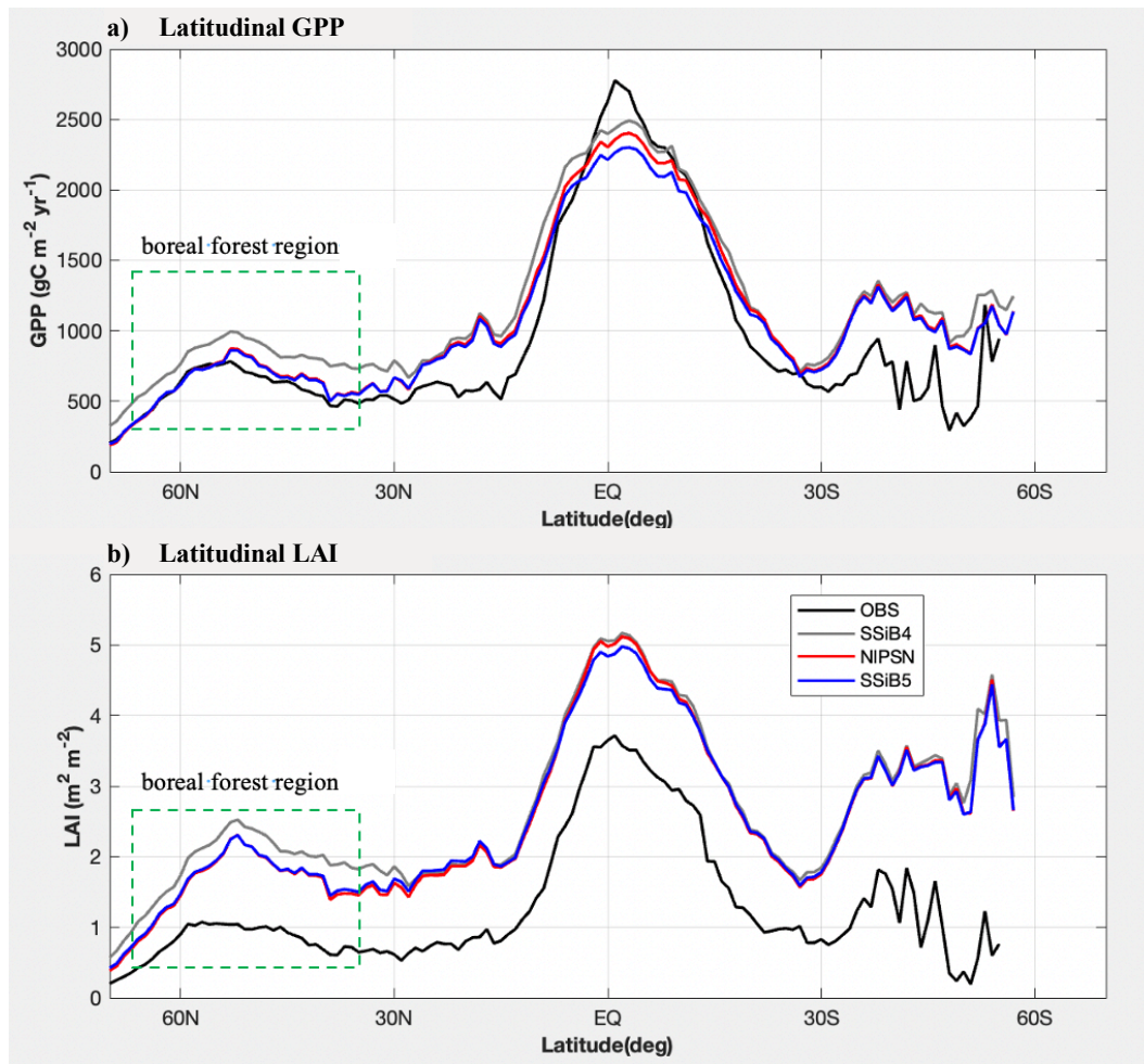
Figure 9. Intercomparisons of latitudinal LAI and GPP among OBS, SSiB4 (control), NIPSN (N limitation on photosynthesis only), and 515 SSiB5 (all N processes) over the period of 1982-2007.
