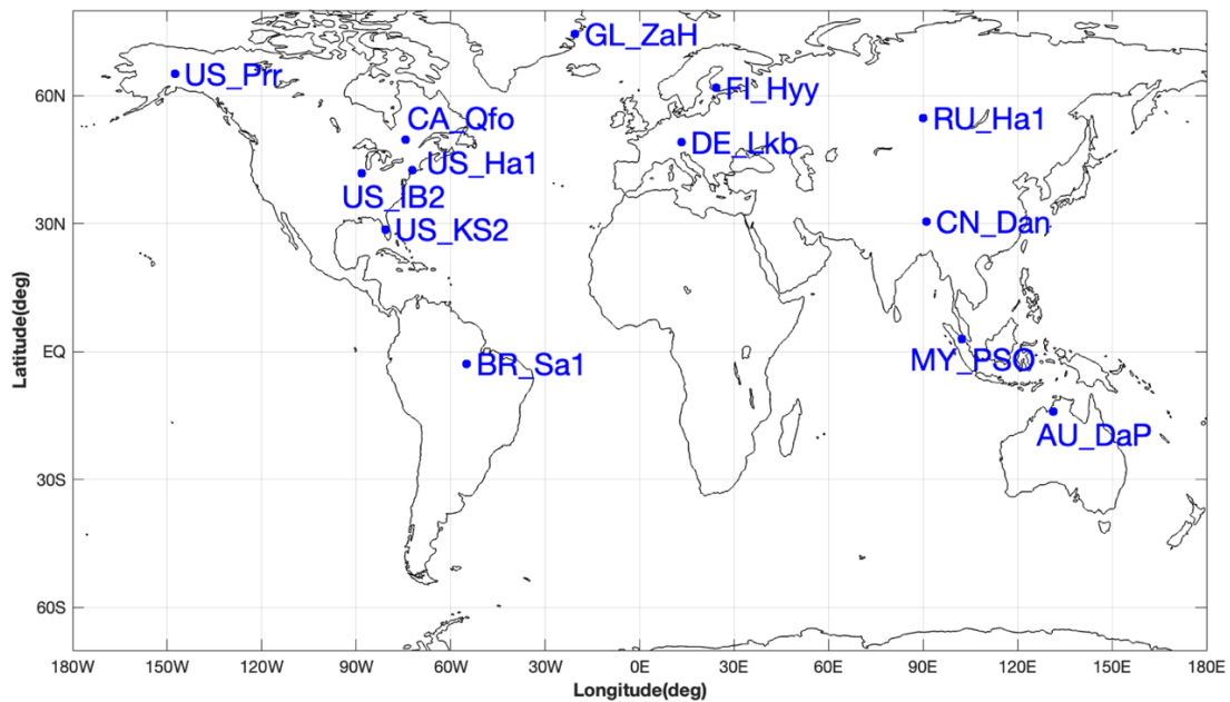
360 Figure 4. Geographical distribution of selected FLUXNET 2015 sites. The information on these FLUXNET sites is listed in Table 4.
