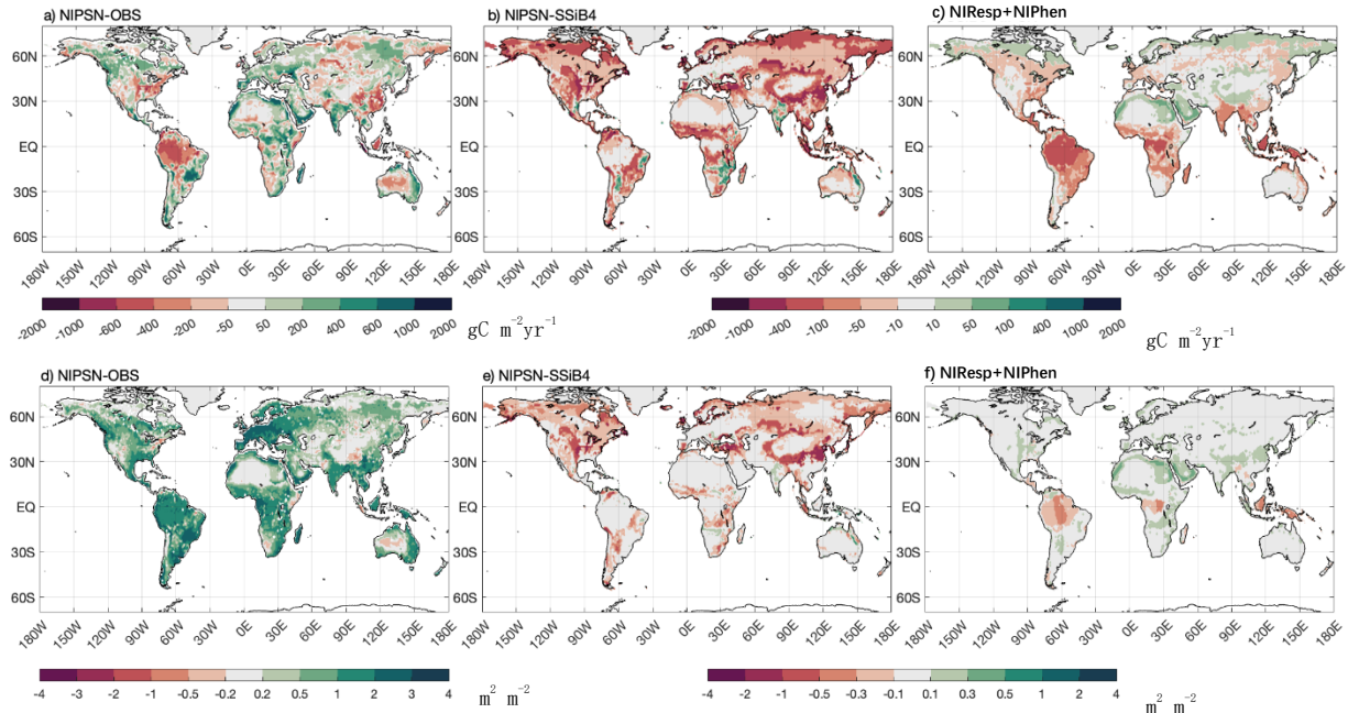
Figure 13. The 1982-2007 average gross primary production difference (a) NIPSN-OBS, (b) NIPSN-SSiB4, (c) NIResp+NIPhen, and leaf area index difference (d) NIPSN- OBS, (e) NIPSN- SSiB4, (f) NIResp+NIPhen
