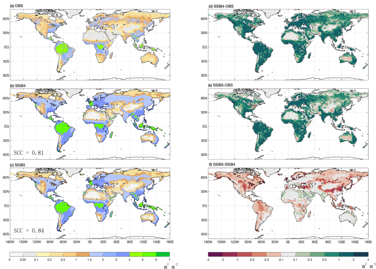
Figure 12. The 1982-2007 average LAI comparison for (a) GIMMS LAI (OBS), (b) SSiB4/TRIFFID (SSiB4), and (c) SSiB5/TRIFFID/DayCent/SOM (SSiB5) and the difference between (d) SSiB4-OBS, (e) SSiB5-OBS, and (f) SSiB5-SSiB4.
