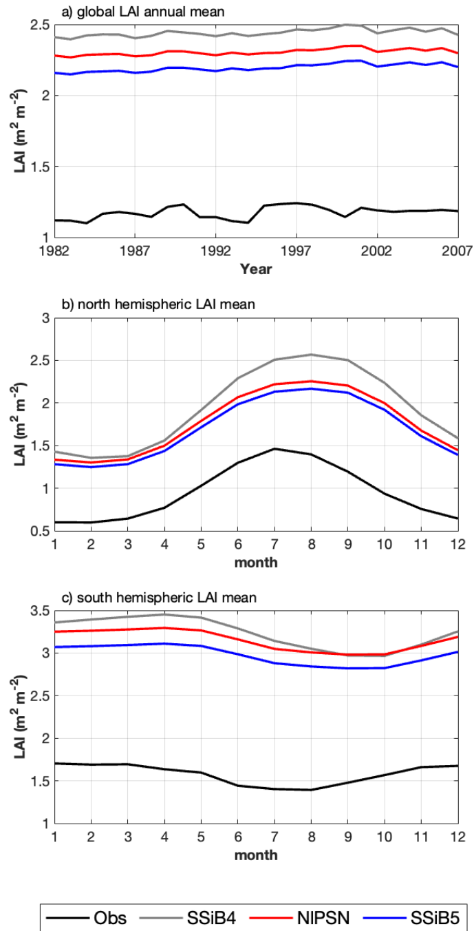
545 Figure 11. Intercomparisons of (a) global annual mean LAIs among OBS, SSiB4, NIPSN, and SSiB5; (b) and (c). Monthly mean LAIs averaged over the period of 1982-2007 for the Northern Hemisphere ( 0^\circ to 50^\circ\text{N} ) and Southern Hemisphere ( 60^\circ\text{S} to 0^\circ ). Note: The observed LAI is the GIMMS LAI.
