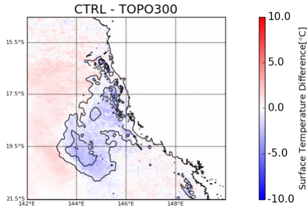
Figure R2: Differences of simulated surface temperature between CTRL and Topo300. Black contours show the topography from 500 to 1500 m with 250 m interval.
