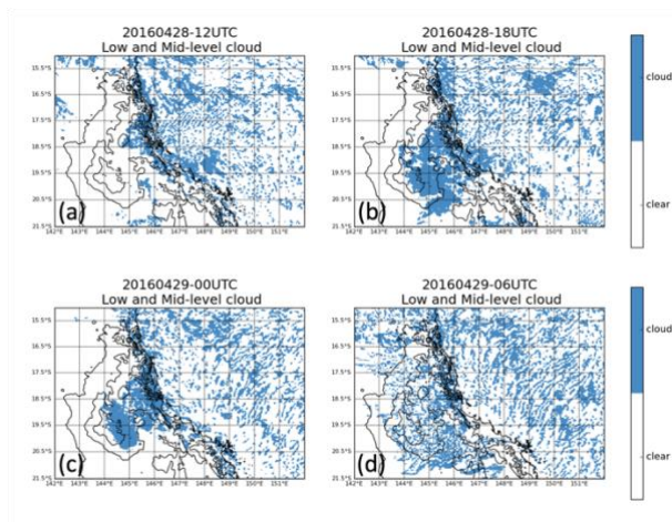
Figure R1: Examples of simulated cloud field from CTRL at (a) 12UTC 28, (b) 18UTC 28, (c) 00UTC 29, and (d) 06UTC 29 April 2016.
