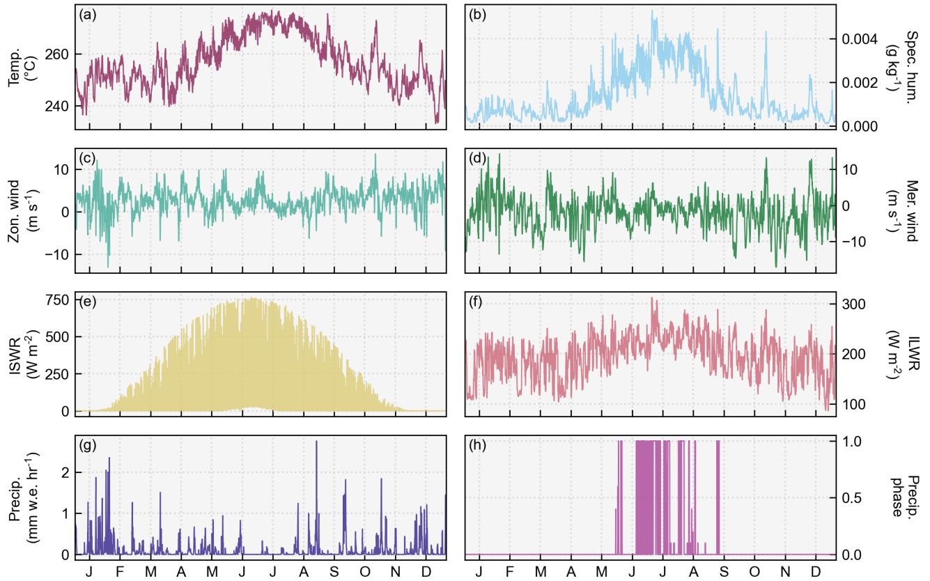
455 Figure A1: Example of one year (1991) of hourly unperturbed atmospheric forcing data for a single location (69.5°N, 27.5°W). (a) Air temperature, (b) specific humidity, (c) zonal wind, (d) meridional wind, (e) incoming shortwave radiation, (f) incoming longwave radiation, (g) precipitation, and (h) precipitation phase. The precipitation phase is a fractional value ranging from 0 to 1, where 0 is all solid precipitation and 1 is all liquid precipitation.
