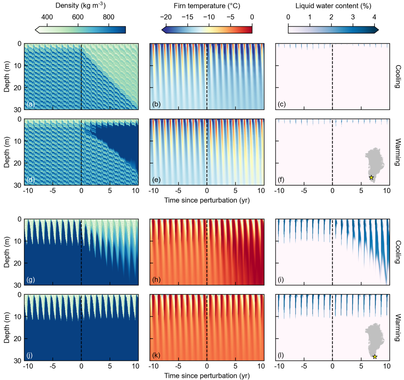
430 Figure 7: Time–depth plots showing firn properties (density, firn temperature, and liquid water content) for the upper 30 m of the firn column for the 10 yr before and after the temperature perturbation (vertical black dashed line) for two example locations. (a–f) Results from a grid cell in southwest Greenland as seen in Fig. 6e. (g–l) Results from a grid cell in southeast Greenland as seen in Fig. 6f. The responses to cooling are shown in panels a–c– and g–i, and the responses to warming are shown in panels d–f and j–l. Inset maps in panels (f) and (l) show each example’s location on the ice sheet as a yellow star.
