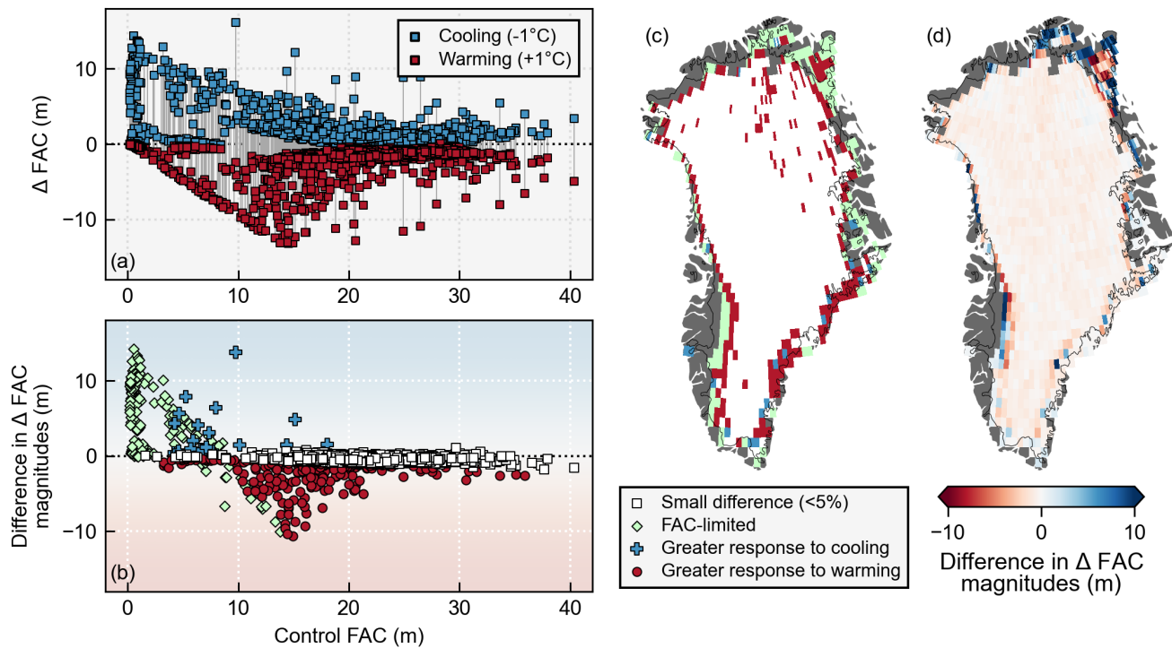
435 Figure 8: Types of firn air content (FAC) response relationships across the ice sheet. (a) The change in firn air content for each grid cell calculated as the final value minus the control mean as a function of the control mean firn air content. Blue markers indicate the effect of cooling and red indicate the effect of warming; gray vertical lines connect the warming and cooling responses from each grid cell. (b) The difference in the magnitudes of firn air content changes due to warming and cooling. The difference is calculated as the magnitude of the cooling change minus the magnitude of the warming change, such that positive values indicate a greater 440 response to cooling (blue background shading) and negative values indicate a greater response to warming (red background shading). The different marker shapes and colors differentiate the four types of responses shown in the legend to the right. (c) Locations of the different response types across the ice sheet. (d) The difference in magnitudes of firn air content change due to cooling and warming shown in map view. The thin black line in (c) and (d) represents the ice sheet outline.
