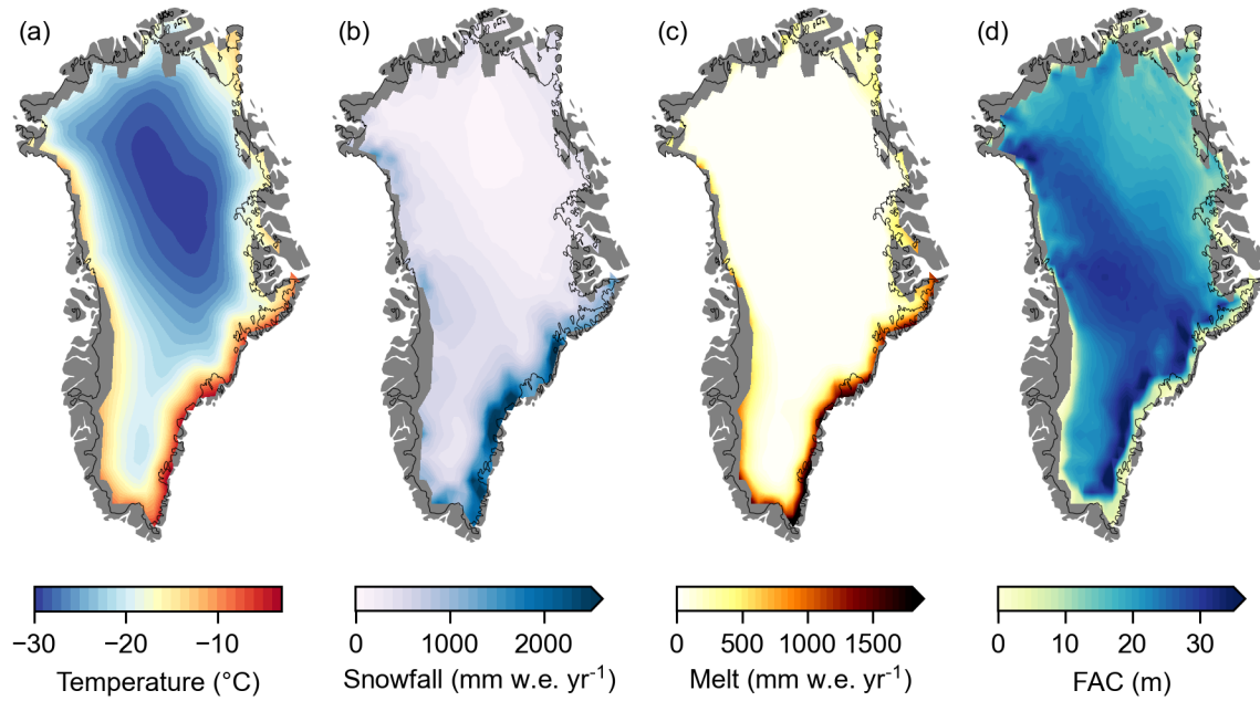
380 Figure 1: Greenland Ice Sheet mean annual (a) temperature, (b) snowfall, (c) melt, and (d) firn air content (FAC) from the 100-yr control climate (i.e., the 1991 climate) prior to the warming and cooling experiments. The thin black line represents the ice sheet outline. The data have been interpolated to more easily show spatial patterns. The original forcing resolution can be seen in Fig. 8.
