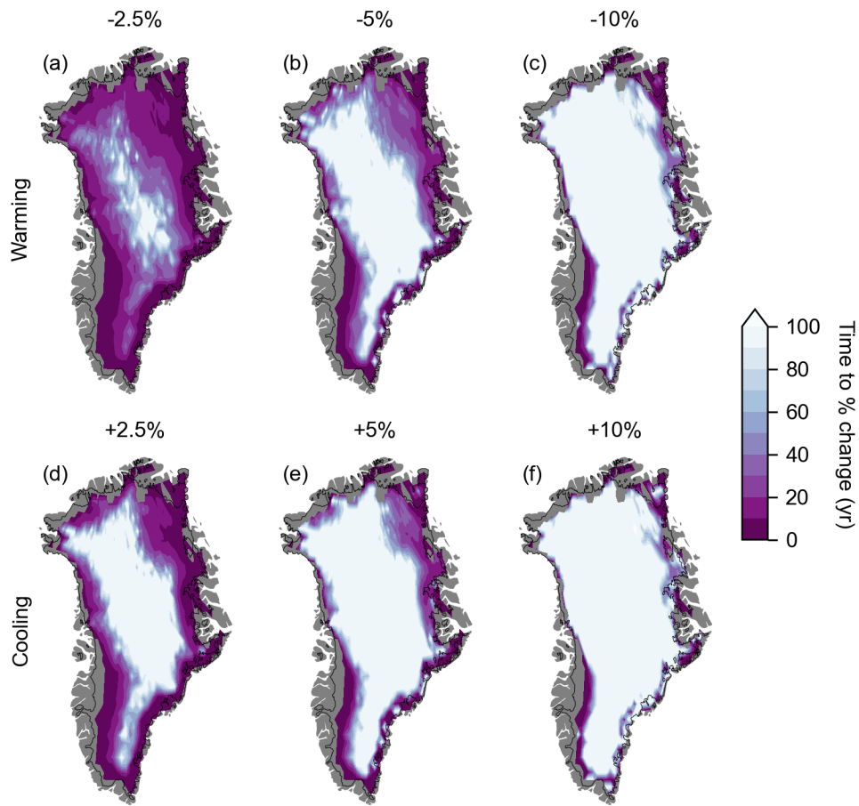
395 Figure 3: Elapsed time to reach a given percent change (shown above each panel) in firn air content following the control mean. Results are shown from both (a–c) warming by 1 °C, and (d–f) cooling by 1 °C. The lightest shading indicates that the given percent change has not been achieved within the 100-yr warming or cooling experiment, and thus the elapsed time is >100 yr. The thin black line represents the ice sheet outline. The data have been interpolated to more easily show spatial patterns. The original forcing resolution can be seen in Fig. 8.
