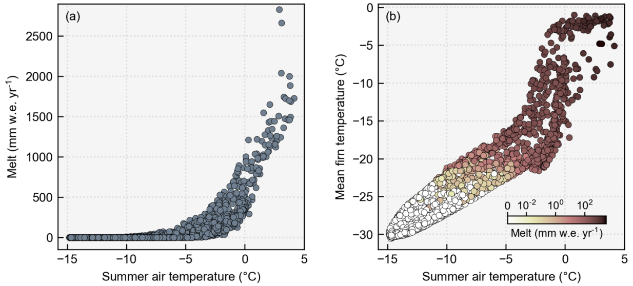
410 Figure 5: Control mean (a) melt and (b) firn temperature as functions of the control mean summer air temperature for all modeled locations. The color of the points in (b) represents the control mean melt.
