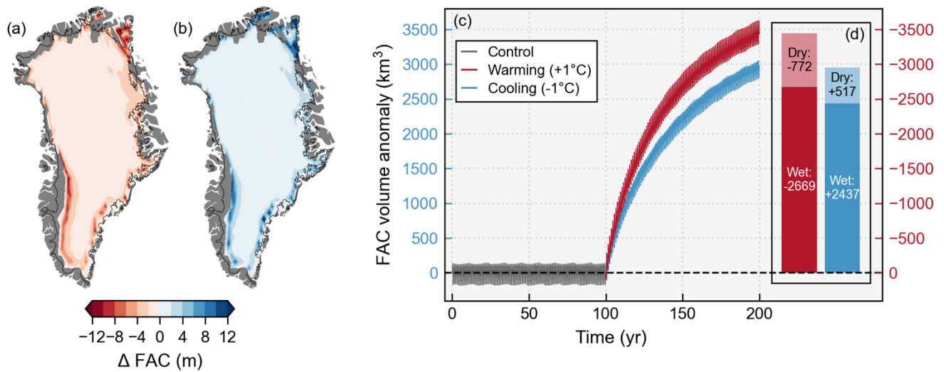
390 Figure 2: Change in firn air content (FAC) for the Greenland Ice Sheet calculated as the final firn air content minus the mean of the control conditions for (a) warming by 1 °C and (b) cooling by 1 °C. The thin black line represents the ice sheet outline. The data have been interpolated to more easily show spatial patterns. The original forcing resolution can be seen in Fig. 8. (c) Time series of the firn air content volume anomaly integrated over the full ice sheet for the control (gray line), warming (red line), and cooling (blue line) periods. The control period and cooling experiment use the positive values on the left y-axis and the warming experiment uses the negative values on the right y-axis. (d) Changes in spatially integrated firn air content in km 3 at the end of the experiments partitioned into wet firn (melt is present) and dry firn (melt is not present) areas for warming (red) and cooling (blue).
