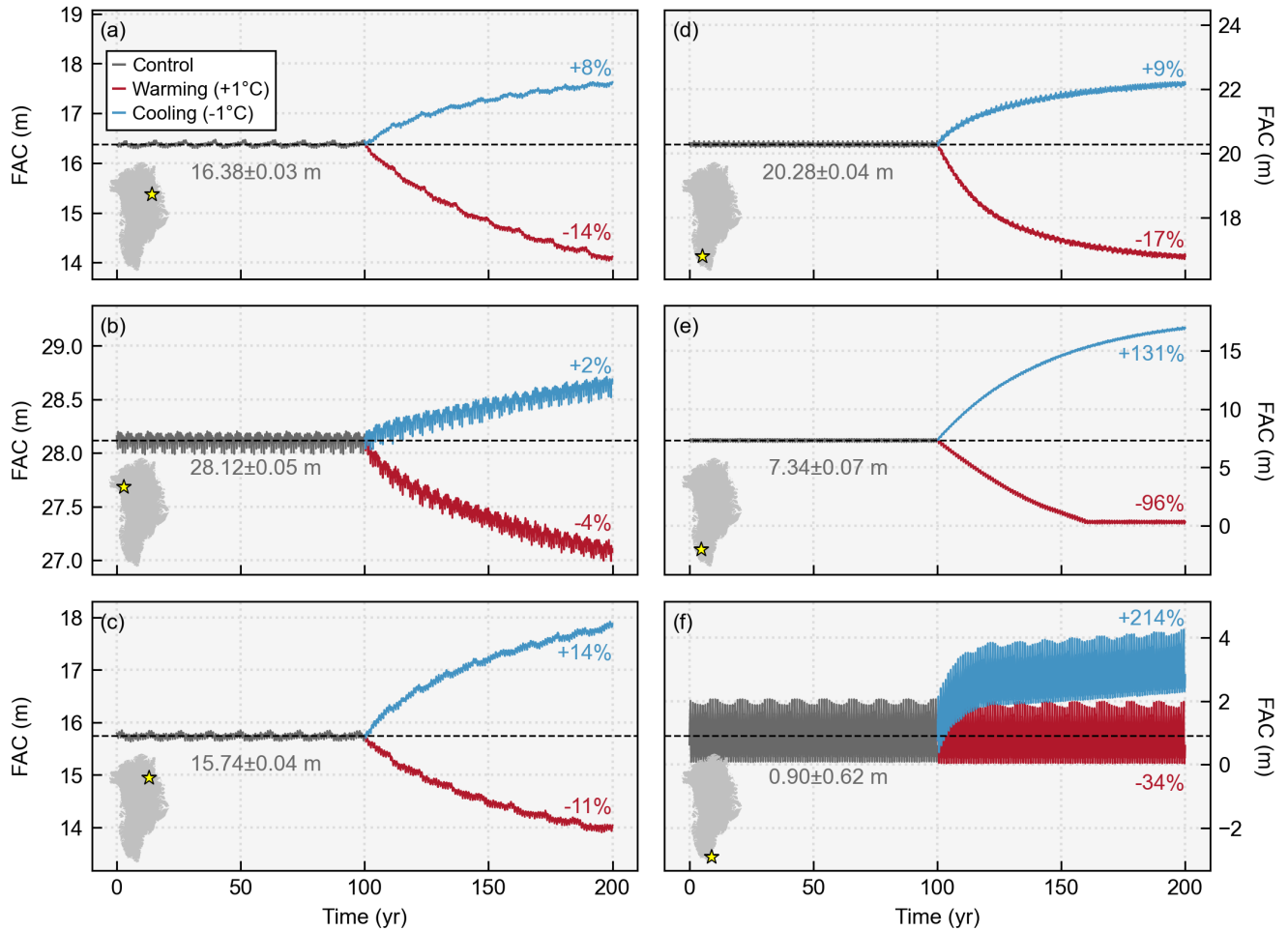
420 Figure 6: Firn air content (FAC) over time in the control period (gray line), warming experiment (red line), and cooling experiment (blue line) from six locations shown in the inset maps as yellow stars. Numbers in gray show the mean and standard deviation of the firn air content in the control period, and red and blue percentages show the total percent change due to warming and cooling, respectively. Note the different y-axis scales. Also note that the approximately decadal oscillations in the time series are a result of leap years affecting the 14-day model output frequency and are not real signals within the data.
