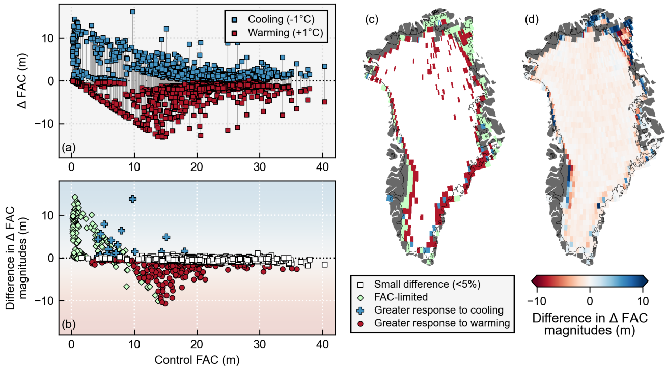
Figure 8: Types of firn air content (FAC) response relationships across the ice sheet. (a) The change in firn air content for each grid cell calculated as the final value minus the control mean as a function of the control mean firn air content. Blue markers indicate the effect of cooling and red indicate the effect of warming; gray vertical lines connect the warming and cooling responses from each grid cell. (b) The difference in the magnitudes of firn air content changes due to warming and cooling. The difference is calculated as the magnitude of the cooling change minus the magnitude of the warming change, such that positive values indicate a greater response to cooling (blue background shading) and negative values indicate a greater response to warming (red background shading). The different marker shapes and colors differentiate the four types of responses shown in the legend to the right. (c) Locations of the different response types across the ice sheet. (d) The difference in magnitudes of firn air content change due to cooling and warming shown in map view. The thin black line in (c) and (d) represents the ice sheet outline.
