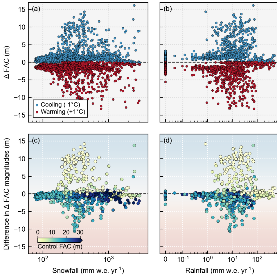
465 Figure A2: (a–b) The change in firn air content (FAC) for each grid cell calculated as the final value minus the control mean as a function of the control mean (a) snowfall and (b) rainfall. Blue markers indicate the effect of cooling and red indicate the effect of warming. (c–d) The difference in the magnitudes of firn air content changes due to warming and cooling. The difference is calculated as the magnitude of the cooling change minus the magnitude of the warming change, such that positive values indicate a greater response to cooling (blue background shading) and negative values indicate a greater response to warming (red background shading). The markers are colored by the control mean firn air content. Note the semi-logarithmic x-scales used in all panels.
