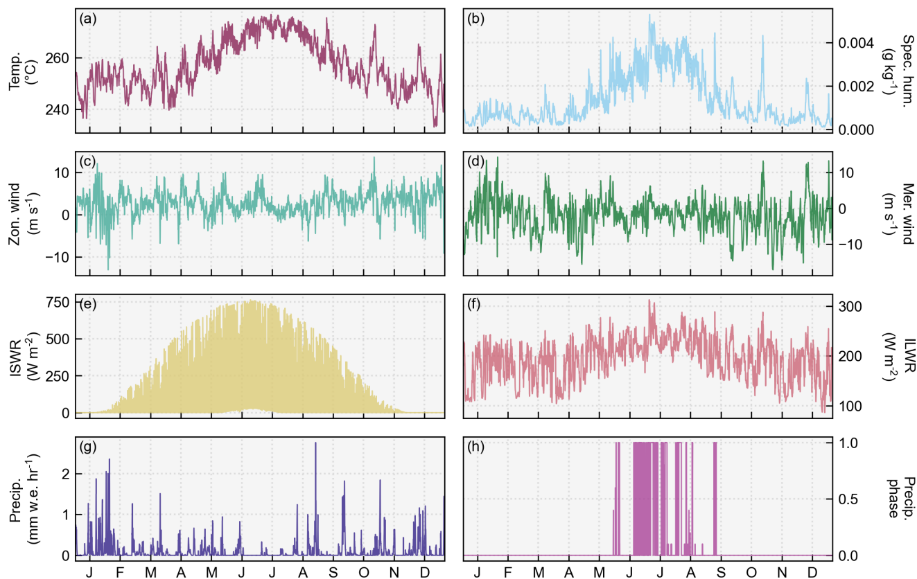
Figure A1: Example of one year (1991) of hourly unperturbed atmospheric forcing data for a single location ( 69.5^{\circ}\text{N} , 27.5^{\circ}\text{W} ). (a) Air temperature, (b) specific humidity, (c) zonal wind, (d) meridional wind, (e) incoming shortwave radiation, (f) incoming longwave radiation, (g) precipitation, and (h) precipitation phase. The precipitation phase is a fractional value ranging from 0 to 1, where 0 is all solid precipitation and 1 is all liquid precipitation.
