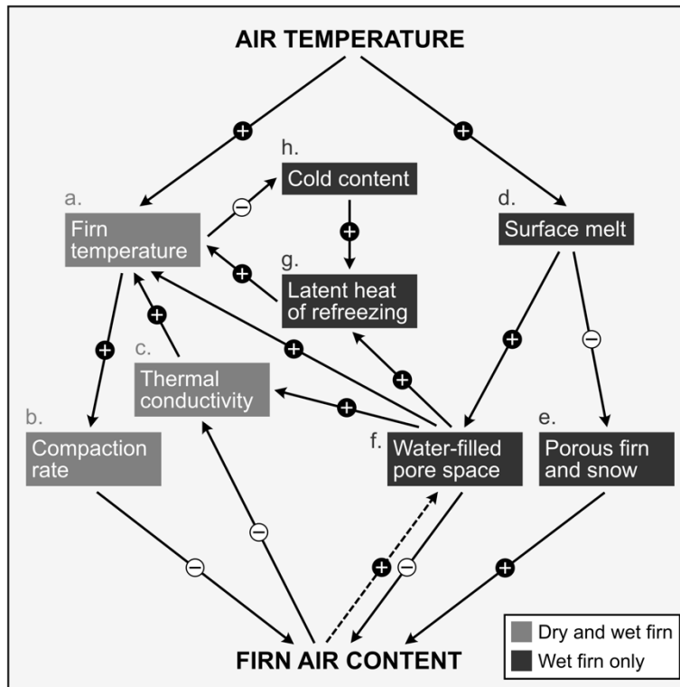
450 Figure 9: Schematic of air temperature-driven interactions within the firn layer. Arrows with plus signs indicate a direct relationship while arrows with minus signs indicate an inverse relationship. The dashed arrow represents a relationship that only exists where runoff occurs and firn air content increases. Dark gray boxes show processes occurring in the presence of melt (i.e., in wet firn only) and light gray boxes show processes occurring in both dry and wet firn.
