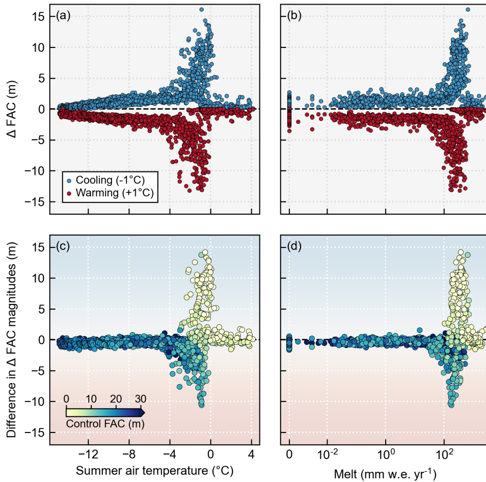
405 Figure 4: (a–b) The change in firn air content (FAC) for each grid cell calculated as the final value minus the control mean as a function of the control mean (a) summer air temperature and (b) melt. Blue markers indicate the effect of cooling and red indicate the effect of warming. (c–d) The difference in the magnitudes of firn air content changes due to warming and cooling. The difference is calculated as the magnitude of the cooling change minus the magnitude of the warming change, such that positive values indicate a greater response to cooling (blue background shading) and negative values indicate a greater response to warming (red background shading). The markers are colored by the control mean firn air content. Note the semi-logarithmic x-scales used for melt in (b) and (d).
