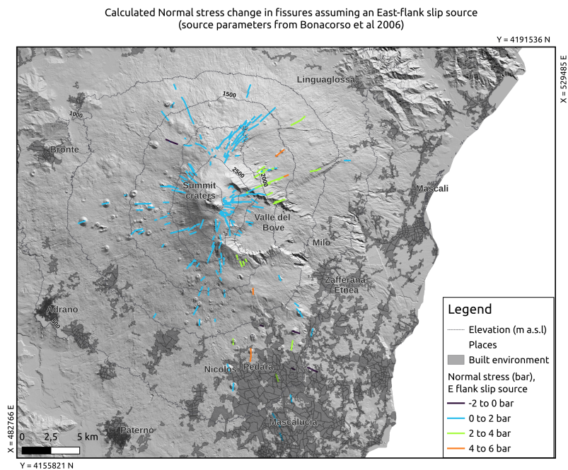
Figure 3. Normal stress change on fissures in the catalog, when an Eastward flank-slip source of deformation at depth is placed, as in Bonaccorso et al (2006) (positive values indicate unclamping; Poisson ratio 0.25; Young's modulus 8.0 \times 10^5 bar). The location and extent of the built environment is shown in dark gray shaded areas.
