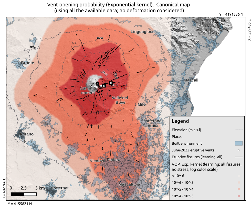
Figure 5. Map of the probability (in Log-scale colours in Log scale ) of flank fissure opening at Etna, based on the data 4000BP-2000 CE to present (black solid lines), in what we call canonical model. The location of the vents active in June 2022 is indicated by white points and labelled as A, B and C. The location and extent of the built environment is shown as shaded pale blue areas, and altitude contour lines are shown in dashed black lines.
