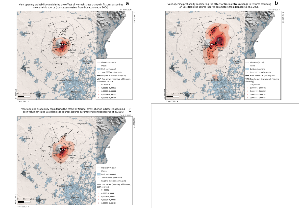
Figure A5. Same as Figure 7 but in linear scale: maps of the probability (in linear scale colours in linear scale) of lateral fissure opening at Etna, based on the data 4000BP-2000 CE to present (black solid lines), considering the unclamping stress in the input fissures. The different panels a, b and c correspond to, respectively, information from the volumetric, flank-slip and both sources. In each panel, the location of the vents active in June 2022 is indicated by white points and labelled as A, B and C. The location and extent of the built environment is shown as shaded pale blue areas. In white solid lines we show the oldest fissures (4000BP-2000 CE to 1599 CE) not used in these maps.
