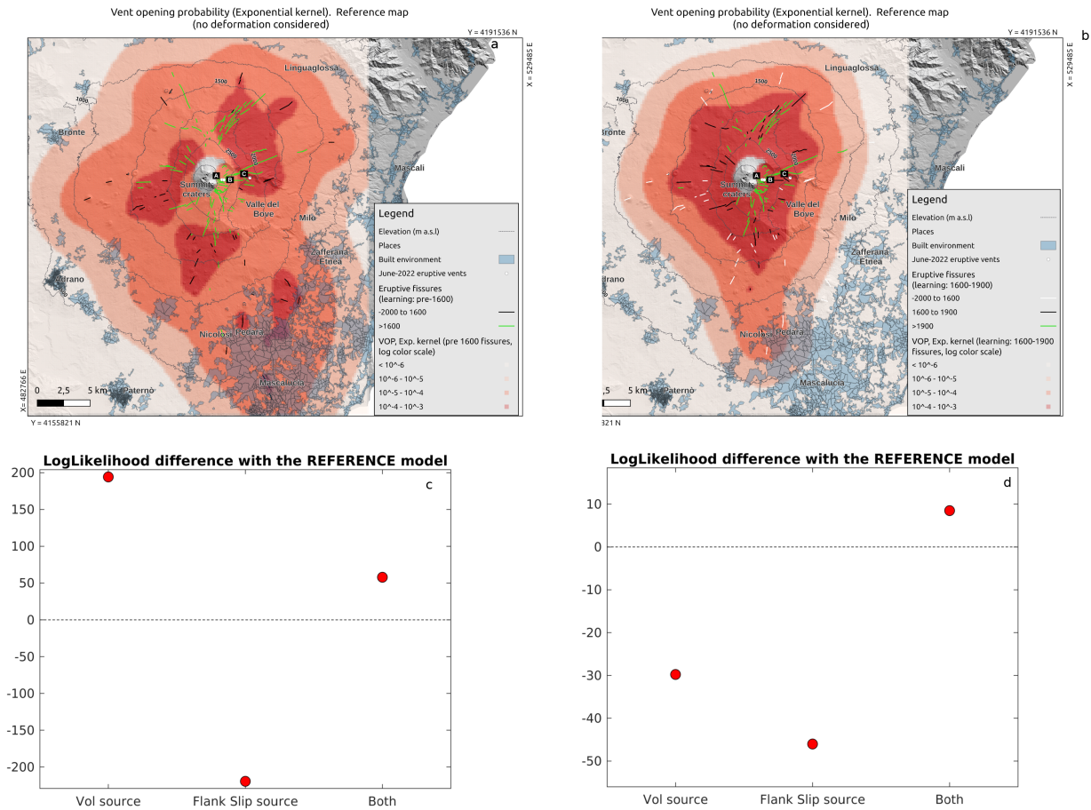
Figure 4. Panels a-b: Spatial probability (in Log-scale colours in Log scale) distribution of flank opening under the reference model for the training period 4000BP-2000 CE to 1600 CE (a) and 1600 CE to 1900 CE (b). In black and green the training and testing (i.e., respectively post 1600 CE and post 1900 CE for a and b) fissures. In panel b, in white solid lines we show the fissures older than 1600 CE, which are not used in the case of panel b. Panels c-d: Log-Likelihood difference between the models weighted with the three deformation sources explored (Volumetric, Flank Slip and Both) and the reference model of panels a and b, respectively. Positive differences (values above the dashed line) indicate a best performance on the testing data with respect of the reference model.
