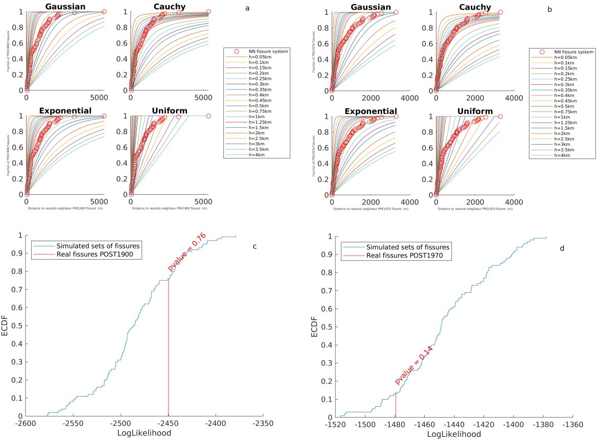
Figure A1. Panels a-b: Empirical Cumulative Density Functions (ECDF) of the distance to the nearest system of fissures (red dots) for the training period 4000BP-2000 CE to 1900 CE (a) and 4000BP-2000 CE to 1970 CE (b). The curves represent the theoretical cumulative for different kernel functions (Gaussian, Cauchy, Exponential and Uniform) and smoothing parameter h , as in legends on the right for each case. Panels c-d: ECDF of the Log-Likelihood of synthetic catalogs of synthetic fissures (black line) under the reference model for the training period (d) 4000BP-2000 CE to 1900 CE (Exponential kernel, h=1000\text{m} ) and (d) 4000BP-2000 CE to 1970 CE (Exponential kernel, h=500\text{m} ). In red we point the value of the Log-Likelihood achieved by the reference model on the real testing data, providing the p -value in percent.
