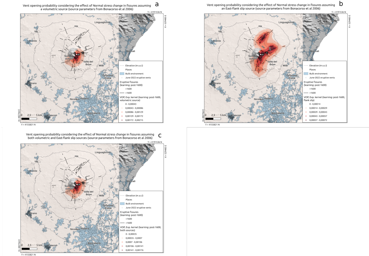
Figure A6. Same as Figure 8 but in linear scale: maps of the probability (in linear scale colours in linear scale) of lateral fissure opening at Etna, based on the data 1600 CE to present (black solid lines), considering the unclamping stress in the input fissures. The different panels a, b and c correspond to, respectively, information from the volumetric, flank-slip and both sources. In each panel, the location of the vents active in June 2022 is indicated by white points and labelled as A, B and C. The location and extent of the built environment is shown as shaded pale blue areas. In white solid lines we show the oldest fissures (4000BP-2000 CE to 1599 CE) not used in these maps.
