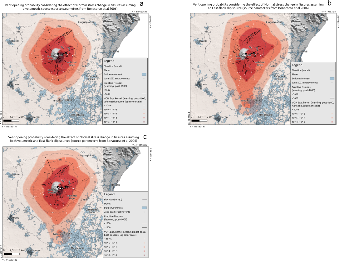
Figure 8. Sensitivity analysis: maps of the probability ( in Log scale colours in Log scale) of flank fissure opening at Etna, based on the data 1600 CE to present (black solid lines), considering the unclamping stress in the input fissures. The different panels a, b and c correspond to, respectively, information from the volumetric, flank-slip and both sources. In each panel, the location of the vents active in June 2022 is indicated by white points and labelled as A, B and C. The location and extent of the built environment is shown as shaded pale blue areas. In white solid lines we show the oldest fissures ( 4000BP-2000 CE to 1599 CE ) not used in these maps.
