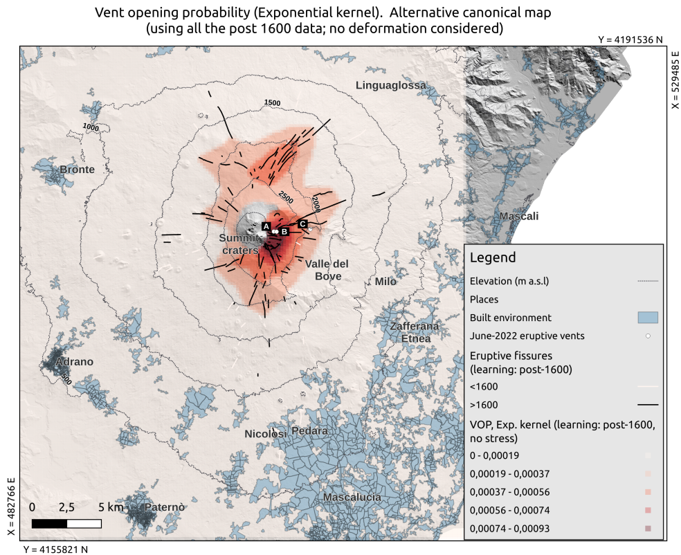
Figure A4. Same as Figure 6 but in linear scale: map of the probability ( in linear scale colours in linear scale ) of flank fissure opening at Etna, based on a shorter time window for input data (1600 CE to present, black solid lines). The location of the vents active in June 2022 is indicated by white points and labelled as A, B and C. The location and extent of the built environment is shown as shaded pale blue areas, and altitude contour lines are shown in dashed black lines.
