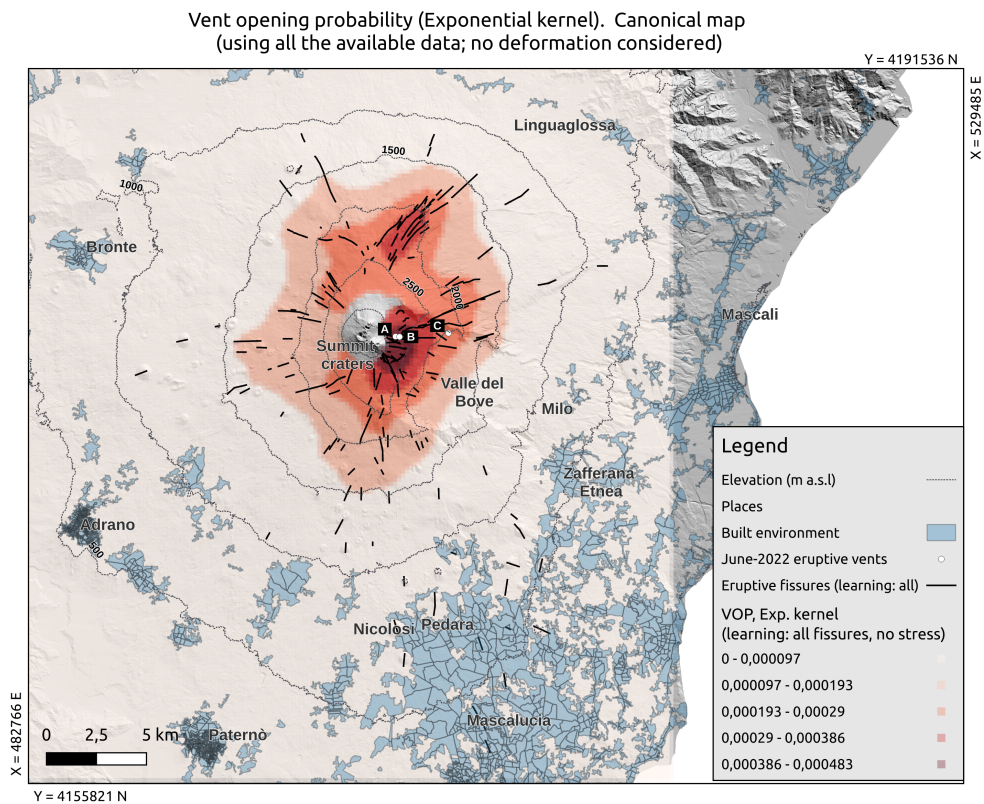
Figure A3. Same as Figure 5 but in linear scale: map of the probability ( in linear scale colours in linear scale ) of flank fissure opening at Etna, based on the data 4000BP-2000 CE to present (black solid lines), in what we call canonical model. The location of the vents active in June 2022 is indicated by white points and labelled as A, B and C. The location and extent of the built environment is shown as shaded pale blue areas, and altitude contour lines are shown in dashed black lines.
