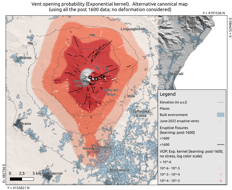
Figure 6. Result of the sensitivity analysis: map of the probability ( in Log-scale colours in Log scale ) of flank fissure opening at Etna, based on on a shorter time window for input data (1600 CE to present, black solid lines). The location of the vents active in June 2022 is indicated by white points and labelled as A, B and C. The location and extent of the built environment is shown as shaded pale blue areas, and altitude contour lines are shown in dashed black lines. In white solid lines we show the oldest fissures ( 4000BP-2000 CE to 1599 CE ) not used in these maps.
