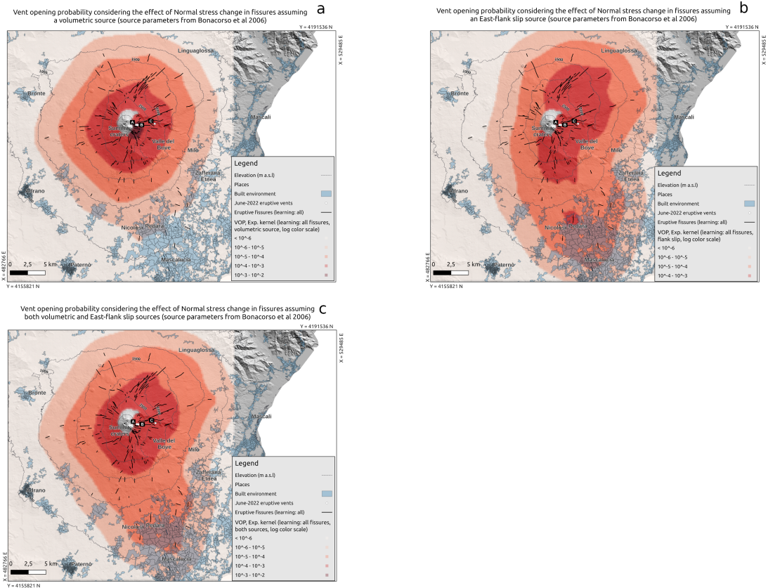
Figure 7. Sensitivity analysis: maps of the probability ( in Log-scale colours in Log scale ) of flank fissure opening at Etna, based on the data 4000BP-2000 CE to present (black solid lines), considering the unclamping stress in the input fissures. The different panels a, b and c correspond to, respectively, information from the volumetric, flank-slip and both sources. In each panel, the location of the vents active in June 2022 is indicated by white points and labelled as A, B and C. The location and extent of the built environment is shown as shaded pale blue areas.
