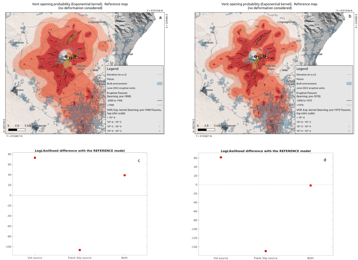
Figure A2. Panels a-b: Spatial probability (in Log-scale colours in Log scale ) distribution of flank opening under the reference model for the training period 4000BP-2000 CE to 1900 CE (a) and 4000BP-2000 CE to 1970 CE (b). In black and green the training and testing (i.e., respectively post 1900 CE and post 1970 CE for a and b) fissures. Panels c-d: Log-Likelihood difference between the models weighted with the three deformation sources explored (Volumetric, Flank Slip and Both) and the reference model of panels a and b, respectively. Positive differences (values above the dashed line) indicate a best performance on the testing data with respect of the reference model.
