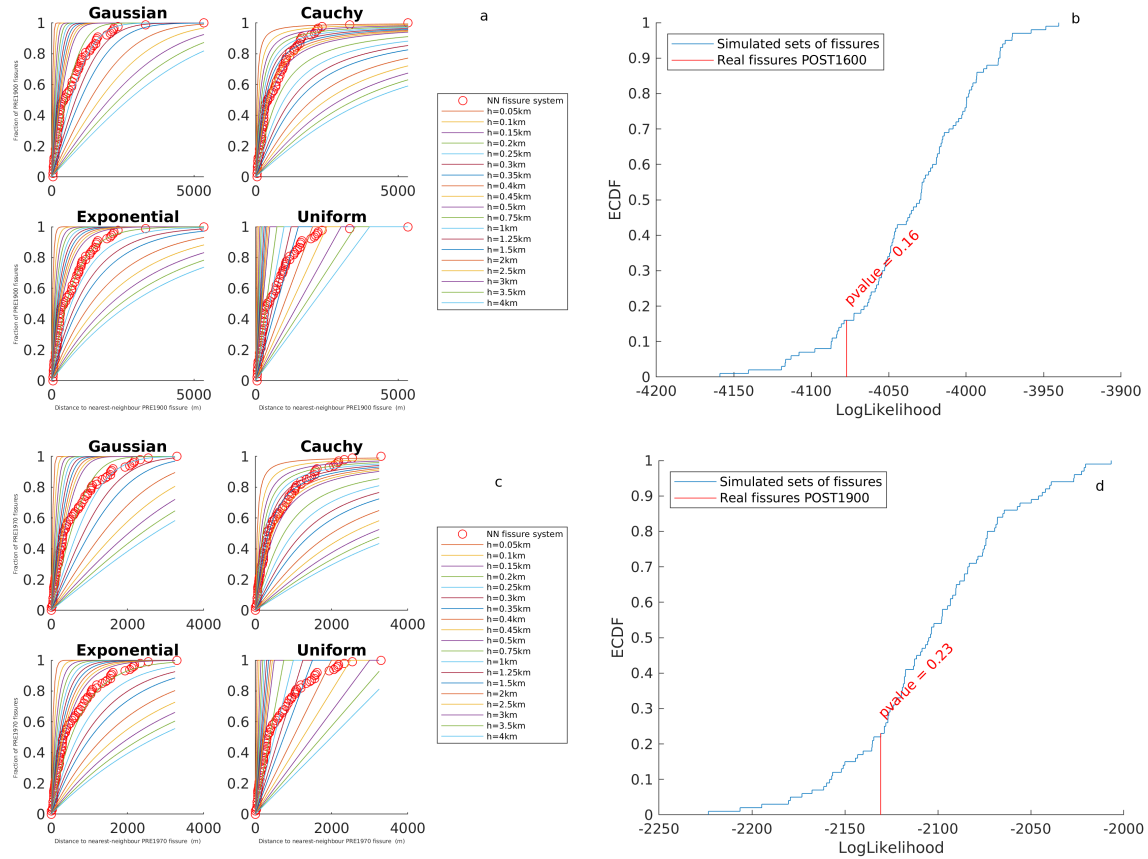
Figure 3. Panels a and c: Empirical Cumulative Density Functions (ECDF) of the distance to the nearest system of fissures (red dots) for the training period 4000BP-2000 CE to 1600 CE (a) and 1600 CE to 1900 CE (c). The curves represent the theoretical cumulative for different kernel functions (Gaussian, Cauchy, Exponential and Uniform) and smoothing parameter h , as in legends on the right for each case. Panels b and d: ECDF of the Log-Likelihood of synthetic catalogs of synthetic fissures (black line) under the reference model for the training period (b) 4000BP-2000 CE to 1600 CE (Exponential kernel, h=1250m ) and (d) 1600 CE to 1900 CE (Exponential kernel, h=1000m ). In red we point the value of the Log-Likelihood achieved by the reference model on the real testing data, providing the p -value in percent.
