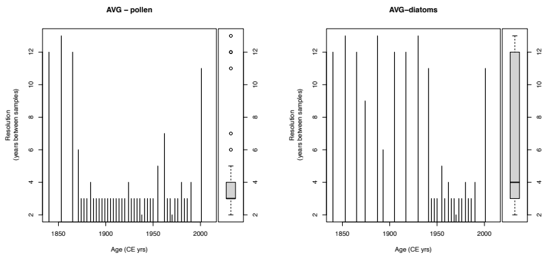
215 Figure A1: Inter-sample distance for the pollen (left) and the diatom records (right) from the sediments of Lago Grande di Avigliana (Finsinger et al., 2006).
