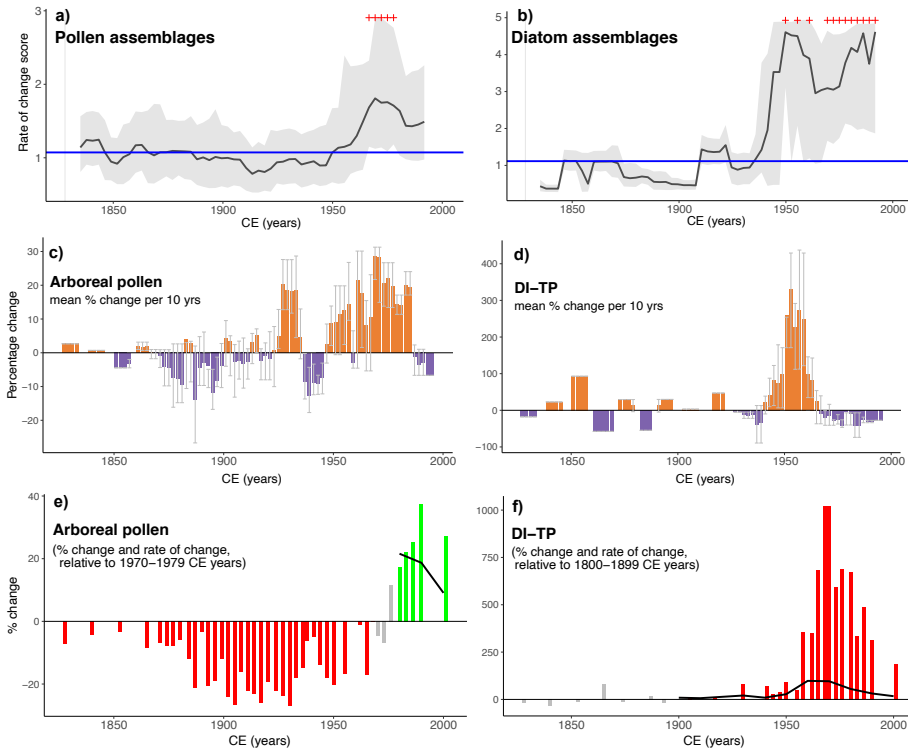
130 Figure 3: Comparison between rates of palaeoecological change based on (a) the pollen and (b) the diatom assemblages from 135 sediments of Lago Grande di Avigliana, and (c-f) the trends of palaeoecological indicators for the terrestrial and aquatic ecosystems (arboreal pollen percentages indicative of tree cover and diatom-inferred total phosphorous concentration (DI-TP), respectively) for the past c. 150 years. The panels in the middle (c-d) document how quickly and in which direction the palaeoecological indicators changed as the average decadal rate of percentage change (coloured bars: mean values; whiskers: first and third quartiles). The bottom panels (e-f) show how much of the indicator was present after (and if applicable also before) the reference period (grey bars), as well as how quickly and in which direction the palaeoecological indicators shifted relative to the reference period (black continuous line). In panels e) and f), the bars are colour-coded based on whether positive changes relative to the average reference level are desired (green) or undesired (red).
