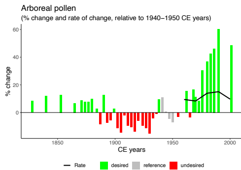
240 Figure A2: Percentage change (green and red bars) and per-decade rate of percentage change (black line) relative to 1940-1950 CE of arboreal pollen (grey bars), and thus by inference of tree cover.
