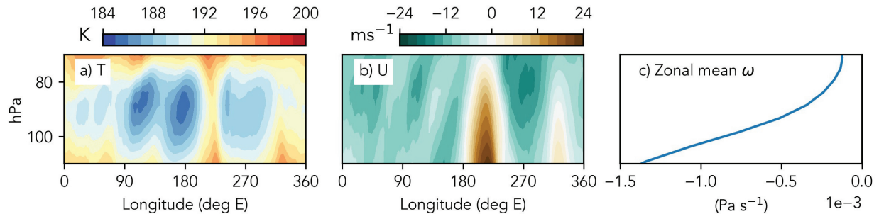
Figure 1. Meridional mean ( 10^\circ S to 10^\circ N) ERA5 tropical tropopause layer (a) temperatures, (b) zonal winds, and zonal mean vertical velocity for January 20–29, 2008. Note that positive zonal wind is eastward and negative vertical wind is upward.
