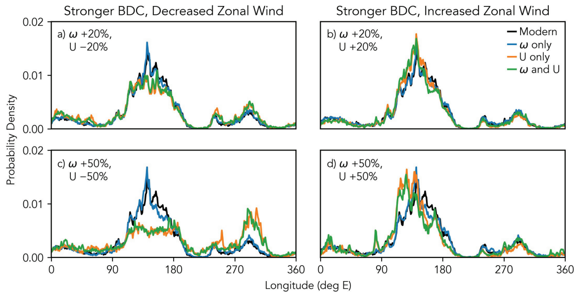
Figure 4. Probability density functions of trajectory cold point longitudes for DJF 2008 for the four altered transport scenarios: a) BDC accelerated by 20% and WE-Walker Circulation decelerated by 20%, b) BDC accelerated by 20% and WE-Walker Circulation accelerated by 20%, c) BDC accelerated by 50% and WE-Walker Circulation decelerated by 50%, d) BDC accelerated by 50% and WE-Walker Circulation accelerated by 50%. Figs. S4 and S5 and S6 show plots for DJF 2007 and 2009.
