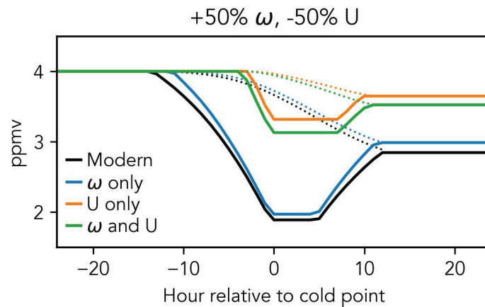
Figure 6. The water vapor concentration (solid lines) and the total water content (vapor + ice; dotted lines) for trajectories with a BDC accelerated by 50% and/or a WC-Walker Circulation decelerated by 50% based on the temperatures in Fig. 5c, with ice nucleation occurring at an ice saturation ratio of 1.6, sublimation occurring at an ice saturation ratio of 0.95, and rehydration limited by ice sedimentation following the cold point.
