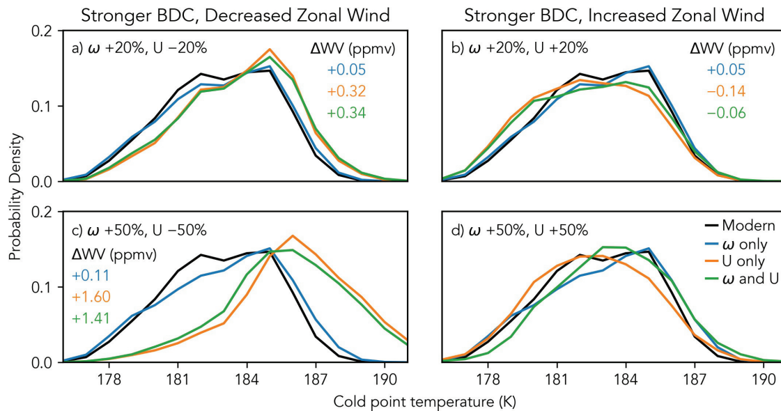
Figure 3. Probability density functions of trajectory cold point temperatures for DJF 2008 for the four altered transport scenarios: a) BDC accelerated by 20% and WC Walker Circulation decelerated by 20%, b) BDC accelerated by 20% and WC Walker Circulation accelerated by 20%, c) BDC accelerated by 50% and WC Walker Circulation decelerated by 50%, d) BDC accelerated by 50% and WC Walker Circulation accelerated by 50%. The corresponding increase in water vapor based on Clausius-Clapeyron scaling is indicated for panel in panels a, which represents b, and c; we omit these values in panel d due to the most likely future scenario-based impact of dispersion on model projections those trajectories. Figs. S2 and S3 and S4 show plots for DJF 2007 and 2009.
