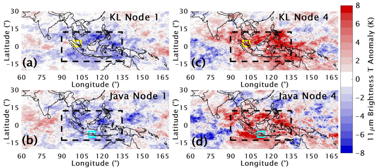
525 Figure 3: Composite anomalies from daily climatology (computed for 1991-2020) of GridSat-B1 11 μm brightness temperatures that correspond to the dates of the SOM node member ozonesonde profiles shown on Figure 2. The yellow, cyan, and black dashed boxes highlight the same regions as in Figure 1.
