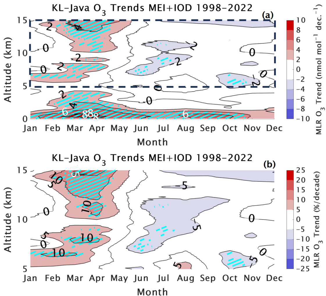
535 Figure 6: 1998-2022 monthly multiple linear regression (MLR) model ozone trends for the merged Kuala Lumpur/Watukosek (KL-Java) ozonesonde data in \text{nmol mol}^{-1} (a) and percent (b) per decade. Panel (a) includes the lowest 5 km, but our focus is on 5-15 km altitudes as indicated by the black dashed box on (a) and shown in (b). Cyan hatching indicates trends beyond the 95% confidence interval (i.e., historically referred to as statistically significant ).
