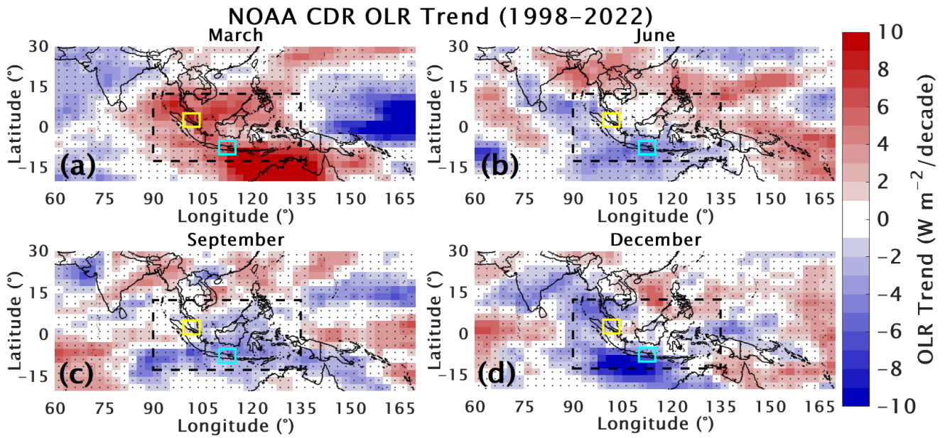
Figure 8: The same as shown in Figure 7, but for NOAA Climate Data Record (CDR) Outgoing Longwave Radiation (OLR) in Watts per square meter per decade.
