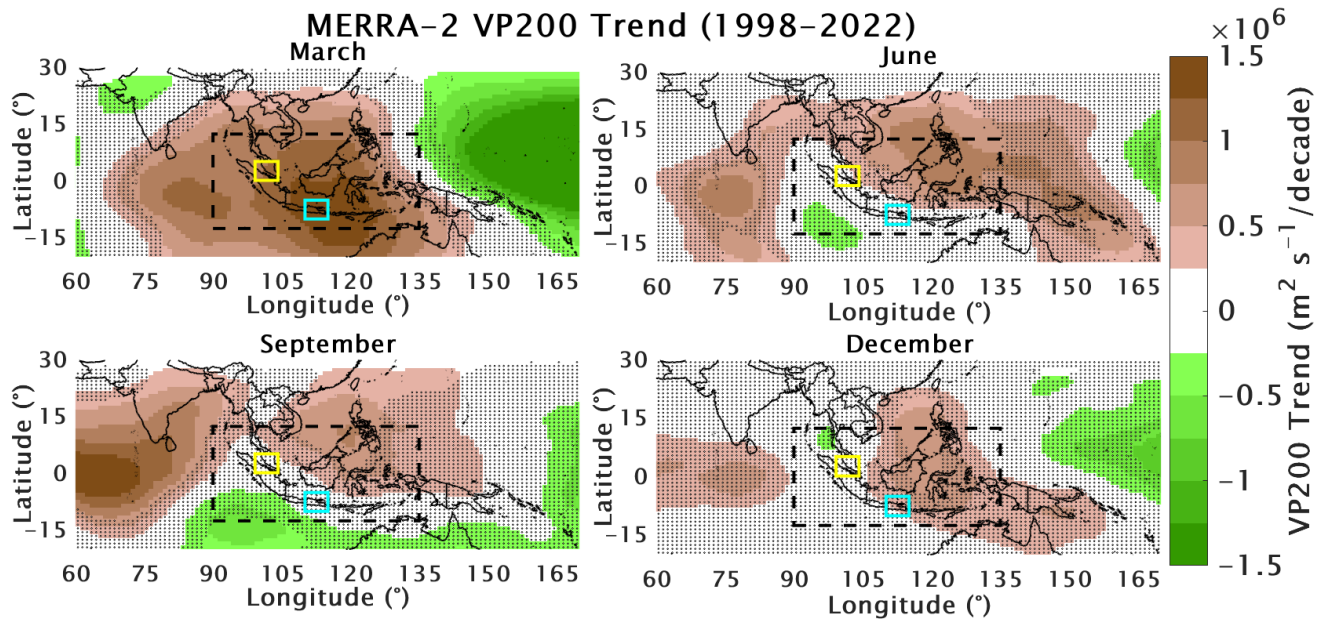
550 Figure 9: The same as shown in Figures 7 and 8, but for MERRA-2 velocity potential at 200 hPa (VP200) in meters squared per second per decade.
