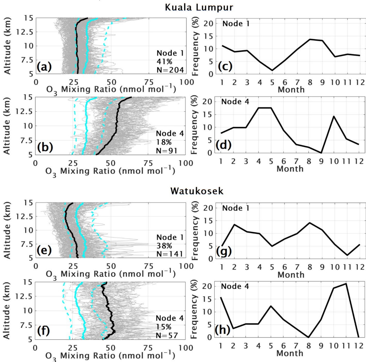
Figure 2: The four left panels show ozone mixing ratio SOM output for Kuala Lumpur (a, b) and Watukosek (e, f). The first (low ozone) and fourth (high ozone) nodes are shown for both SHADOZ stations. Grey profiles indicate all members of the respective nodes, with thick black lines showing node mean profiles, and cyan thick and dashed lines showing the average, 20 th , and 80 th percentile ozone for all profiles from the station. Text in each panel indicates the percent membership and total number of profiles for each node. The right four panels are the percent frequency according to month of the member profiles shown to their left for Kuala Lumpur (c, d) and Watukosek (g, h).
