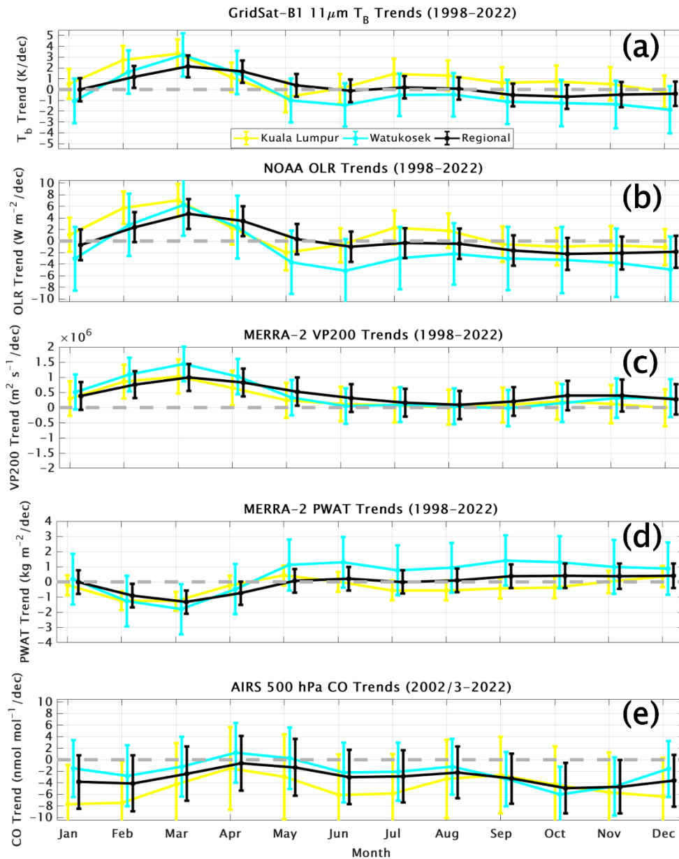
Figure 12: Monthly average trends with 95% confidence interval (error bars) for the three regions highlighted on the maps of previous Figures (yellow = Kuala Lumpur; cyan = Watukosek; black = larger region). The monthly trends are presented for GridSat-B1 11 \mu\text{m} T_b (a), NOAA OLR (b), MERRA-2 VP200 (c), MERRA-2 PWAT (d), and AIRS 500 hPa CO (e). All trends are for 1998–2022, except for AIRS CO (e) for which data are only available since September 2002.
