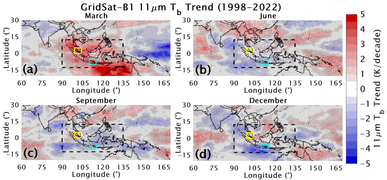
Figure 7: 1998–2022 MLR trends of GridSat-B1 11\ \mu\text{m} brightness temperature in Kelvin per decade for March (a), June (b), September (c), and December (d). The yellow, cyan, and black dashed boxes highlight the same regions as in Figure 1. Stippling indicates trends within the 95% confidence interval (i.e., historically referred to as statistically insignificant ).
