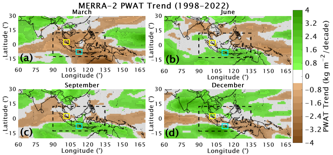
555 Figure 10: The same as shown in Figures 7-9, but for MERRA-2 precipitable water (PWAT) in kilograms per square meter per decade.
