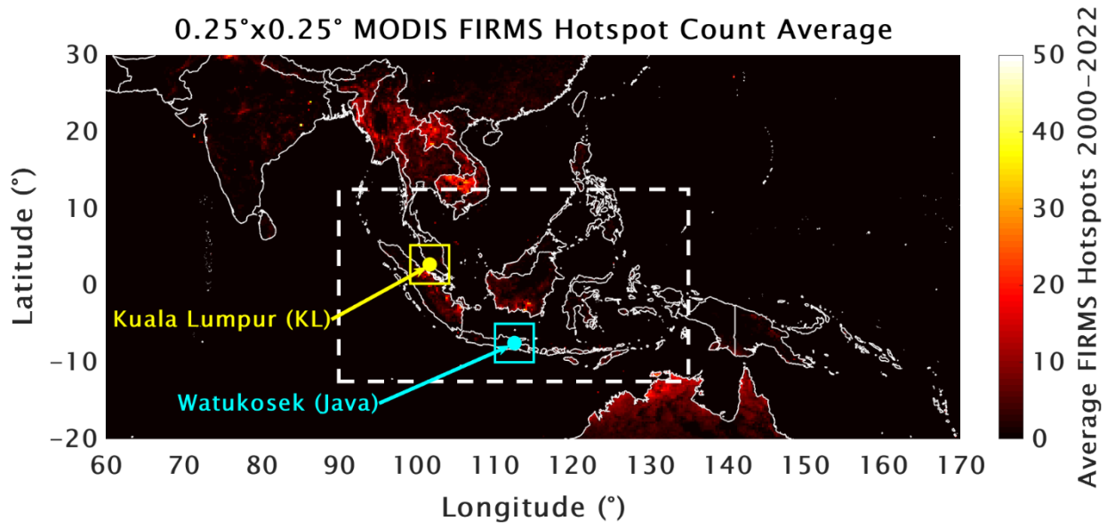
510 Figure 1: Map of the study region including average monthly Fire Information for Resource Management System (FIRMS) fire hotspot count from MODIS on the Terra and Aqua satellites for 2000-2022. The boxes indicate specific regions for which monthly trends will later be examined in greater detail. These include Kuala Lumpur (KL; yellow), Watukosek (Java; cyan), and the larger area outlined by the white dashed box.
