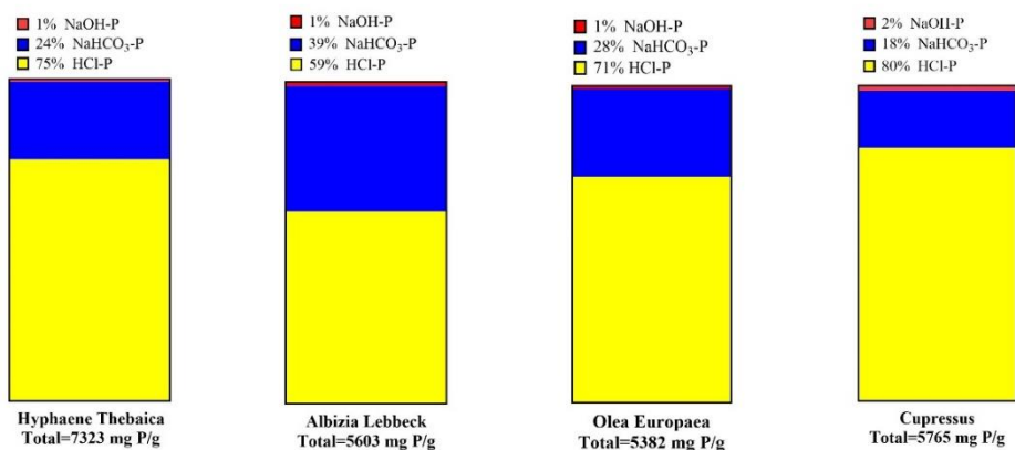
265 Figure 1: The fractionation of P in fire ash particles. Yellow color represents P fraction released by 1M HCl, blue color represents P fraction released by 0.5M NaHCO 3 and red color represents P fraction released by 1M NaOH. The average total P value of the four samples is 6018 mg P/g.
