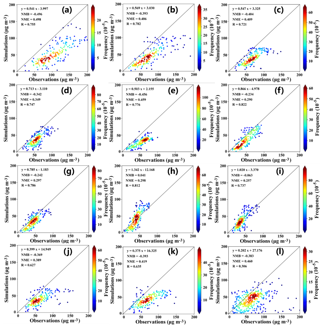
Figure S1. Density scatterplots of model performance and validation based on monthly mean observations; (a) to (l) are the results from January to December
