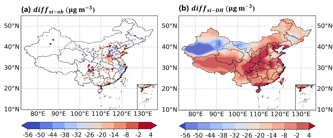
345 Figure 4. Spatial distribution of the annual mean simulated minus annual mean observed values (a), as well as the spatial distribution of the annual mean simulated values minus the Dalhousie dataset (b) for China in 2014 under scenario C1.
