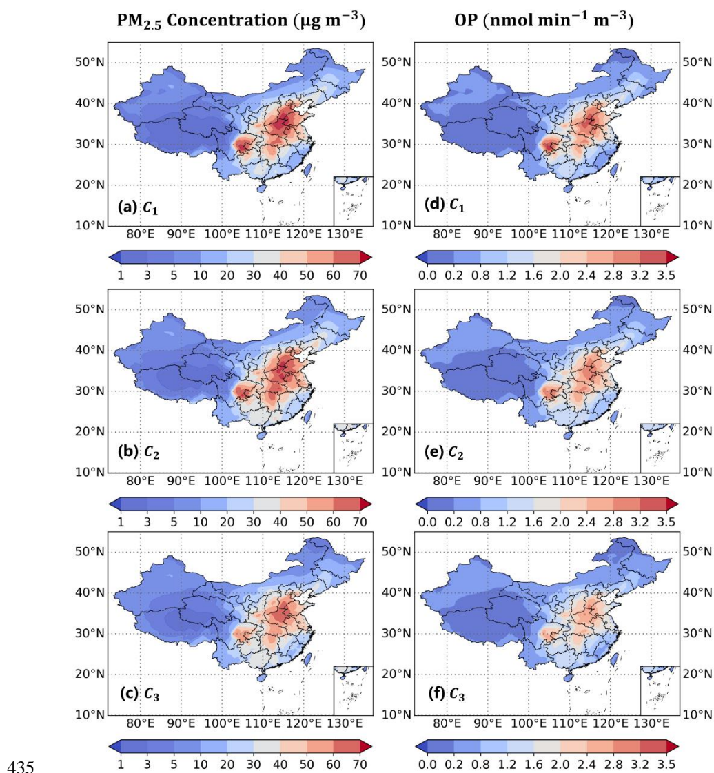
Figure 8. Spatial distribution of annual mean PM_{2.5} concentrations and annual mean OP for China in 2014 under different scenarios; (a)~(c) are PM_{2.5} concentrations in scenarios C_1 , C_2 and C_3 , respectively; (d)~(f) is the OP in scenarios C_1 , C_2 , and C_3 , respectively; The meteorological datasets (emission inventories) employed
