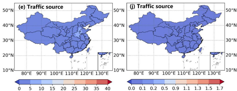
Figure 11. Spatial distribution of annual mean PM_{2.5} concentrations and annual mean OP from different anthropogenic sources for China in 2014 under scenario C1; (a)~(e) are PM_{2.5} concentrations derived from coal combustion for residential heating, biomass burning, secondary aerosol formation, industry, and traffic respectively; (f)~(j) are the OP derived from coal combustion for residential heating, biomass burning, secondary aerosol formation, industry, and traffic respectively.
