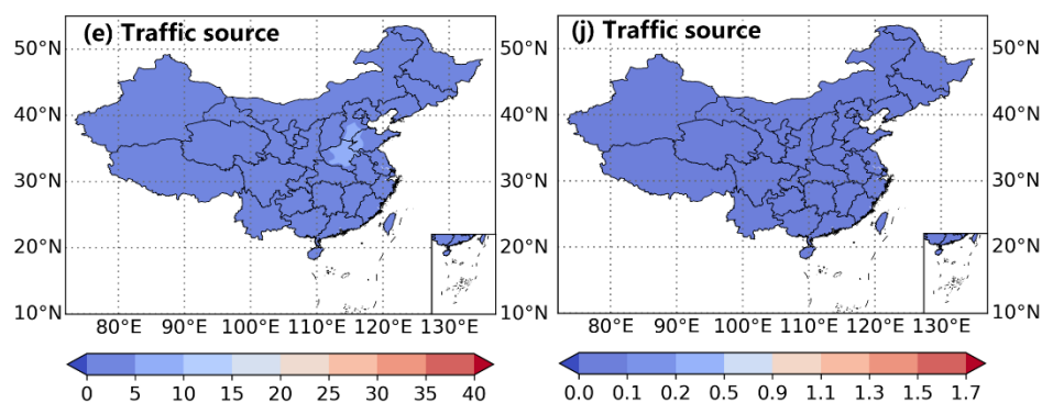
495 Figure 11. Spatial distribution of annual mean PM 2.5 concentrations and annual mean OP from different anthropogenic sources for China in 2014 under scenario C 1 ; (a)~(e) are PM 2.5 concentrations derived from coal combustion for residential heating, biomass burning, secondary aerosol formation, industry, and traffic respectively; (f)~(j) are the OP derived from coal combustion for residential heating, biomass burning, secondary aerosol formation, industry, and traffic respectively.
