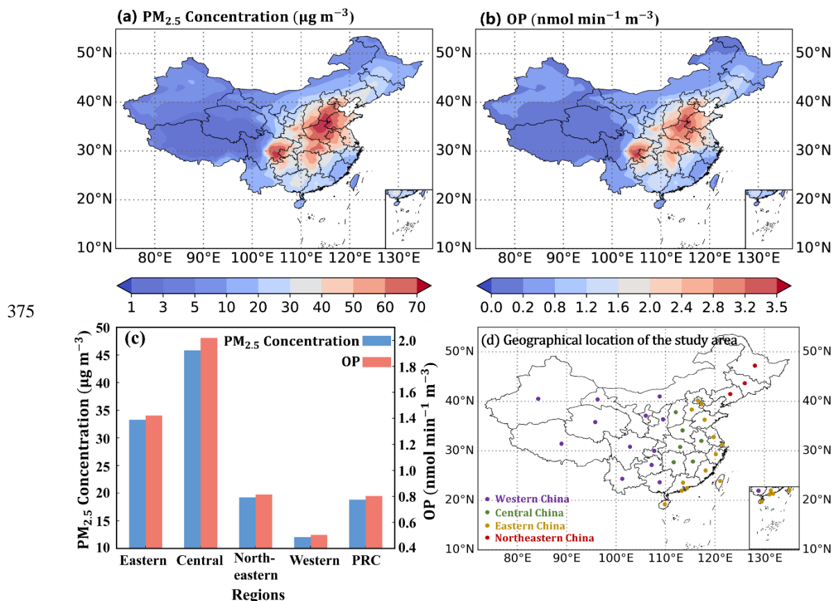
Figure 6. Spatial clustering of annual mean PM_{2.5} concentrations (a) and annual mean OP (b) in China, annual mean PM_{2.5} concentrations and annual mean OP (c) in different regions of China in 2014 under scenario C_1 , and geographical location of the study area (d); the central region of China comprises Shanxi, Anhui, Jiangxi, Henan, Hubei, and Hunan provinces; the eastern region of China comprises Beijing, Tianjin, Hebei, Shanghai, Jiangsu, Zhejiang, Fujian, Shandong, Guangdong, Hainan, Hong Kong, Macao, and Taiwan; It should be noted that the eastern region in this study includes Hong Kong, Macao and Taiwan; the western region of China consists of twelve provinces (autonomous regions and municipalities): Inner Mongolia, Guangxi, Chongqing, Sichuan, Guizhou, Yunnan, Tibet, Shaanxi, Gansu, Qinghai, Ningxia and Xinjiang; the northeastern region of China comprises Liaoning, Jilin and Heilongjiang provinces.
