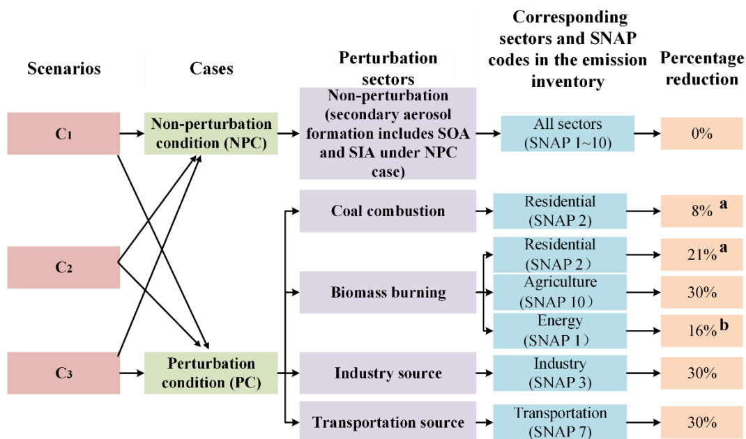
Figure 2. Emission reduction design for perturbed emissions; a was obtained from the literature (Yun et al., 2020), b were obtained from the literature (Zheng et al., 2018; Tong et al., 2018; Yun et al., 2020; MEE, 2020; Wang et al., 2020; Tang et al., 2020; Lin et al., 2021; Chen et al., 2022).
