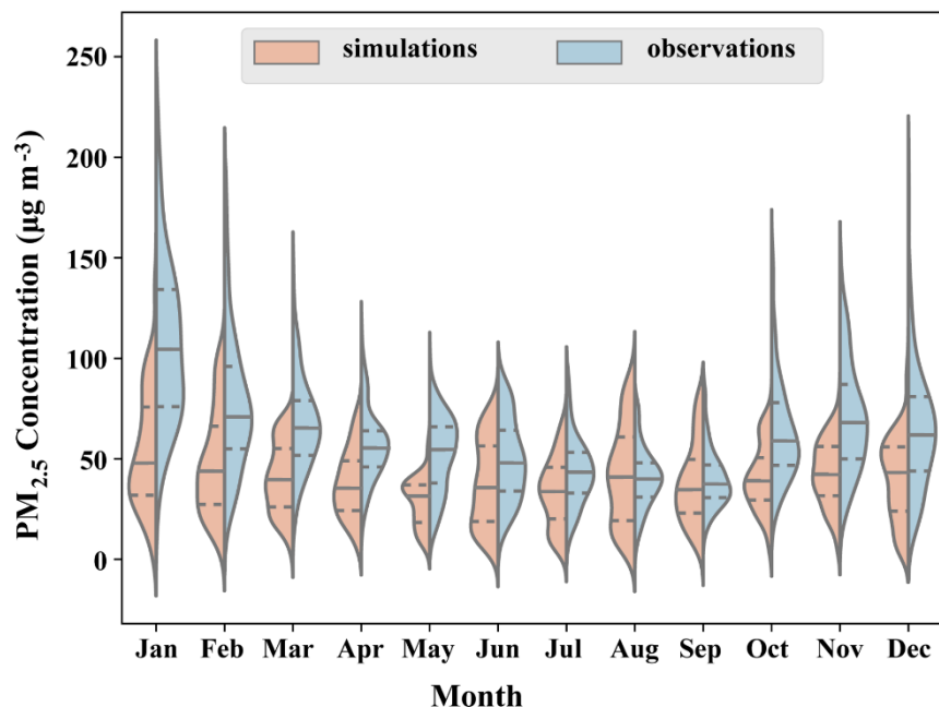
355 Figure 5. Violin plots of monthly average from MEE observations and simulations averaged over various observation stations for China in 2014 under scenario C 1 ; The red and blue colors represent the statistical distribution of simulated and observations, respectively; The width of the violin represents the sample size; The solid black line inside the violin indicates the median. The upper and lower dashed black lines within the violin indicate the upper quartile (the 75th percentile) and lower quartile (the 25th percentile), respectively.
