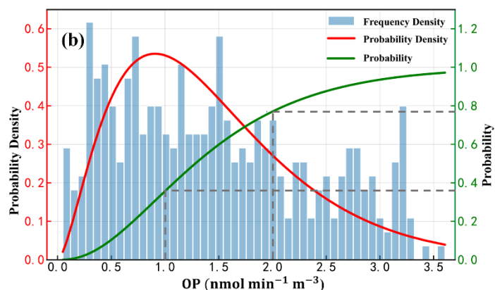
Figure 7. Probability distribution of (a) annual mean PM 2.5 concentrations and (b) annual mean OP for China in 2014 under scenario C 1 .
