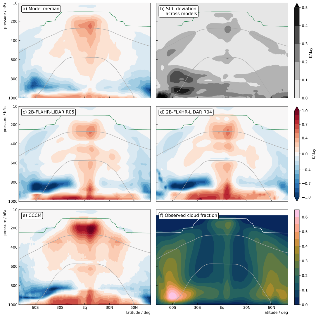
Figure 3. Model agreement and disagreement in cloud-radiative heating in models and observations . The upper row show the model median (panel a) of zonal-mean time-mean cloud-radiative heating and the standard deviation (panel b) across the amp simulations of the 20 CMIP6 models. The middle and lower row-rows shows the satellite-based estimates of cloud-radiative heating from the products 2B-FLXHR-LR R05 and R04 (panel-panels c and d) and CCCM (panel e). Observed cloud fraction is shown in panel f . In all panels, the gray lines mark the model median of the 0 and -38 deg C isotherms and the green line marks the model median of the thermal tropopause ( white line in panel f ).
