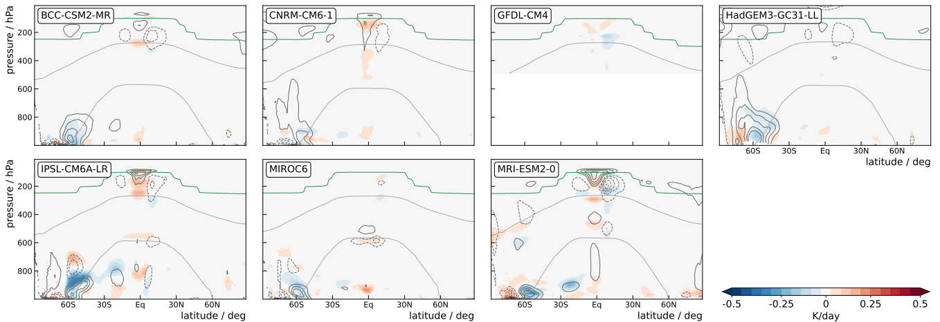
Figure 10. Difference between the zonal-mean time-mean cloud-radiative heating in the amip-future4K and amip-p4K simulations (amip-future4K - amip-p4K). The darker gray contour lines mark the 0 and -38 deg C isotherms, and show the green lines difference in zonal-mean time-mean cloud fraction between the thermal-tropopause two simulations (amip-future4K - amip-p4K; solid for amip-positive and dashed for amip-future4K negative values, contour spacing of 0.01). Cloud-radiative heating in For GFDL-CM4, cloud fraction is not available and cloud-radiative heating is restricted to above 500 hPa because it is derived from zonal-mean heating rates in the amip-future4K simulation but zonally-resolved heating rates in the amip-p4K simulation (cf. Tab. 1). This leads to spurious differences below 500 hPa due to topography. The gray lines mark the 0 and -38 deg C isotherms and the green lines the thermal tropopause for the amip simulations.
