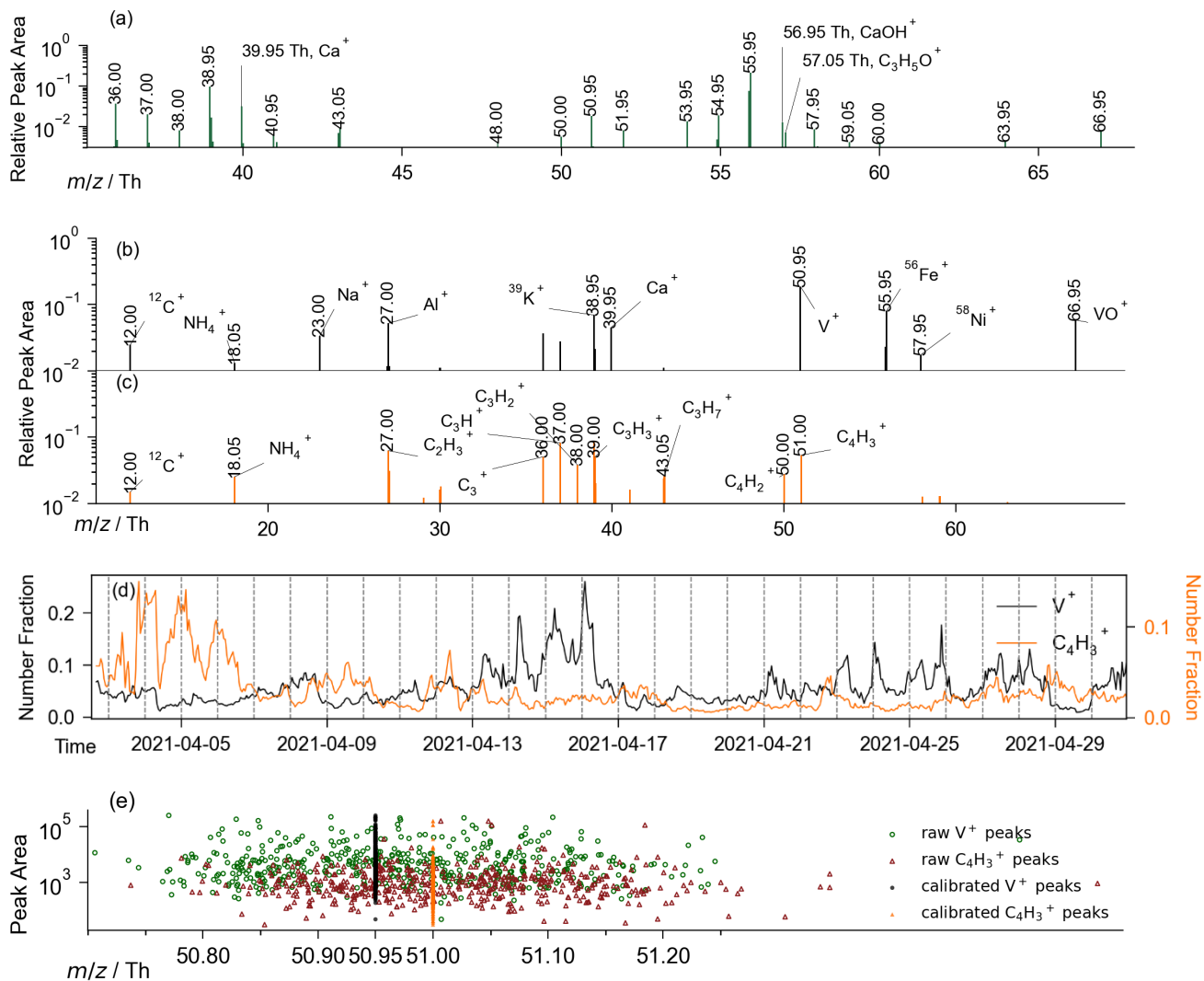
260 Figure 5. (a) Averaged spectrum (locally illustrated) of 5,601 spectra that simultaneously contain CaOH + and C 3 H 5 O + . Averaged positive spectrum of (b) V + -containing (in gray) and (c) C 4 H 3 + -containing (in orange) particles were obtained by averaging millions of particles of the two particle groups separately. (d) Time series of V + -containing and C 4 H 3 + -containing particles in number fraction. (e) Raw and calibrated peaks around 51 Th of 1000 randomly chosen V + -containing or C 4 H 3 + -containing particles.
