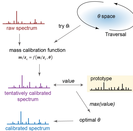
135 Figure 1. Simplified procedure of the calibration algorithm. Raw spectrum is calibrated using mass deviation function with candidate coefficient pairs \theta_i to generate initially calibrated spectra. A value is calculated using a value function based on a prototype dataset. A calibrated spectrum is obtained when the value is maximal.
