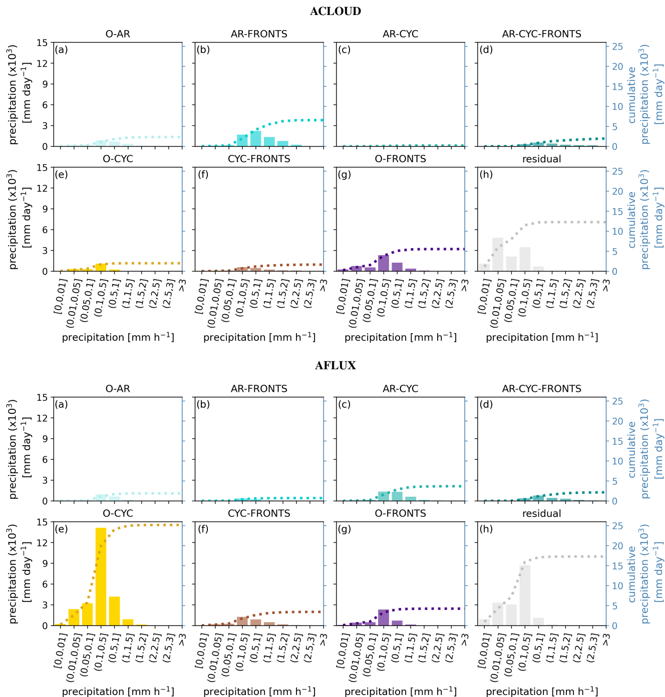
Figure 5. Contribution of different precipitation rates [ \text{mm h}^{-1} ] to the daily averaged precipitation [ \text{mm day}^{-1} ] for co-located and separated components (a-h) during ACLOUD (top) and AFLUX (bottom). The accumulated daily precipitation rate [ \text{mm day}^{-1} ] is shown by the dotted line and their value is given by the y-axis. Note, that each 0.25 \times 0.25 grid cell is not area-weighted. Thus, the sum of the cumulative precipitation deviates from Table 1 which includes the area-weighted precipitation. The contribution of the area-weighted precipitation is shown in Fig. A3.
