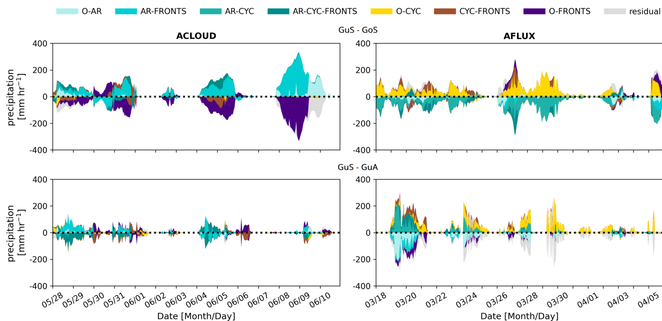
Figure 9. Time series for ACLLOUD (left) and AFLUX (right) showing the difference of the contribution to precipitation by using different algorithms. Comparison of AR algorithms (GuS - GoS) ((a) and (b)), and comparison of cyclone algorithms (GuS - GuA) ((c) and (d)) for co-located and separated components (colors as in Fig. 1).
