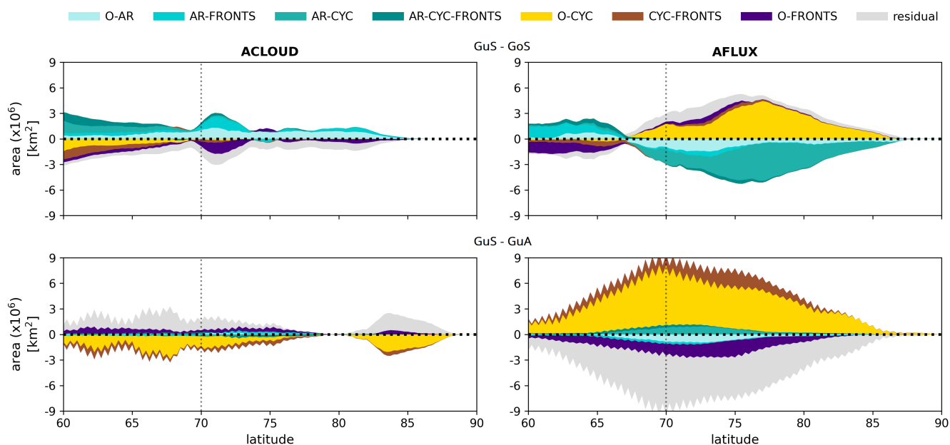
Figure 10. Latitudinal dependence for ACLLOUD (left) and AFLUX (right) regarding the difference of the affected area by using different algorithms. Comparison of AR algorithms (GuS - GoS) ((a) and (b)), and comparison of cyclone algorithms (GuS - GuA) ((c) and (d)) for co-located and separated components (colors as in Fig. 1). The zigzag pattern in (c) and (d) is caused by the interpolation to the 0.25° ERA5 grid.
