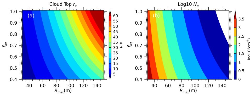
Figure 2. Response of Equation 18 (a - r_e ) and Equation 17 (b - N_d ) to typical values of R_{max} and f_{ad} .
