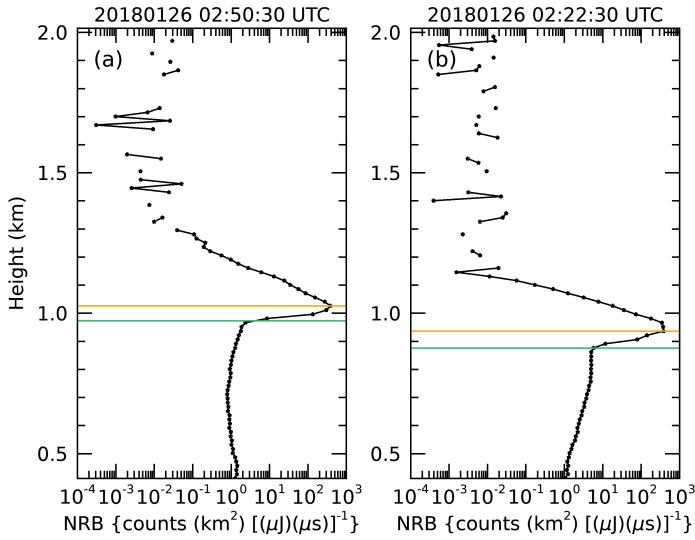
Figure 1. Two Examples of Normalized Relative Backscatter (NRB; Campbell et al., 2002) from Micropulse Lidar data collected during Marcus on January 26, 2018. a) shows a profile in a non-drizzling cloud collected at 02:50:30 UTC . b) shows a profile collected at 02:22:30 that had sub cloud drizzle as indicated by the cloud radar. The green line indicates the height determined to be cloud base while the red line indicate the maximum in \beta_{obs} . The distance between the green and red lines is defined as r_{max} .
