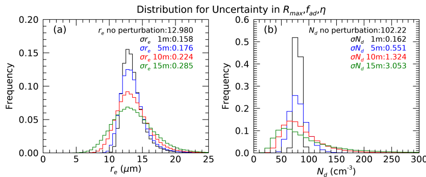
Figure 3. Sensitivity of Eqns. 17(a) and 18(b) to uncertainty in input parameters. Inset lists the resulting uncertainties corresponding to the color-coded frequency distributions. Insets list normalized standard deviations for an assumed standard deviation in R_{max} of 1, 5, 10, and 15 m. The lidar range gate spacing would be twice the standard deviation in R_{max} .
