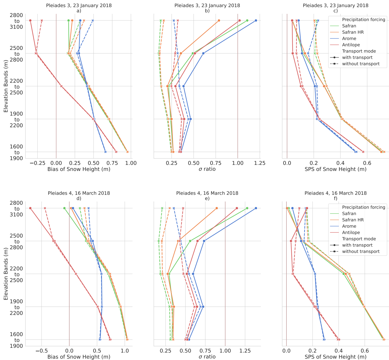
Figure 8. Scores comparing simulations with the Galibier Pléiades observations. (a-b-c) compares simulations with the 23 January 2018 Pléiades 3 image ; (d-e-f) is based on the 16 March 2018 Pléiades 4 image. (a-d) Bias (m) ; (b-e) Standard deviation ratio (no unit) ; (c-f) SPS (m). All scores are presented as a function of 300 m elevation intervals.
