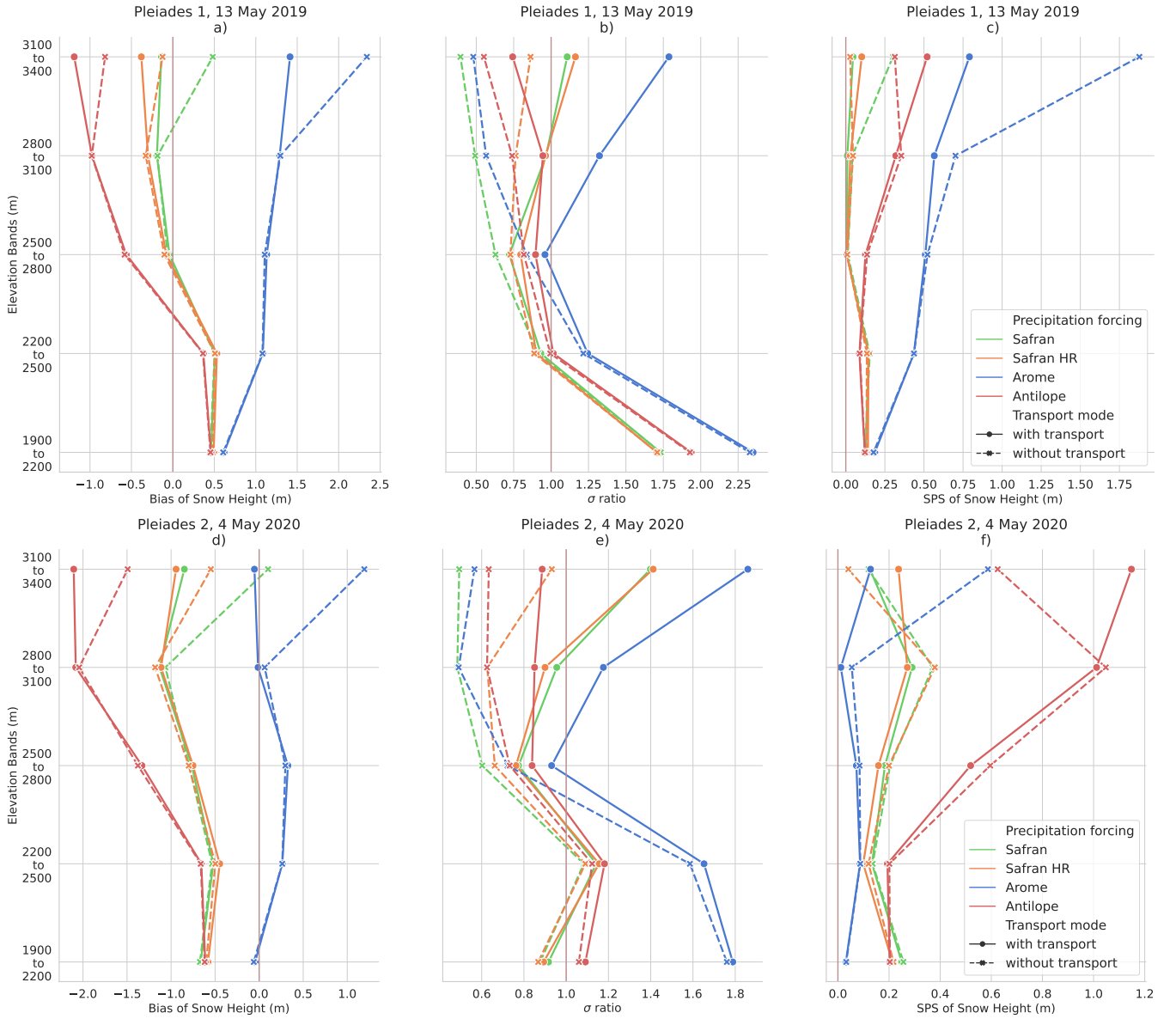
Figure 6. Scores comparing simulations with the Grandes Rousses Pléiades observations. (a-b-c) compares simulations with the 13 May 2019 Pléiades 1 image ; (d-e-f) is based on the 4 May 2020 Pléiades 2 image. (a-d) Bias (m) ; (b-e) Standard deviation ratio (no unit) ; (c-f) SPS (m). All scores are presented as a function of 300 m elevation intervals.
