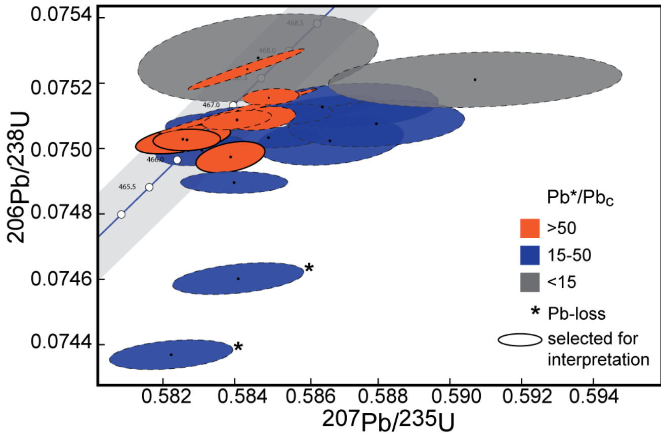
Fig. 1) Concordia diagram generated in ETRedux v. 3.7.1, using colour coding for bands of Pb^*/Pb_c as discussed in the text for the error ellipses as a function of the Pb^*/Pb_c value. Red-Orange colours indicates higher Pb^*/Pb_c > 50 , whereas blue colours indicates low Pb^*/Pb_c values between 15-50, grey error ellipses indicate Pb^*/Pb_c < 15 . Ellipses marked by an asterisk are interpreted to be affected by Pb-loss. Black outline indicates analyses considered for the weighted mean age, where the selection criterion is Pb^*/Pb_c > 50 and analytical concordance (part or full ellipse overlaps with the uncertainty band of the Concordia curve). Grey band illustrates the uncertainty band of the Concordia curve.
