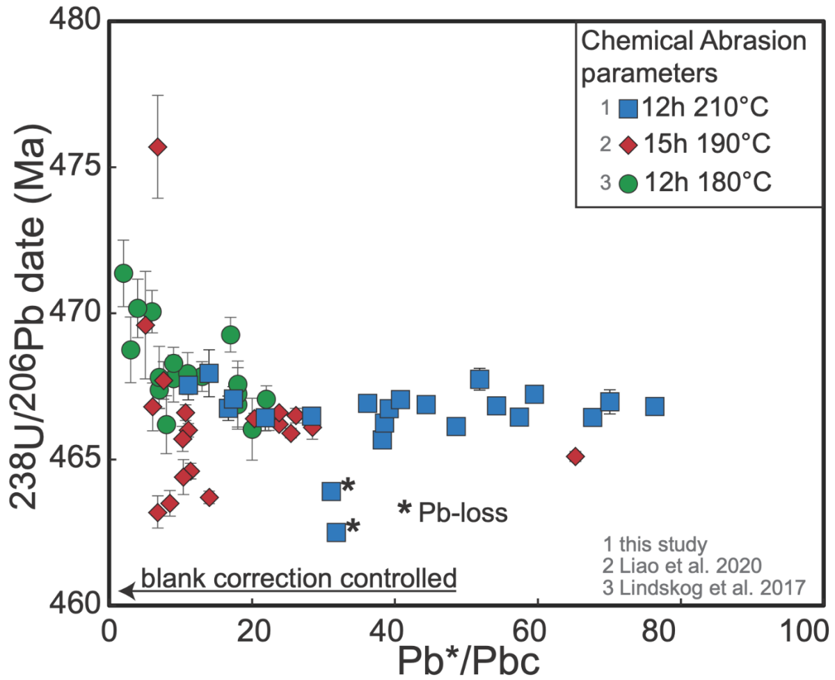
Fig. 3) Comparison of calculated ^{238}\text{U}/^{206}\text{Pb} zircon dates with their respective \text{Pb}^*/\text{Pb}_c values. Low \text{Pb}^*/\text{Pb}_c values typically indicate stronger effects of blank correction on the calculated ^{238}\text{U}/^{206}\text{Pb} dates (Schaltegger et al. 2021). Colours indicate the different studies and differences in their chemical abrasion procedure. Samples marked with an asterisk are discordant in concordia space (see Fig. 1).
