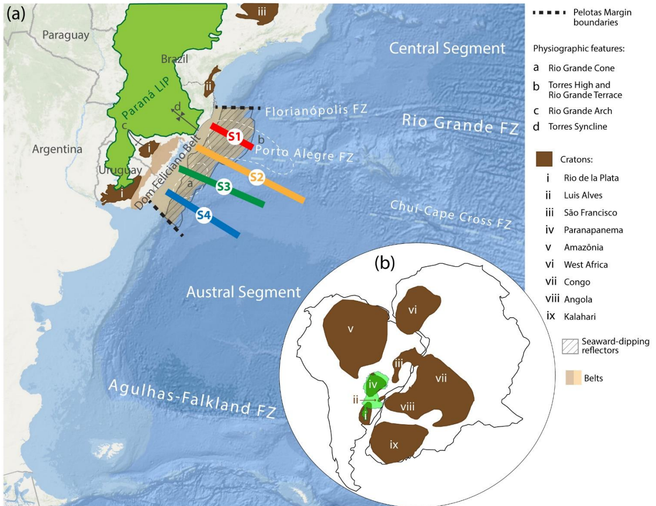
65 Figure 1: (a) Map of the Austral South Atlantic (adapted from Cassel et al., 2022) showing: the location of the 4 Pelotas Margin seismic reflection profiles examined in this study; the distribution of seaward-dipping reflectors from Chauvet et al. (2021); crustal basement from Stica et al. (2014); and Paraná Large Igneous Province (LIP) adapted from Rossetti et al. (2018). (b) Regional paleo-map of Western Gondwana adapted from Heilbron et al. (2008) showing the Paraná LIP and cratons.
