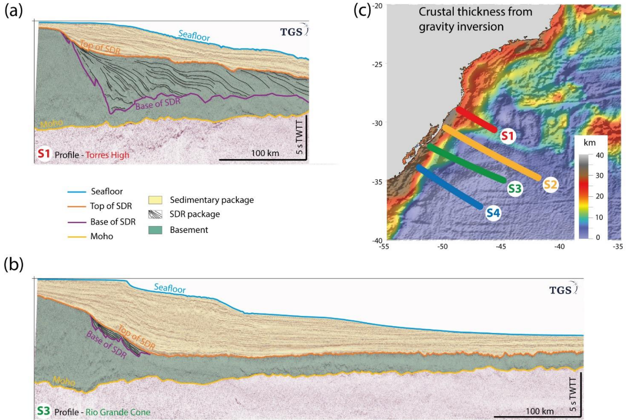
115 Figure 2: (a) Seismic profiles in TWTT showing interpreted surfaces and units for profile S1 (b) Seismic profiles in TWTT showing interpreted surfaces and units for profile S3. (c) Locations of the 4 seismic profiles superimposed on map of crust thickness from gravity inversion (adapted from Graca et al. 2019): Profile S1 is located in the northern Pelotas margin along the Torres High. Profile S3 is located in the southern Pelotas margin crossing the Rio Grande Cone.
