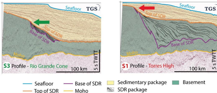
225 Figure 8: (a) Maximum thickness of SDRs in TWTT for profiles S1-S4 plotted against latitude showing north to south decrease. (b) TWTT of first proximal occurrence of SDRs plotted against latitude showing north to south decrease. (c and d) Comparison of the seismic reflection sections for S3 and S1 in TWTT highlighting the first proximal occurrence of SDRs.
