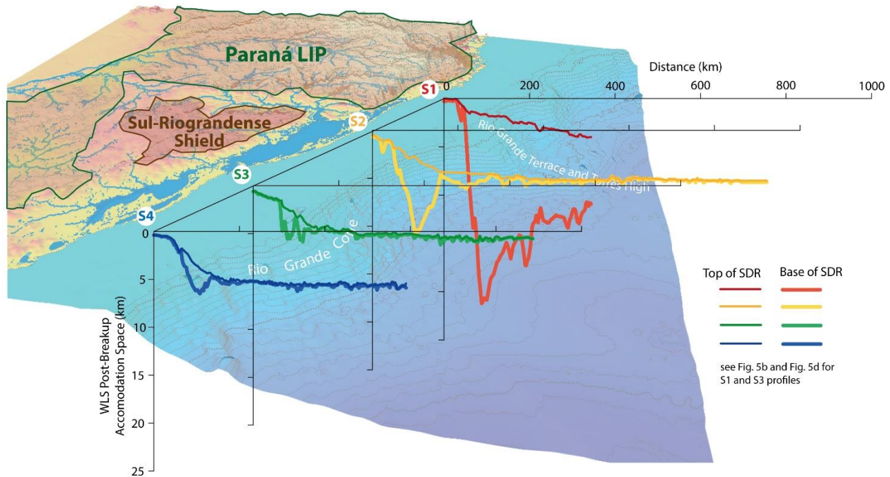
200 Figure 7: Comparison of water-loaded post-rift accommodation space for the 4 profiles S1-S4 showing north to south variation along the Pelotas margin. Profiles S1 (Torres High) is offshore Serra Geral volcanics of the Parana LIP. Profiles S3 is offshore cratonic lithosphere of the Sul Riograndense Shield (SRS) where Serra Geral is absent.
