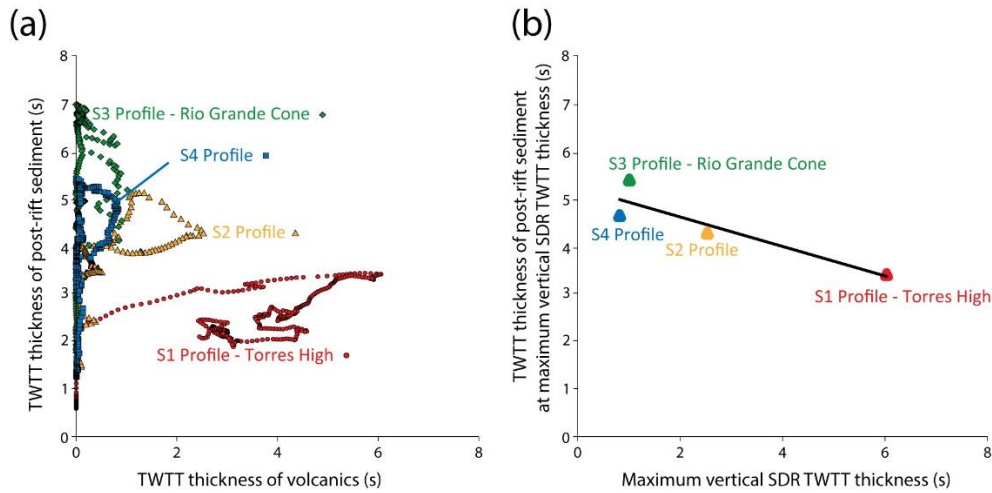
130 Figure 4: (a) Plot of TWTT thickness of post-rift sediment against TWTT thickness of SDR for the same 300 km profile horizontal distance for each of the 4 profiles S1-S4. (b) Plot of TWTT thickness of post-rift sediment at maximum vertical SDR TWTT thickness against maximum vertical SDR TWTT thickness at the same horizontal profile distance for each profile S1-S4.
