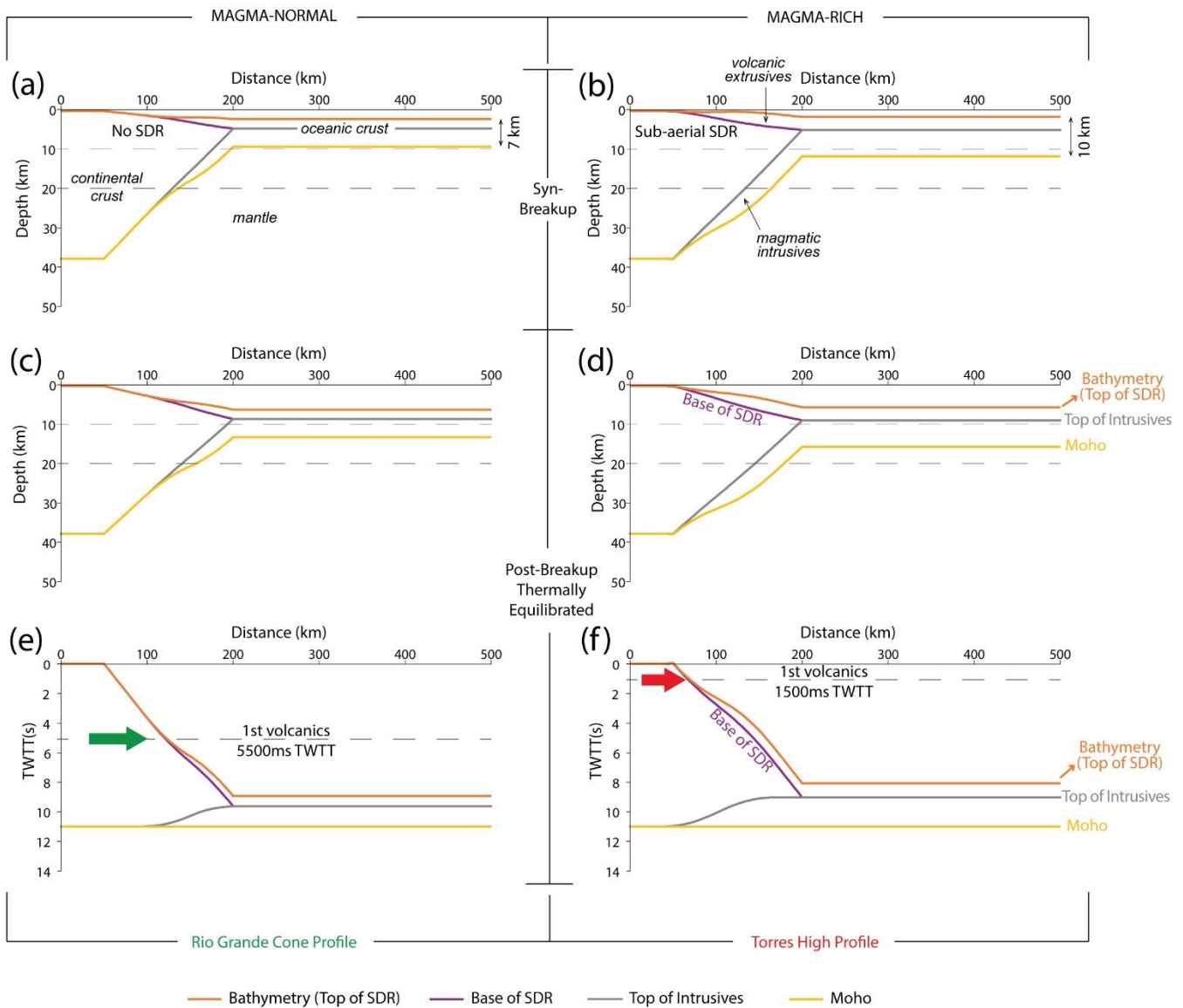
300 Figure 9: Isostatically balanced model cross-sections of a rifted margin with varying amounts of magmatic addition. (a and b) at breakup time with syn-rift lithosphere thermal uplift. (c and d) at large post-breakup time with full lithosphere thermal re- equilibration. (e and f) Time domain representation of model cross-sections for full lithosphere thermal re-equilibration converted from depth model using Warner’s “10 second rule” (1987). The proximal onset of first volcanics is indicated by the coloured arrows. Left column: an idealized margin with normal magmatic addition as for the Rio Grande Cone S3 Profile. Right column: an idealized 305 magma-rich margin as for the Torres High S1 Profile.
