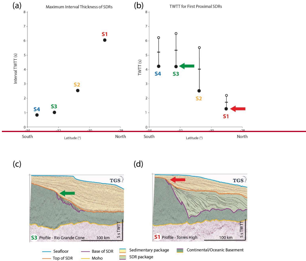
245 Figure 8: (a) Maximum thickness of SDRs in TWTT for profiles S1-S4 plotted against latitude showing north to south decrease. (b) TWTT of first proximal occurrence of SDRs plotted against latitude showing north to south decrease. (c and d) Comparison of the seismic reflections sections for S3 and S1 in TWTT highlighting the first proximal occurrence of SDRs.
