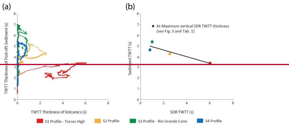
140 Figure 4: (a) Plot of TWTT thickness of post-rift sediment thickness in TWTT against TWTT thickness of SDR thickness in TWTT for at the same 300 km profile horizontal distance location out to profile distance 300 km for each of the 4 profiles S1-S4. (b) Plot of TWTT thickness of post-rift sediment at maximum vertical SDR thickness in TWTT thickness against maximum vertical SDR thickness-TWTT thickness at the same horizontal profile distance location for each profile S1-S4.
