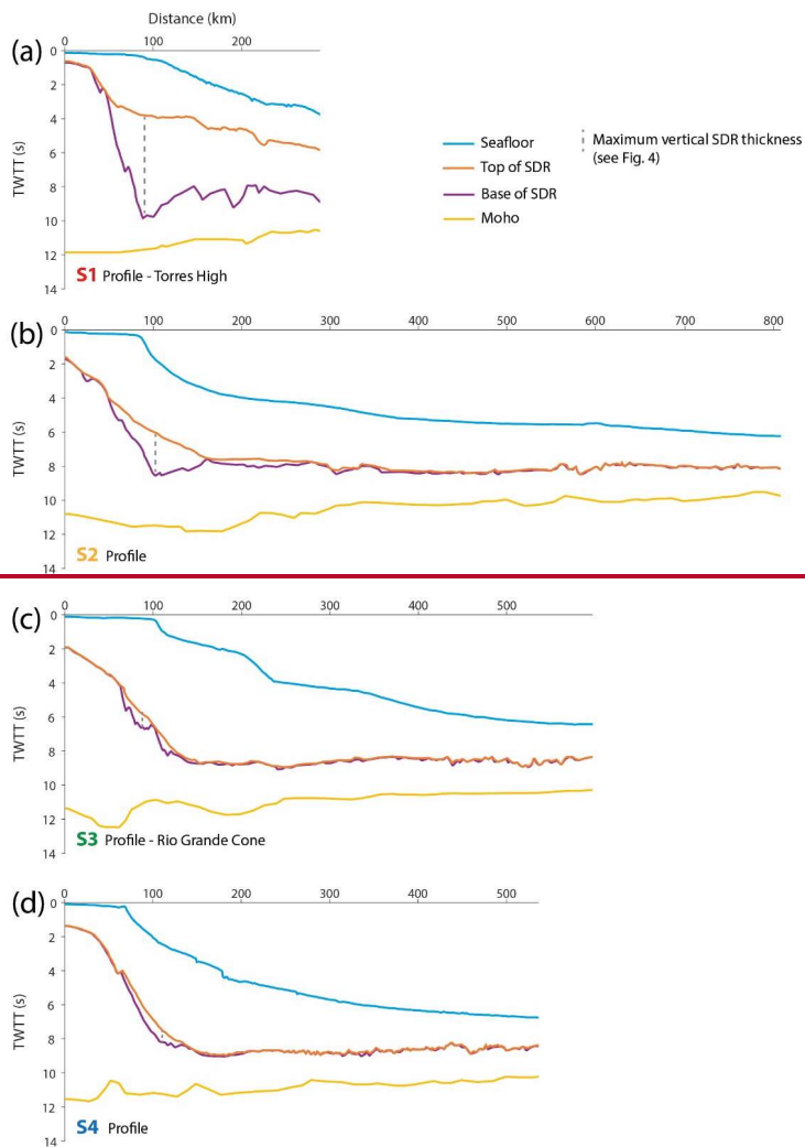
135 Figure 3: Comparison of the 4 seismic profiles showing the interpreted surfaces in TWTT. (a) Seismic profile S1, located in the northern Pelotas Basin-margin crossing the Torres High. (b) Seismic profile S2. (c) Seismic profile S3 located in the southern Pelotas Basin-margin crossing the Rio Grande Cone. (d) Seismic profile S4.
