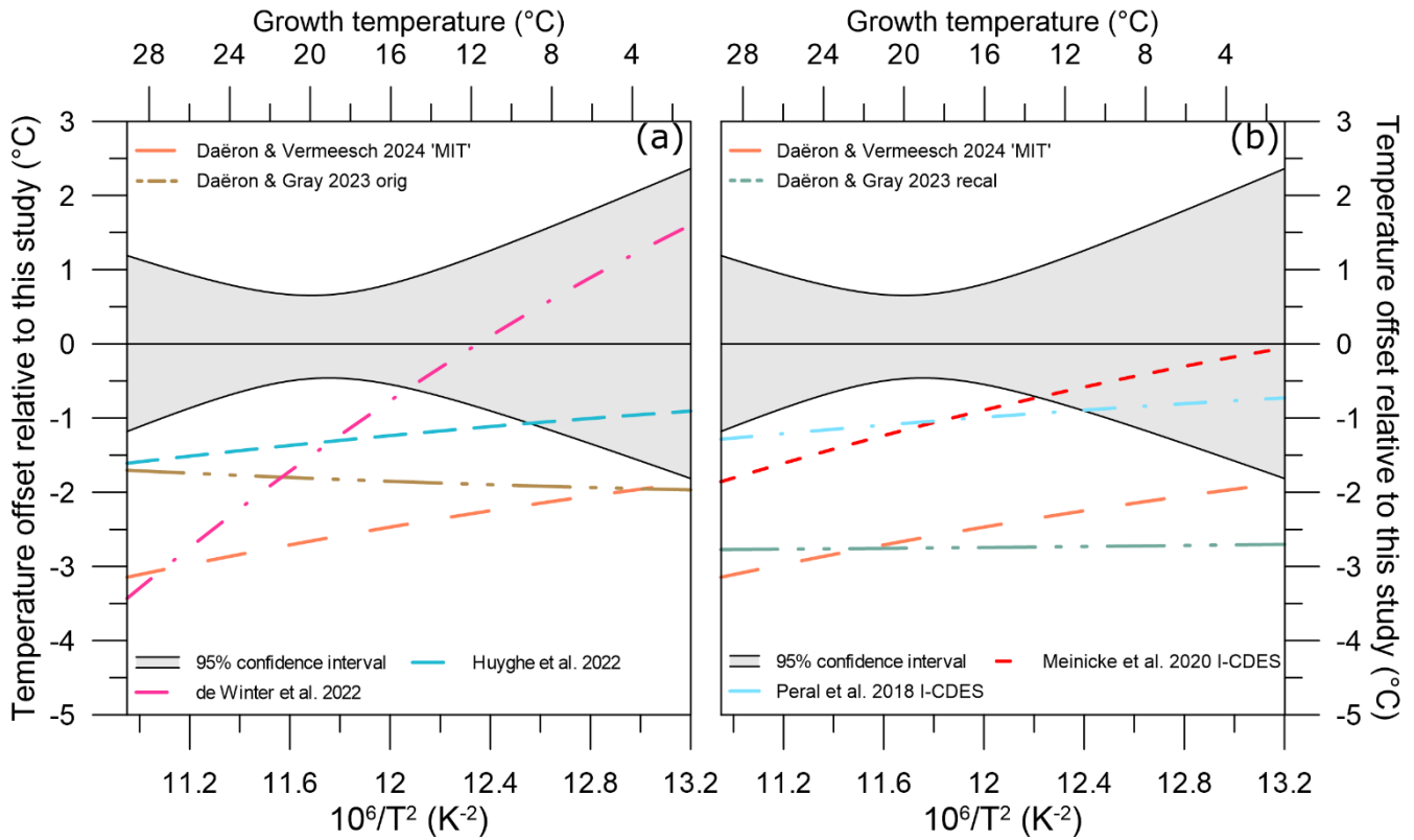
950 Figure 8. Temperature offset of different \Delta_{47} -temperature calibrations relative to our study's equivalent temperature. a) Temperature offsets of two non-foraminifera biogenic carbonate calibration studies; de Winter et al. (2022; pink dash-dot-dash line) and Huyghe et al. (2022; blue dashed line). b) Temperature offsets of two planktic foraminifera biogenic carbonate calibration studies; Peral et al. (2018; light blue dash-dot-dash line) and Meinicke et al. (2020; red dashed line), using original published temperatures. Other included studies' calibration data are colour coded following Fig. 7. The 95% confidence interval for our study is given as light grey shading.
