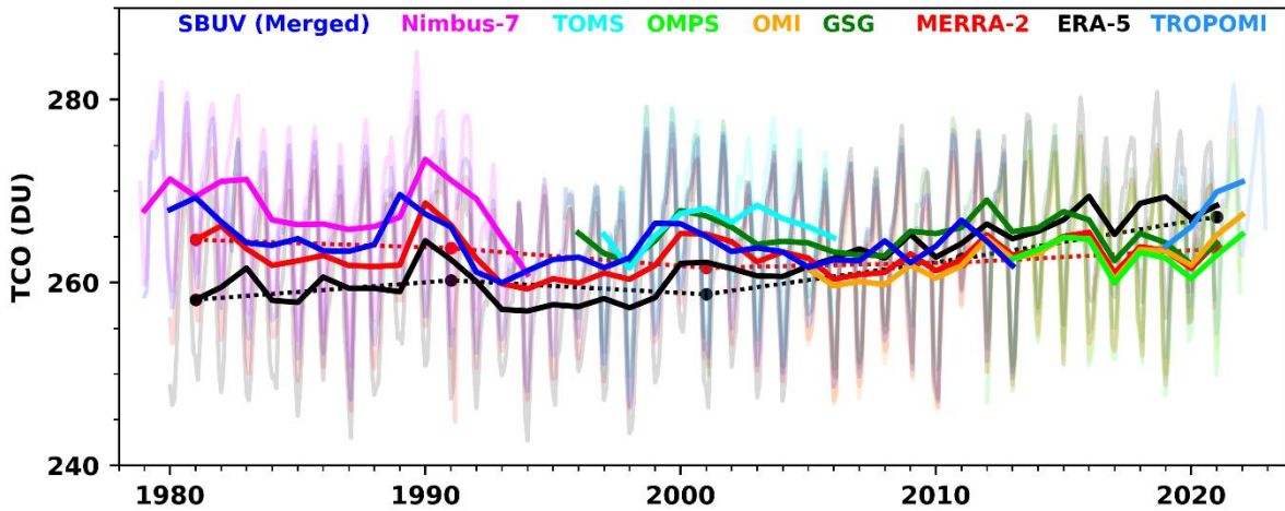
Figure 2: The distribution of Total Column Ozone (TCO in DU) averaged over the tropics (30° S–30° N) from different satellites from 1978 to 2022. The light lines show the monthly distribution, whereas dark lines show the annually averaged value of TCO. The dotted line shows the decadal distribution of TCO from MERRA-2 and ERA-5. Here, TOMS is Total Ozone Mapping Spectrometer, OMPS is Ozone Mapping and Profiler Suite, OMI is Ozone Monitoring Instrument, TROPOMI is Tropospheric Ozone Monitoring Instrument and GSG is Global Ozone Monitoring Experiment (GOME) - Scanning Imaging Absorption spectroMeter for Atmospheric CHartography (SCIAMACHY) - GOME-2 satellite data. MERRA-2 is Modern-Era Retrospective analysis for Research and Applications, version 2 reanalysis and ERA-5 is the 5 th Generation European Centre for Medium-Range Weather Forecasts (ECWMF) atmospheric reanalysis data set. The peak in 1991 may be driven by the Mount Pinatubo volcanic eruption.
