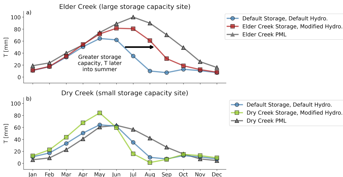
Figure 7. Comparison between average monthly ET as estimated by LPJ-GUESS using different storage and hydrology and from PML-V2 for (a) Elder Creek, which has large subsurface storage capacity and (b) Dry Creek, which has small subsurface storage capacity. Transpiration from PML (black triangles) shows sustained T (transpiration) into the dry season. LPJ-GUESS best approximates this behavior at Elder Creek with both greater subsurface storage capacity and the modified hydrology routine.
