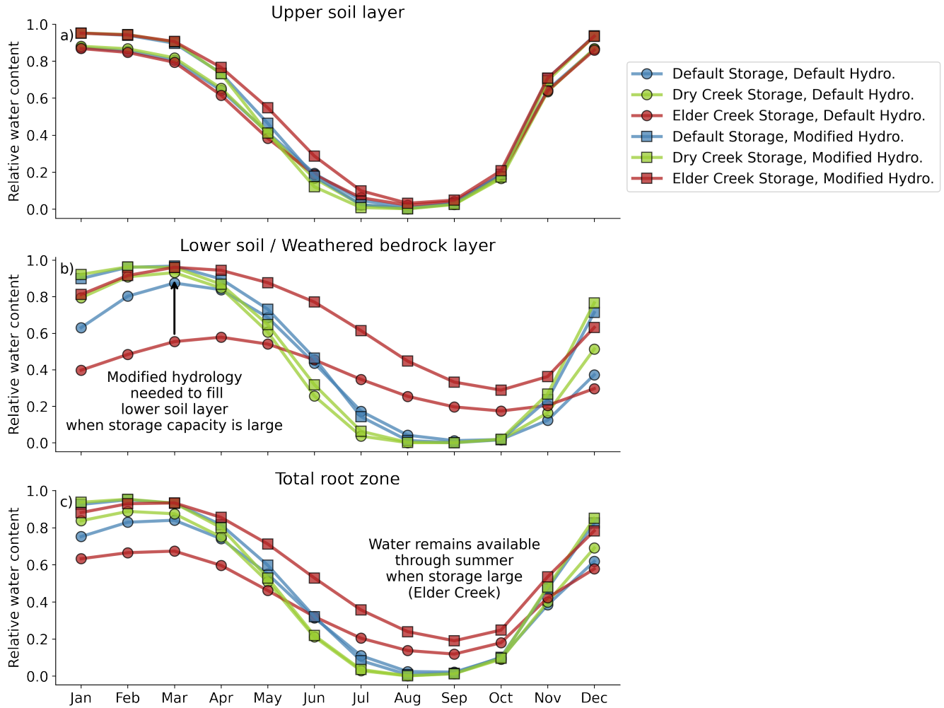
Figure 4. Monthly mean relative water content in the (a) upper soil layer, (b) lower soil or weathered bedrock layer and (c) total root zone for each model setup. Squares denote the modified hydrology scheme, and circles denote the default hydrology scheme. Color indicates the subsurface storage, with Blue default, green Dry Creek, and red Elder Creek. Default and Dry Creek water contents go to zero in the summer for both hydrology schemes. Only the large storage capacity for Elder Creek allows for sustained water supply through the summer. By comparing the circles and squares for each storage, it is clear that more water enters the lower layer with the modified hydrology scheme in the wet season, leading to enhanced water availability even with the same storage.
