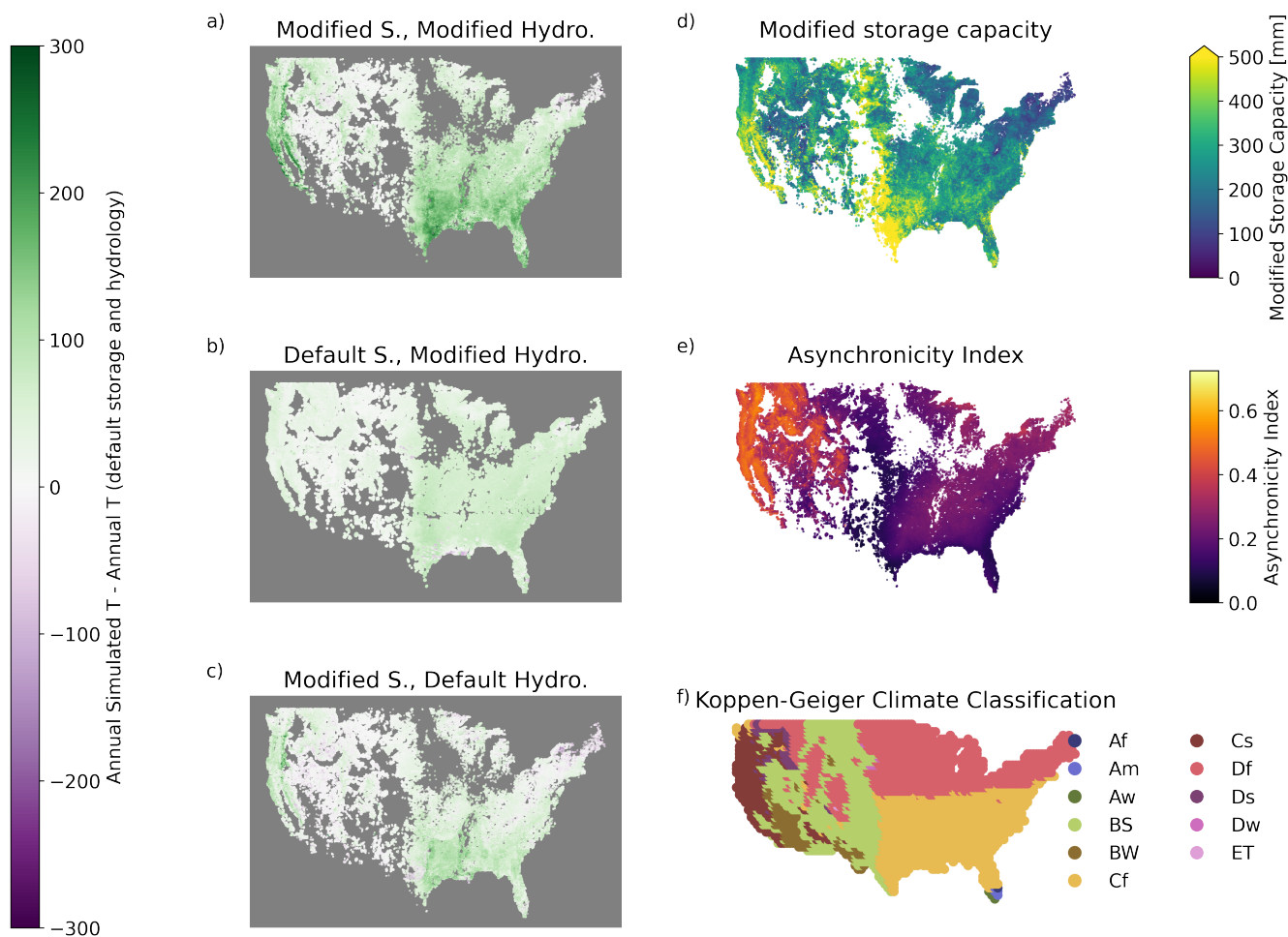
Figure 8. (a)-(c) Difference in simulated annual T between each modified simulation and the simulation with default storage capacity and hydrology. In (a), regions with largest enhancement in T from modifications to storage and hydrology include the West Coast, Texas, and the Southeast. (d) Root-zone storage used for the modified storage capacity, as described in Section 2.3. Largest storage capacities are found in California and in a vertical band running north from Texas. (e) Asynchronicity index, demonstrating difference in seasonality between ET and precipitation at each pixel, following Feng et al. (2019). See Section 2.3 for more detail. (f) Koppen Geiger Climate Classification from Kottek et al. (2006). Symbols are defined as: Af–tropical rainforest, Am–Tropical monsoon, Aw–Tropical savanna, BS–Dry Semi-Arid, BW–Dry Arid Desert, Cf–Temperate No dry season, Cs–Temperate Dry summer, Df–Continental No dry season, Ds–Continental Dry summer, ET–Polar Tundra.
