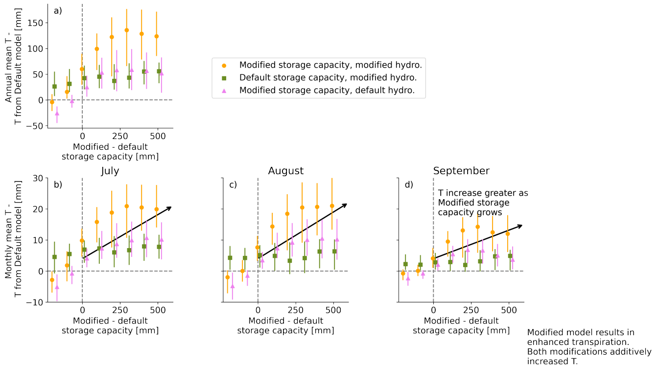
Figure A4. Binned histograms of the difference in simulated Transpiration (T) between each simulation and the simulation with default storage capacity and hydrology as a function of the change in storage capacity from the default to modified for (a) annual T and (b)-(d) monthly T for July, August, and September, respectively. Grey dashed lines mark (horizontal) no T change from the default model and (vertical) no storage capacity change between the modified and default storage capacity. Vertical lines for each marked point indicate the spread from 25th-75th percentile. There is little change in T for locations with a change in storage of <100 mm. Greater than 100 mm, though, both the modified hydrology and modified storage capacity separately result in enhanced T, with the combined effect for the fully modified simulation an average of about 100 mm annual increase for sites with large modified storage capacity or a monthly difference of about 20 mm in August. The result is significantly enhanced T, with the largest effect at sites with the largest storage capacity in the modified model.
