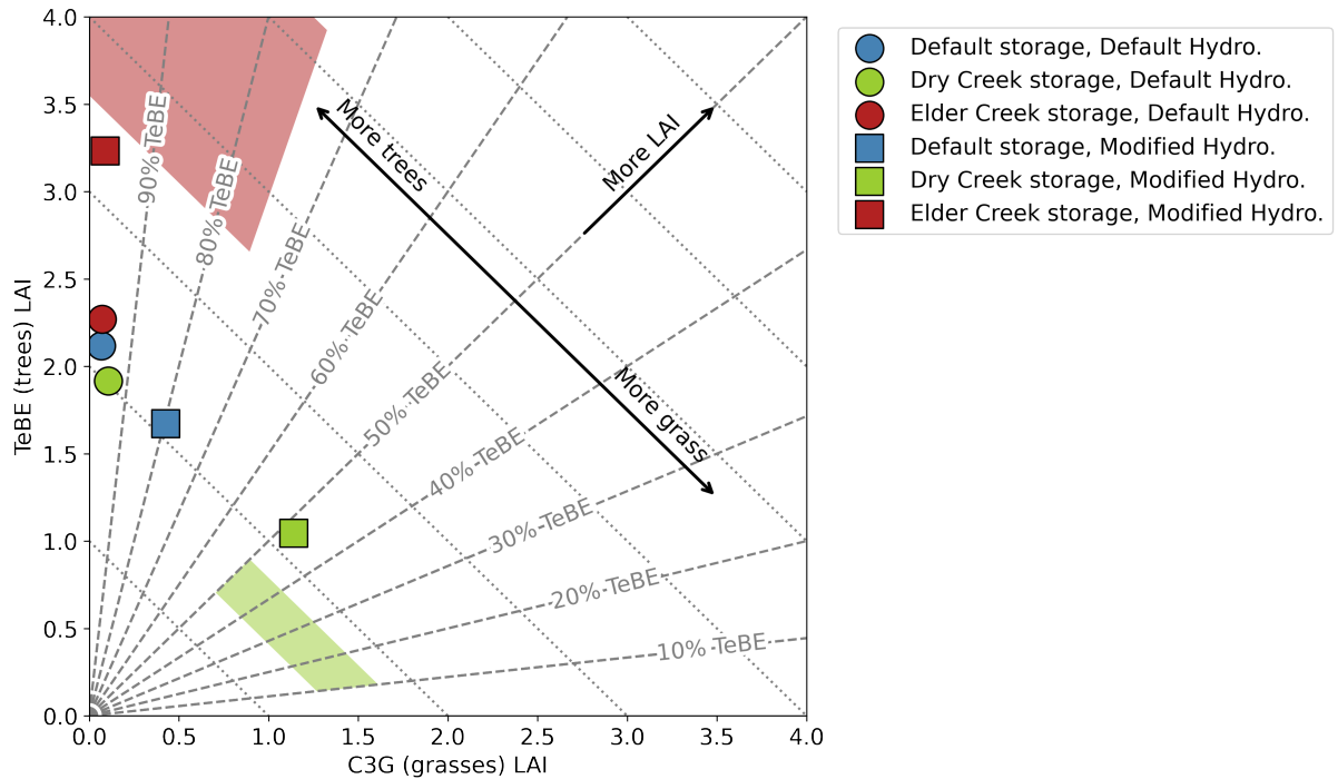
Figure 5. Predicted vegetation community, as measured by fraction of LAI devoted to C3G (C3 grass) versus TeBE (temperate broadleaf evergreen tree). The shaded regions denote the actual vegetation community composition at (red) Elder Creek and (green) Dry Creek, estimated from field observations. Dotted lines indicate lines of constant total LAI, and dashed lines indicated lines of constant ratio between TeBE and C3G. Default model configuration (blue circle) does not closely match either the Dry Creek or Elder Creek biome. It is necessary to modify both the hydrology scheme (squares) and the subsurface storage capacity (red for Elder Creek and green for Dry Creek) to achieve the best match to the actual vegetation community.
