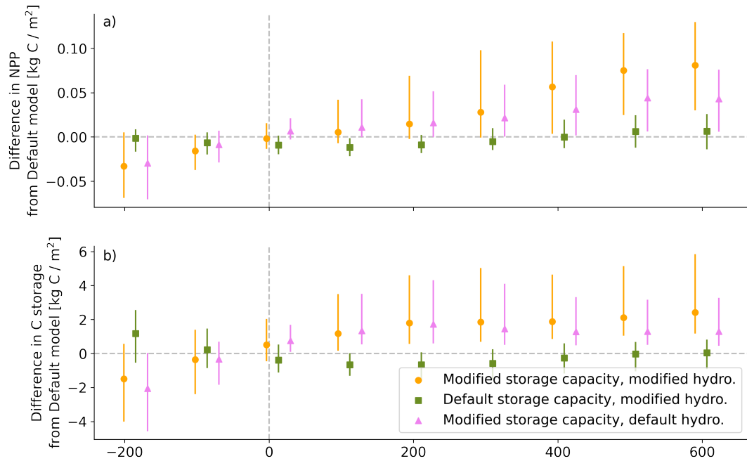
Figure A2. Impact of modified hydrology and storage relative to default LPJ-GUESS model on (a) Net primary productivity (NPP) and (b) Carbon sequestration. Both NPP and C are enhanced with modified storage and hydrology schemes.
