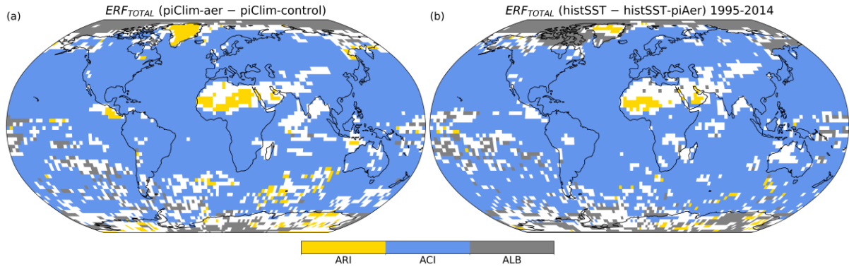
Figure 6. Areas where each of the three main ERF components ( ERF_{ARI} , ERF_{ACI} , and ERF_{ALB} ) dominates the total ERF. The absolute values of ERF_{ARI} , ERF_{ACI} , and ERF_{ALB} are summed, and every grid cell is colored after the ERF component that contributes at least 50% to the resulting value, while each of the other two components contributes less than 33% to the resulting value. In cases where the above criterion is not met, the grid cell is colored white.
