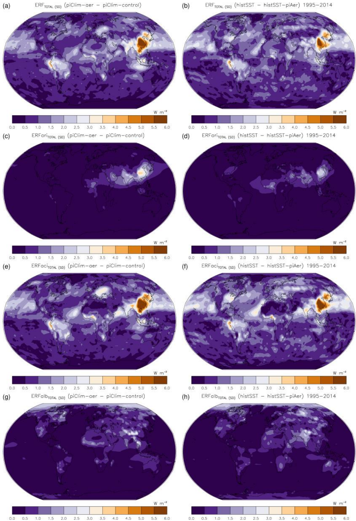
Figure 1: Inter-model variability (one standard deviation) of total (SW+LW) ERF (a, b), ERFari (c, d), ERFaci (e, f) and ERFalb (g, h) due to all anthropogenic aerosols relative to the pre-industrial era. The spatial distribution is presented for the multi-model ensembles of piClim-aer (left column) and histSST (averaged over 1995–2014; right column) experiments, respectively.
