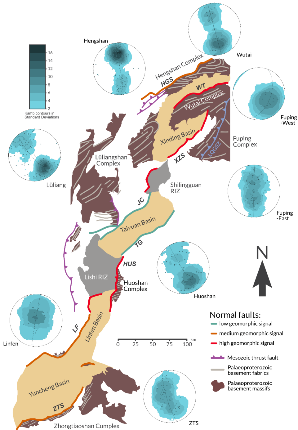
Figure 5: Schematic fault map of the Shanxi Rift with faults colour coded according to their geomorphic signal – compare with Table 1. Exposed basement of the TNCO in brown with the main structural trends highlighted in light grey. Stereonets of poles to
