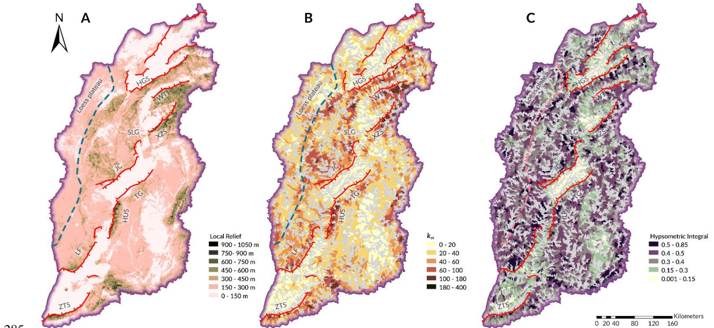
290 Figure 6: Geomorphic indices map of the Shanxi Rift. Major extensional faults shown in red, boundary of the Loess plateau indicated by dashed line A) Local relief map. Darker colours indicate higher relief regions. Local relief was calculated within a 1km circular radius. High relief is found especially in the northern Shanxi Rift in the footwalls of the Wutai and Xizhoushan faults as well as further south along the Huoshan and Zhongtiaoshan faults. Noticeably lower local relief values occur along the central Jiaocheng and Taigu faults. B) Mean normalised channel steepness ( k_{sn} ) calculated for 1st Strahler order basins. High values are commonly located in the footwalls of active faults, especially the Wutai, Xizhoushan and Huoshan faults. Low values are found in the lower lying basin regions. Central faults (Taigu and Jiaocheng) show noticeably less high k_{sn} basins than other faults. C) Hypsometric Integral (HI) calculated for 1st Strahler order basins. High values are commonly located in the footwalls of active faults, especially the Wutai, Linfen, Shilingguan and Huoshan faults. Low values are found in the lower lying basin regions.
