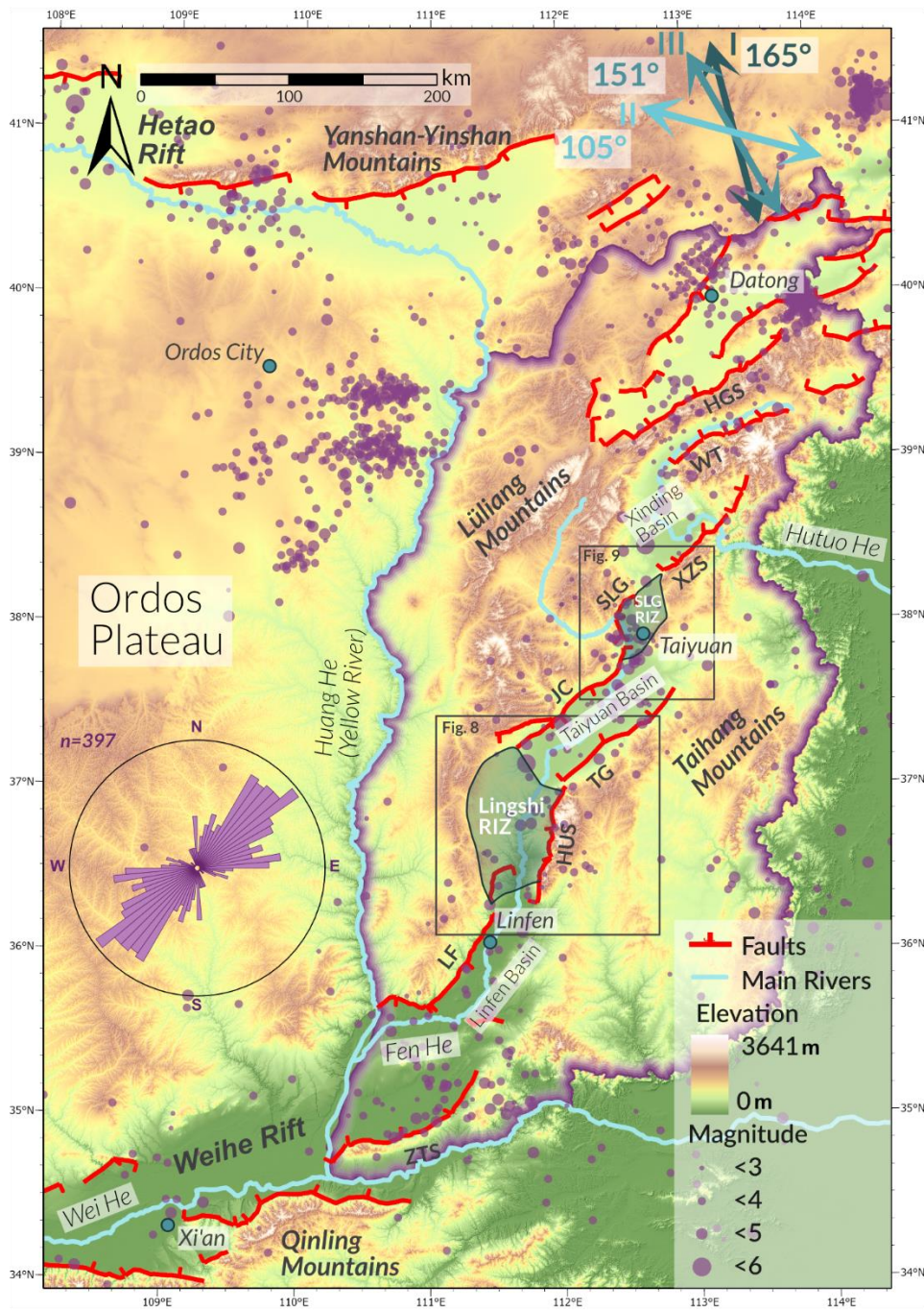
Figure 2: Detailed map of the circum-Ordos Rifts and the main rivers. Extension directions shown are from: I - Zhang et al. (1998) II - Shen et al. (2000) III - Middleton et al. (2017). Rose plot shows the mean orientation of major rift faults in the Shanxi Rift (defined here as the regions that lie within the purple bounding line). Faults were split into individual segments according to their orientation. Purple dots represent earthquakes from the ISC catalogue (Storchak et al., 2013; 2015; Di Giacomo et al., 2018) and are weighted
