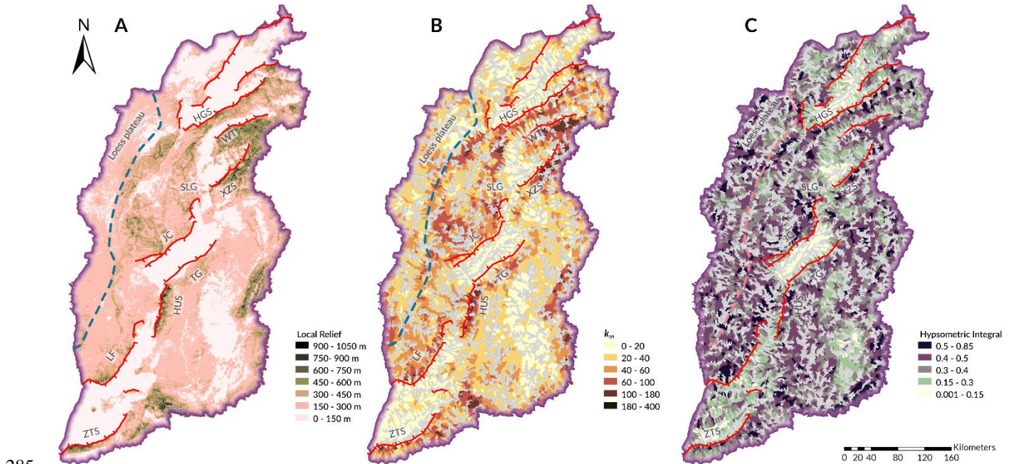
Figure 6: Geomorphic indices map of the Shanxi Rift. Major extensional faults shown in red, boundary of the Loess plateau indicated by dashed line A) Local relief map. Darker colours indicate higher relief regions. Local relief was calculated within a 1km circular radius. High relief is found especially in the northern Shanxi Rift in the footwalls of the Wutai and Xizhoushan faults as well as further south along the Huoshan and Zhongtiaoshan faults. Noticeably lower local relief values occur along the central Jiaocheng and Taigu faults. B) Mean normalised channel steepness ( k_{sn} ) calculated for 1st Strahler order basins. High values are commonly located in the footwalls of active faults, especially the Wutai, Xizhoushan and Huoshan faults. Low values are found in the lower lying basin regions. Central faults (Taigu and Jiaocheng) show noticeably less high k_{sn} basins than other faults. C) Hypsometric Integral (HI) calculated for 1st Strahler order basins. High values are commonly located in the footwalls of active faults, especially the Wutai, Linfen, Shilingguan and Huoshan faults. Low values are found in the lower lying basin regions.
